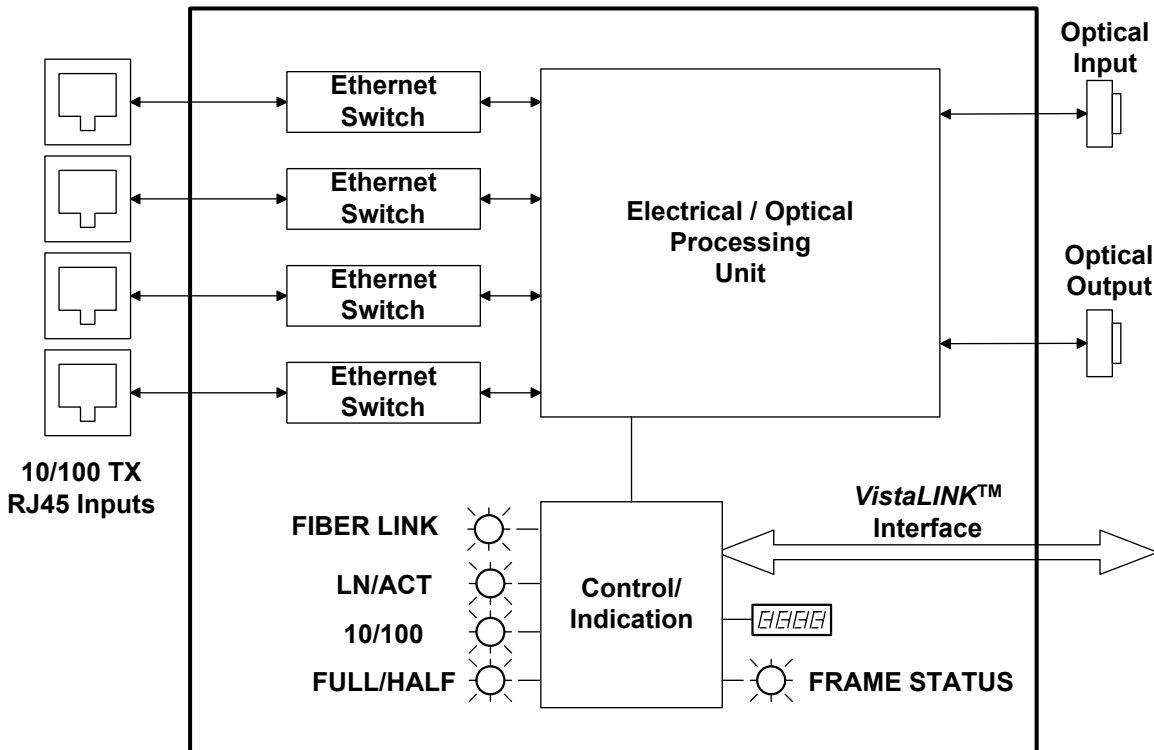
Figure 6: 7707ET-4-F2 Block Diagram
