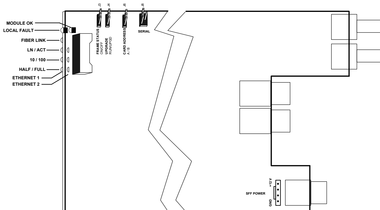
Figure 9: LED and Jumper Locations (ET versions)
