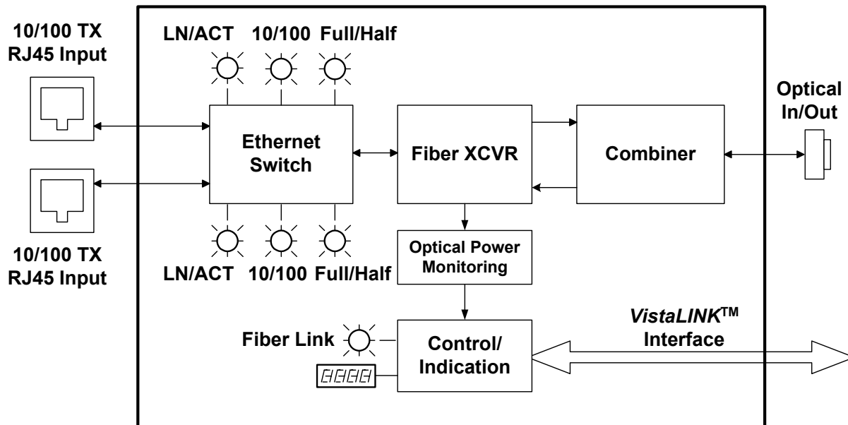
Figure 1: 7707ET Block Diagram
