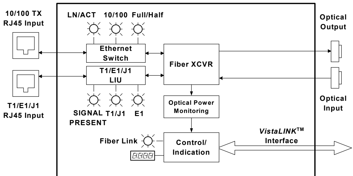
Figure 4: 7707ET-TE1-F2 Block Diagram
