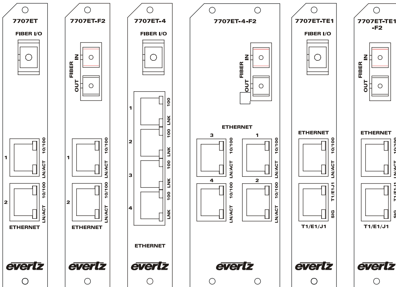
Figure 7: 7707ET Rear panels
