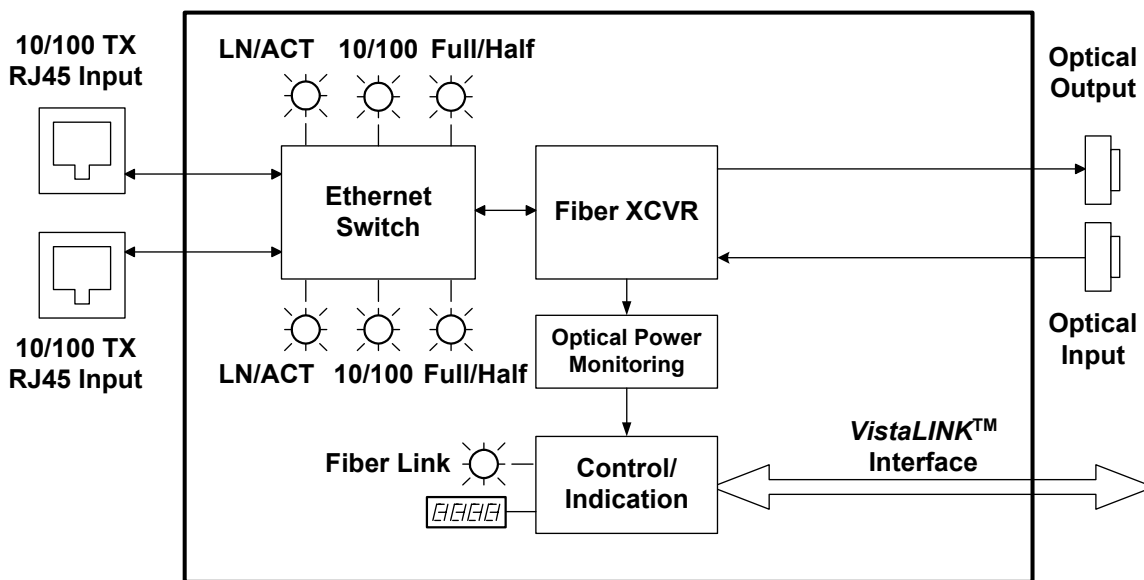
Figure 2: 7707ET-F2 Block Diagram
