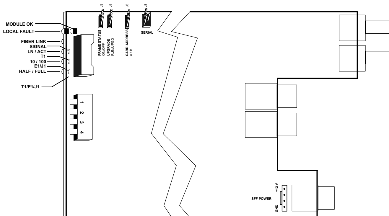
Figure 11: LED and Jumper Locations (TE1 versions)
