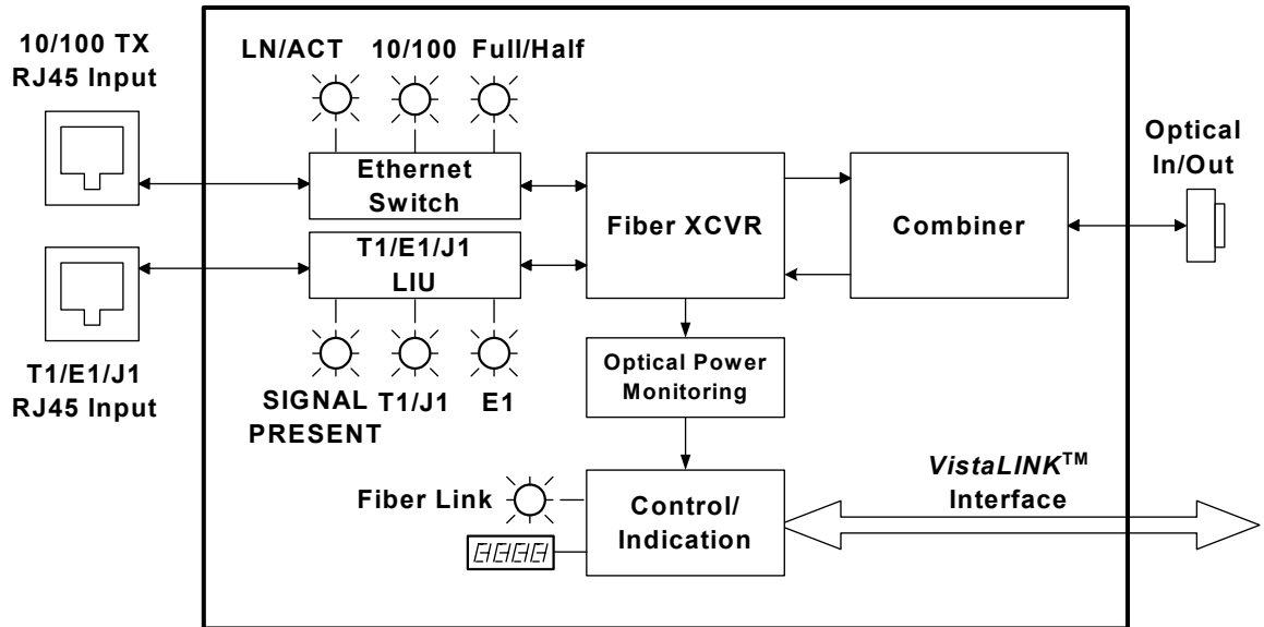
Figure 3: 7707ET-TE1 Block Diagram
