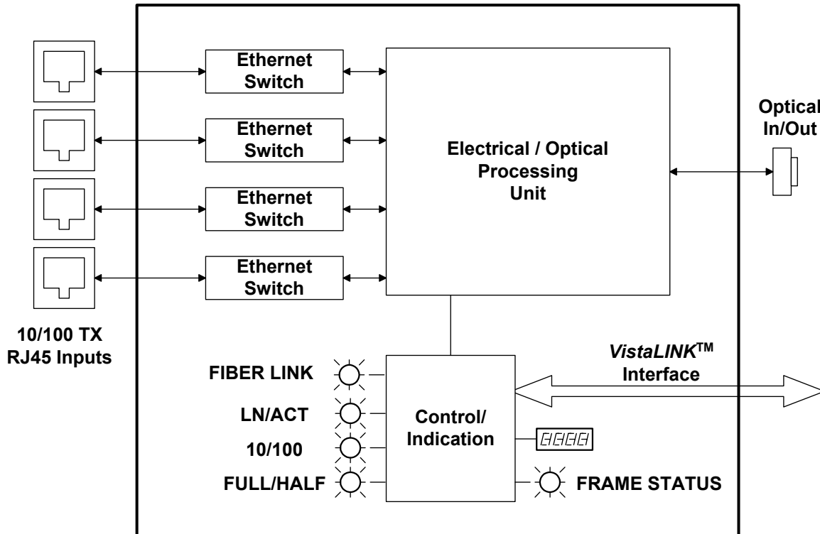
Figure 5: 7707ET-4 Block Diagram
