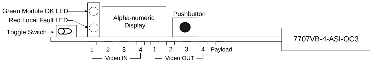
Figure 4-1: Location of Status Indicators and Controls
