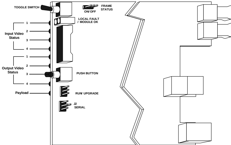
Figure 5-1: Location of Status Indicators and Jumpers
