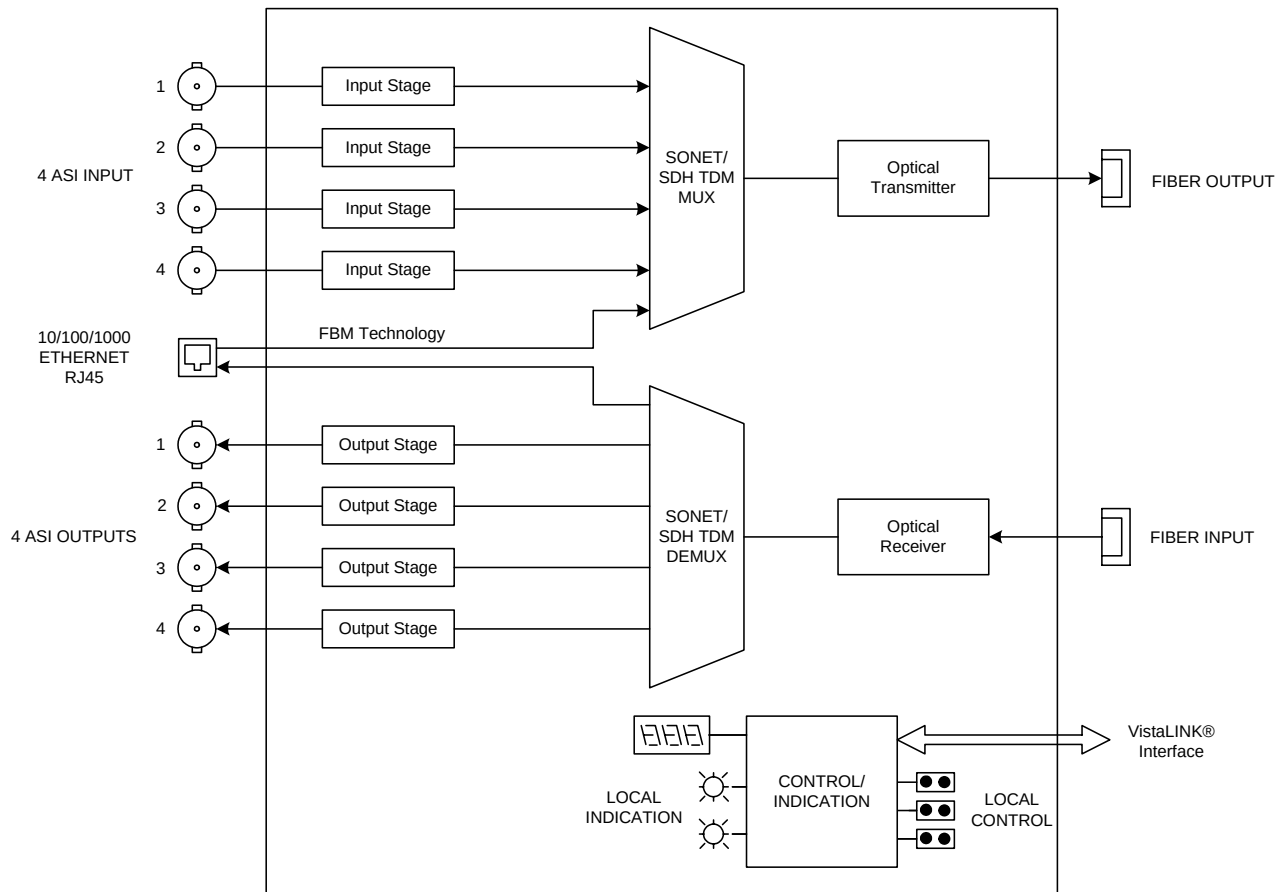
Figure 1-1: 7707VB-4-ASI-OC3 Block Diagram
