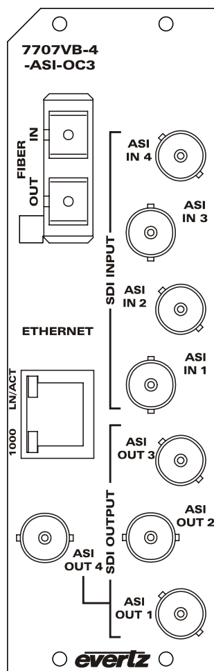
Figure 2-1: 7707VB-4-ASI-OC3 Rear Panel
