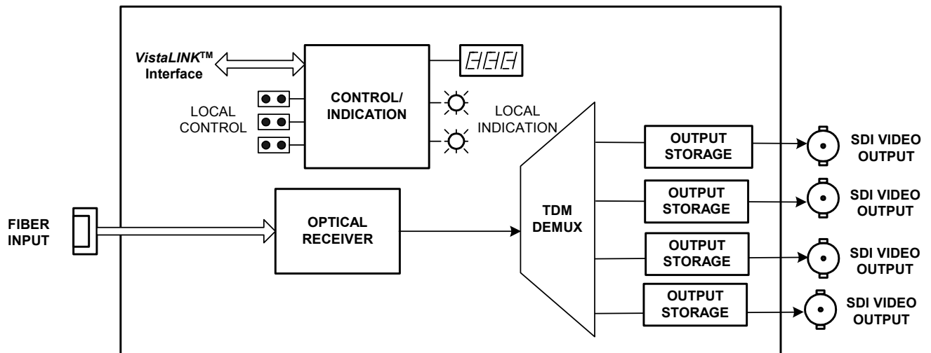
Figure 1: 7707VR-4 Block Diagram
