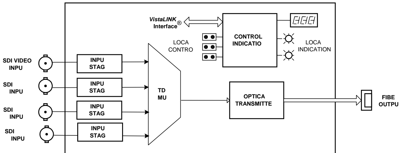
Figure 1-1: 7707VT-4 Block Diagram
