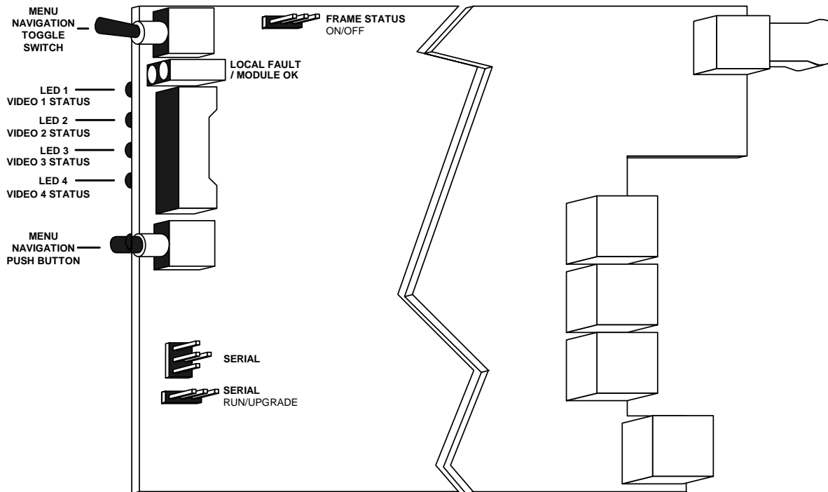
Figure 4-1: Location of Status Indicators, Jumpers and Controls
