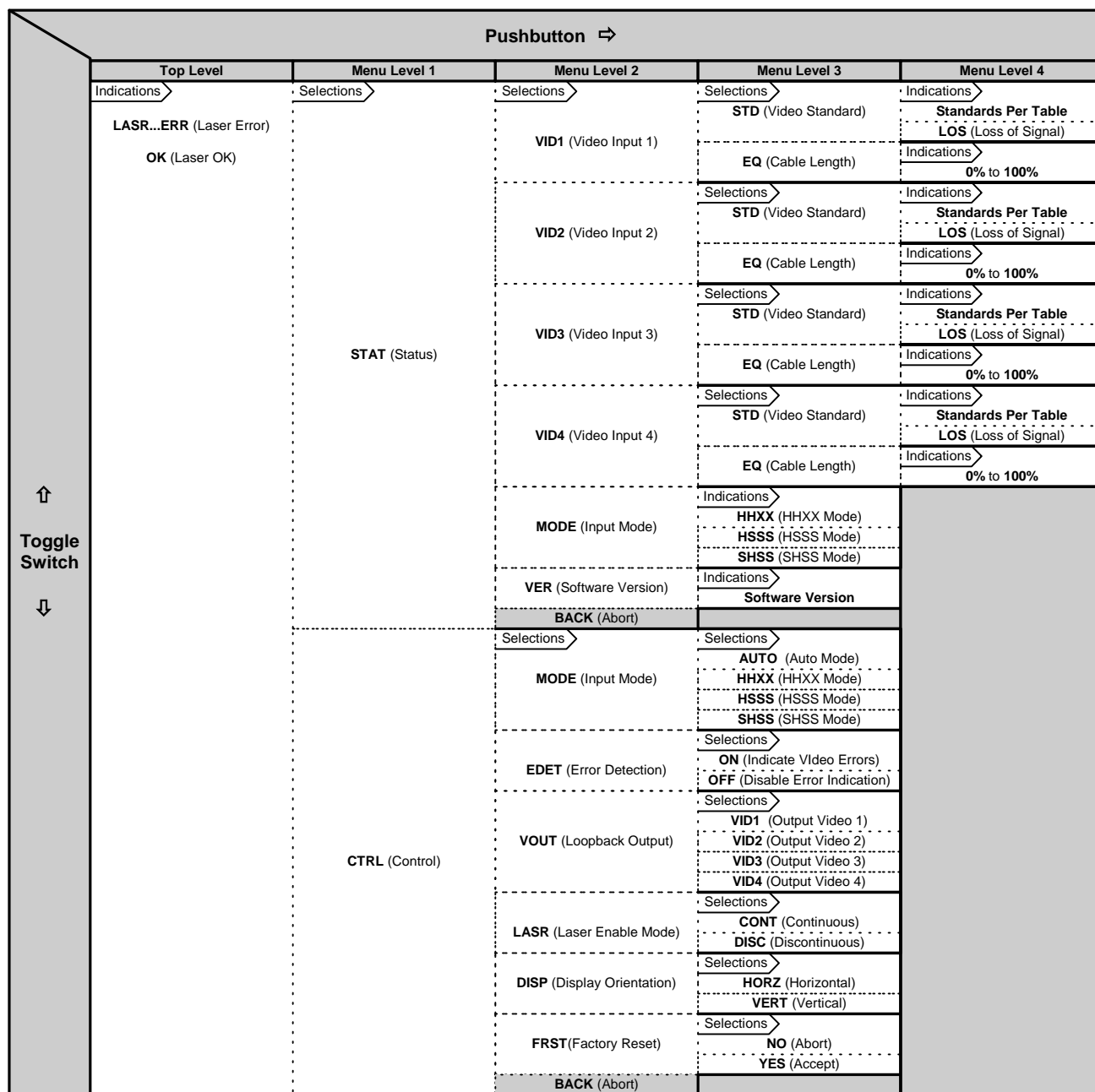
Figure 4-2: Card Edge Menu Structure
