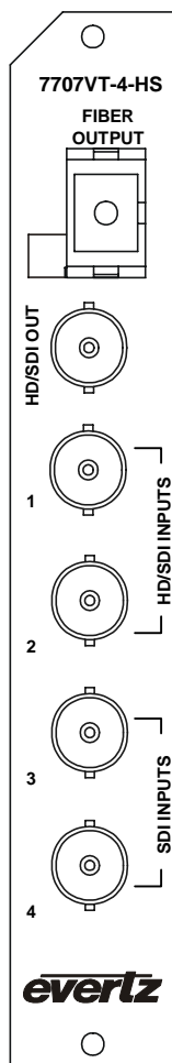
Figure 2-1: 7707VT-4-HS Rear Panel
