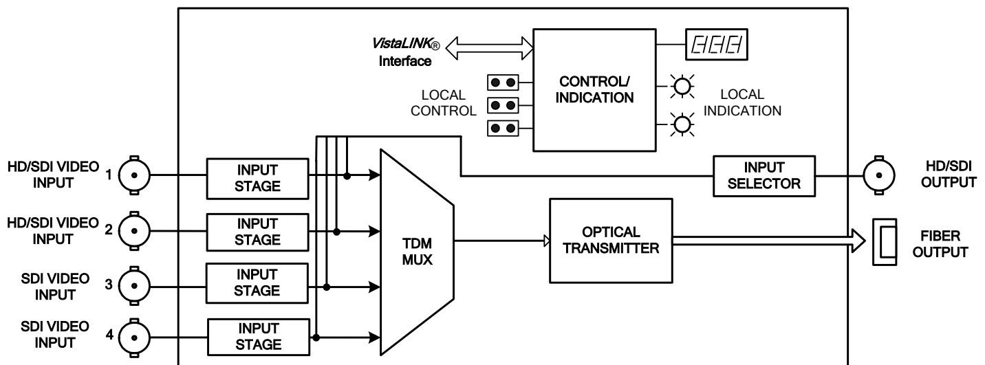
Figure 1-1: 7707VT-4-HS Block Diagram
