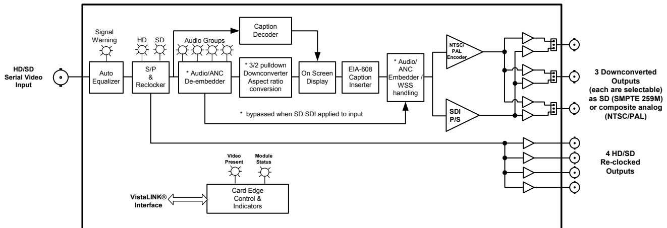
Figure 1: 7710DCDA-HD Block Diagram
