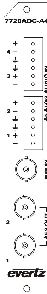
Figure 2: 7720ADC-A4 Rear Panel
