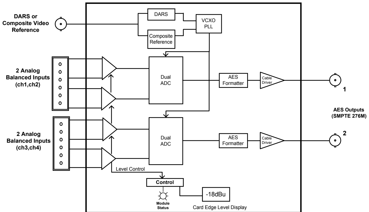
Figure 1: 7720ADC-A4 Block Diagram
