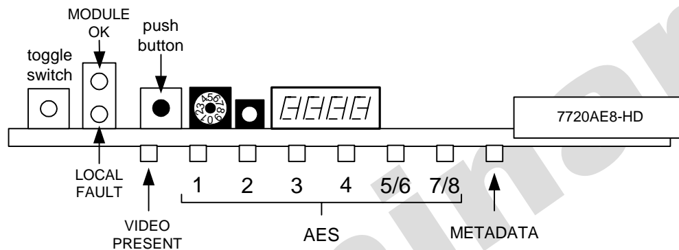
Figure 4: Status LED Locations
