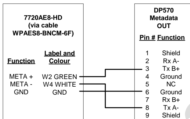
Figure 3: Connecting to a Dolby DP570
