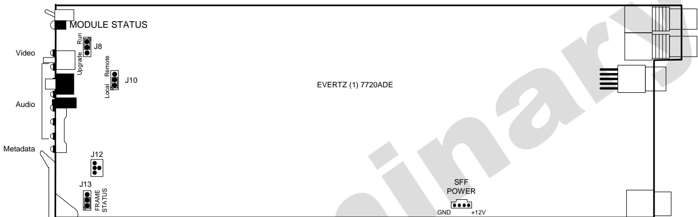
Figure 6: Location of Jumpers
