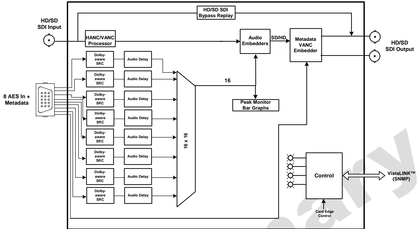
Figure 1: 7720AE8-HD Block Diagram
