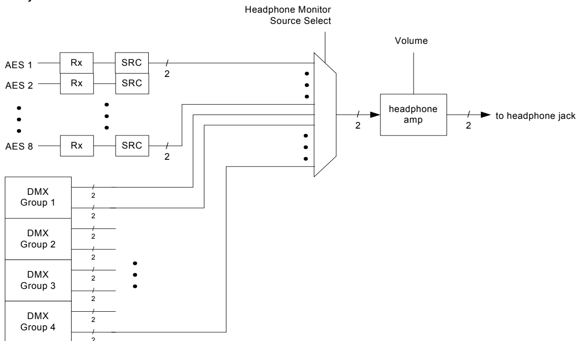
Figure 6-5: Headphone Monitoring
