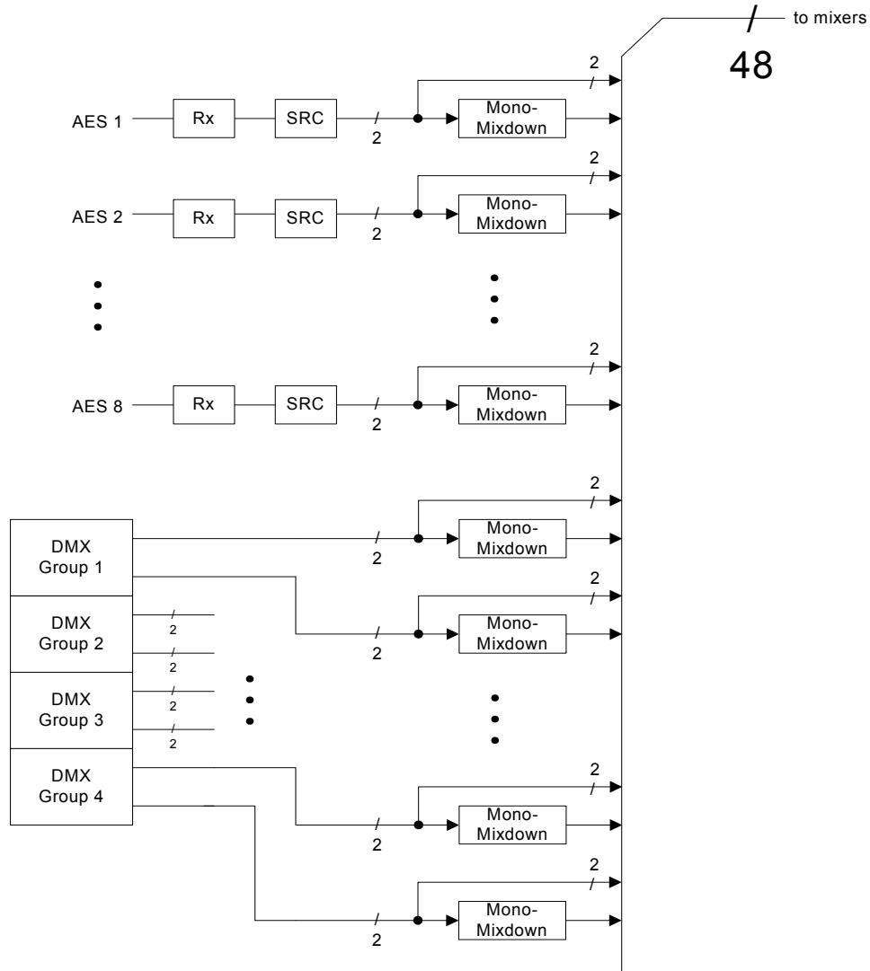
Figure 6-4: Mono-Mixers
