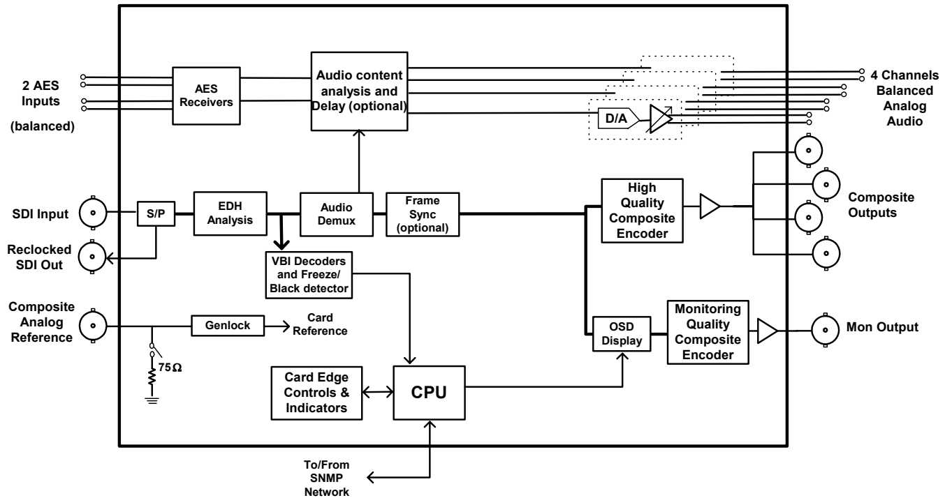
Figure 3: 7736CEM-A4-B Block Diagram
