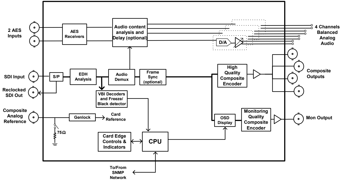
Figure 1: 7736CEM-A4 Block Diagram
