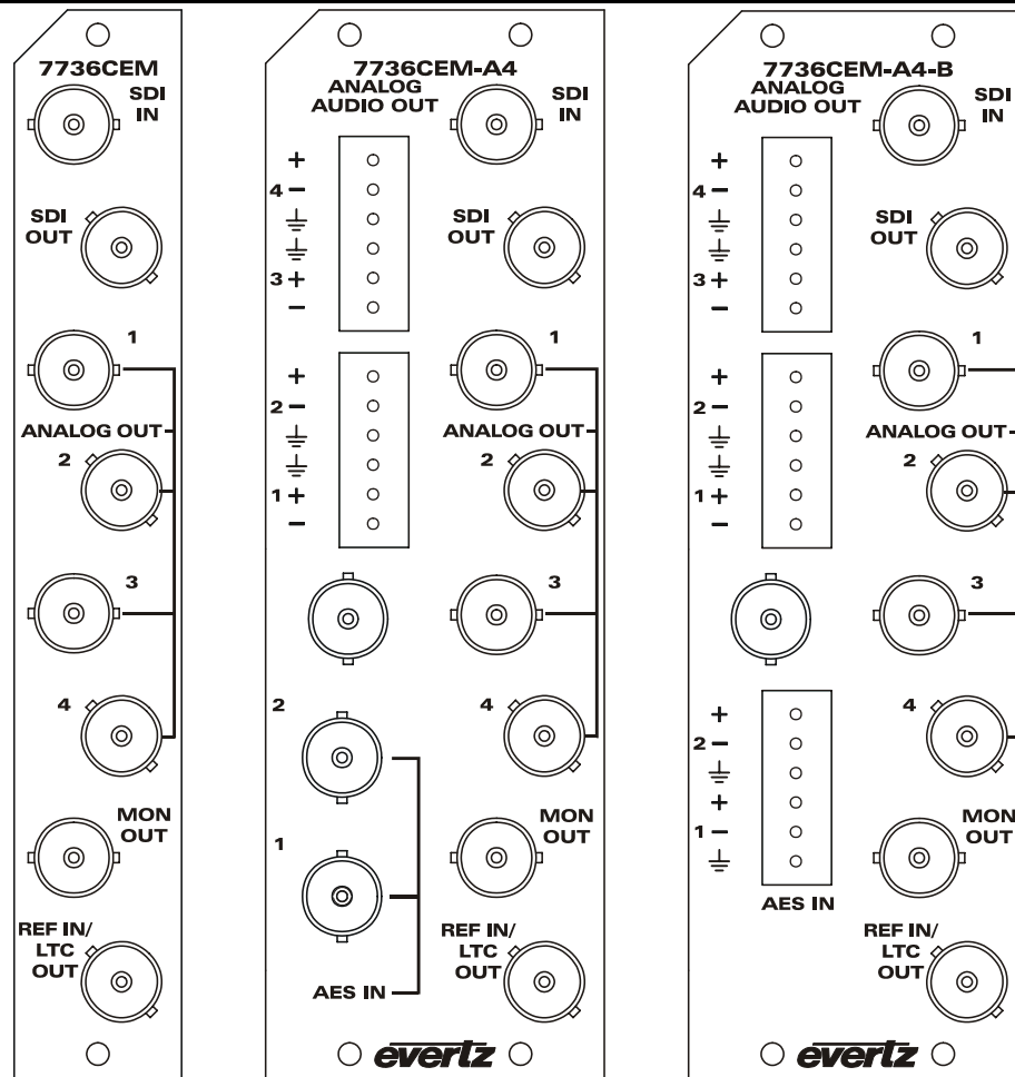
Figure 4: 7736CEM Rear Panels
