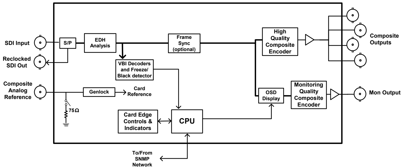
Figure 2: 7736CEM Block Diagram
