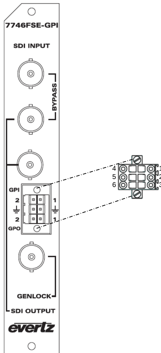
Figure 2-4: GPI and GPO Connections
