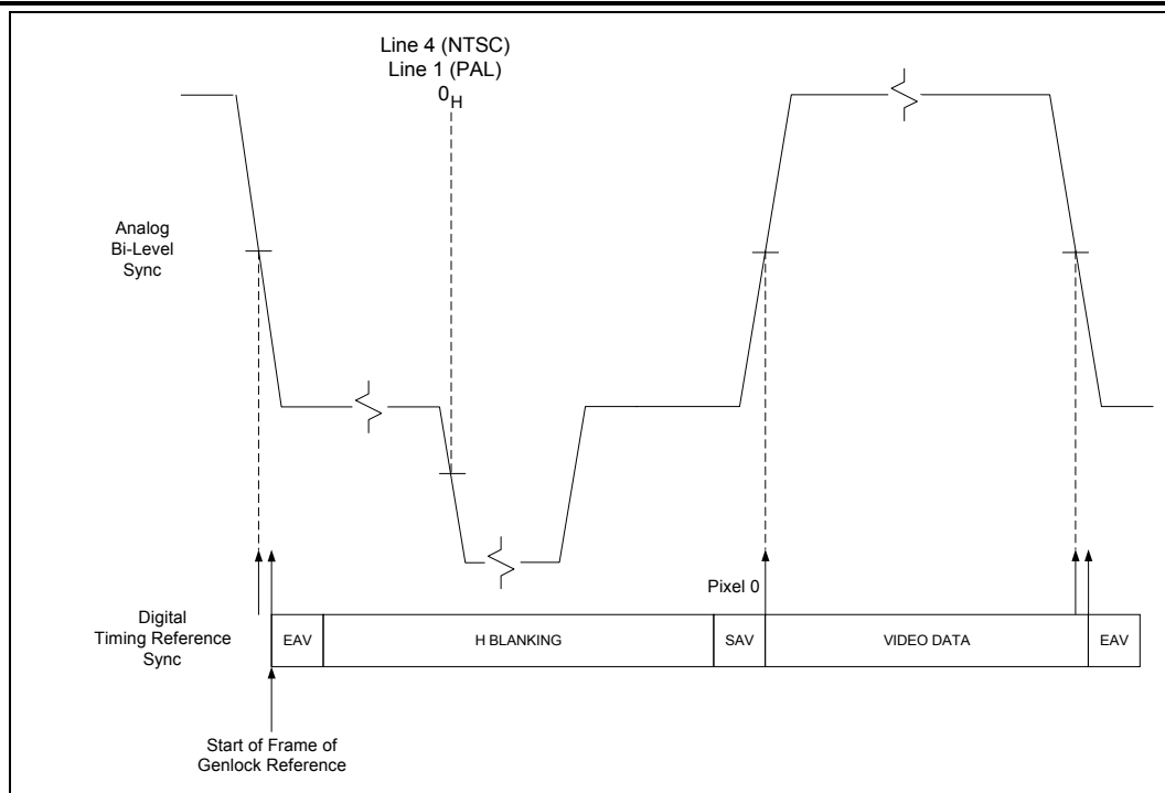
Figure 4: Default Bi-Level Gen Lock Reference Timing
