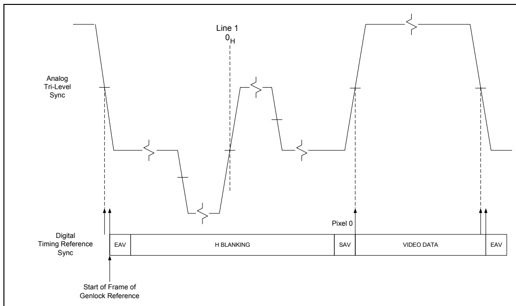
Figure 3: Default Tri-Level Gen Lock Reference Timing
