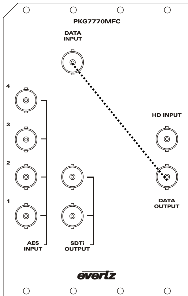
Figure 2: PKG7770MFC-HD Rear Panel
