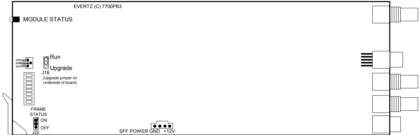
Figure 4: Location of Jumpers Bottom Board (PKG7770MFC)
