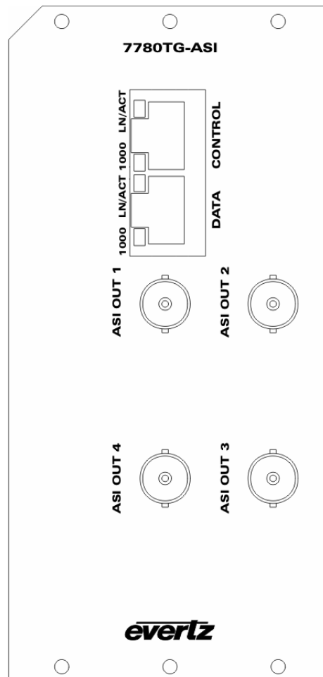
Figure 2-1: 7780TG-ASI Rear Panel
