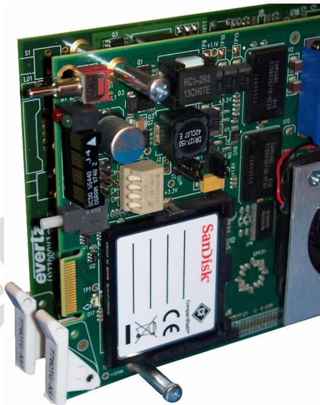
Figure 2-3: Compact Flash Card Installed
