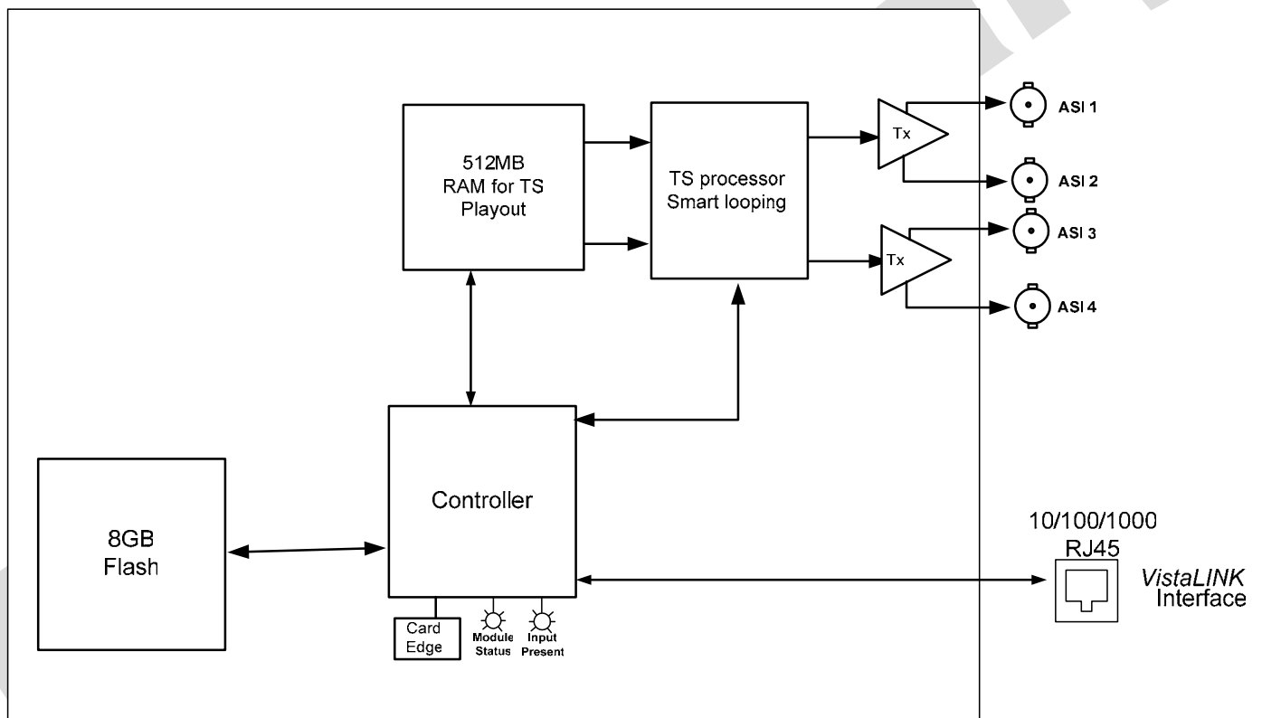
Figure 1-1: 7780TG-ASI Block Diagram
