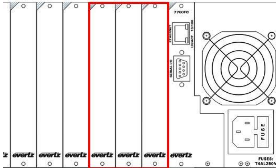
Figure 2-2: 7700 Chassis
