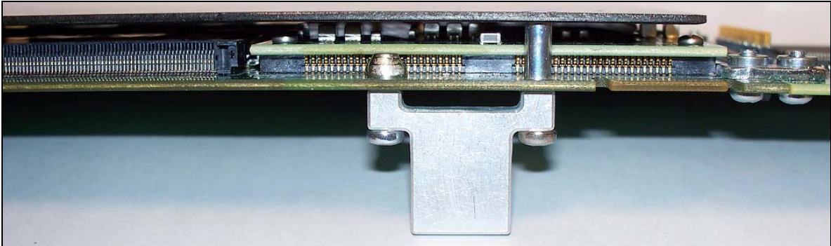
Figure 8-1: Slot Blocker
