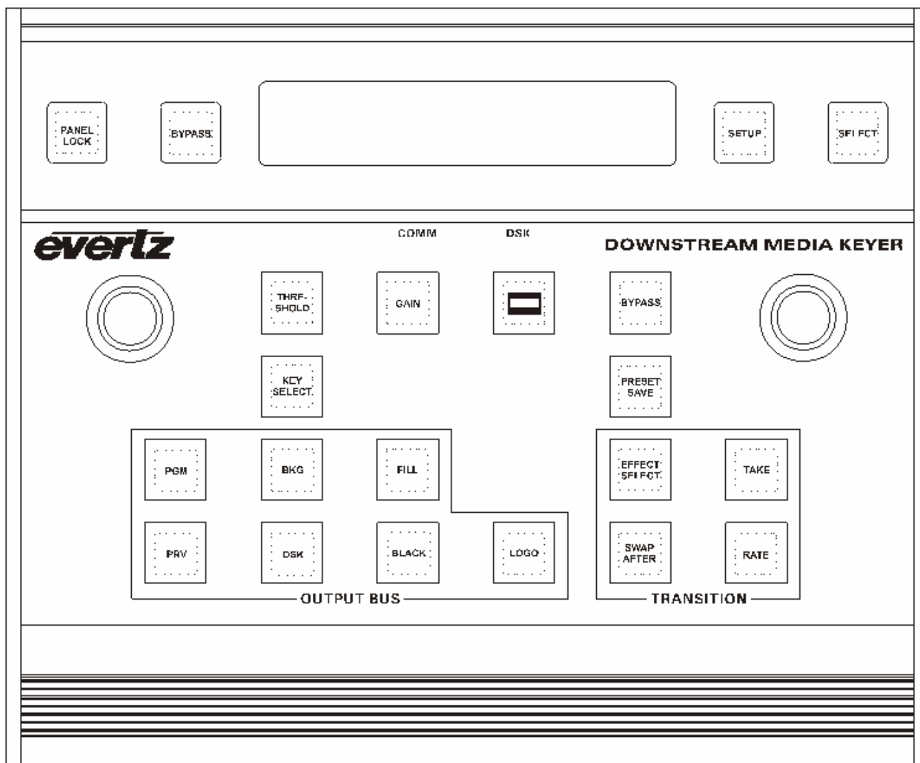
Figure 7-1: 7825DSK2-LG-HD – Desktop Control Panel Layout
