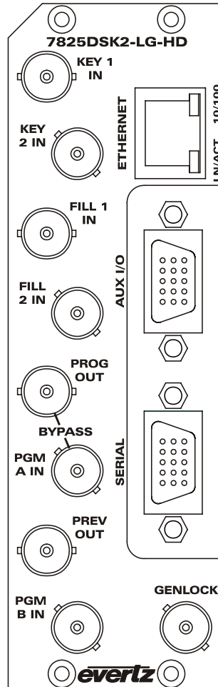
Figure 2-1: 7825DSK2-LG-HD Rear Panel
