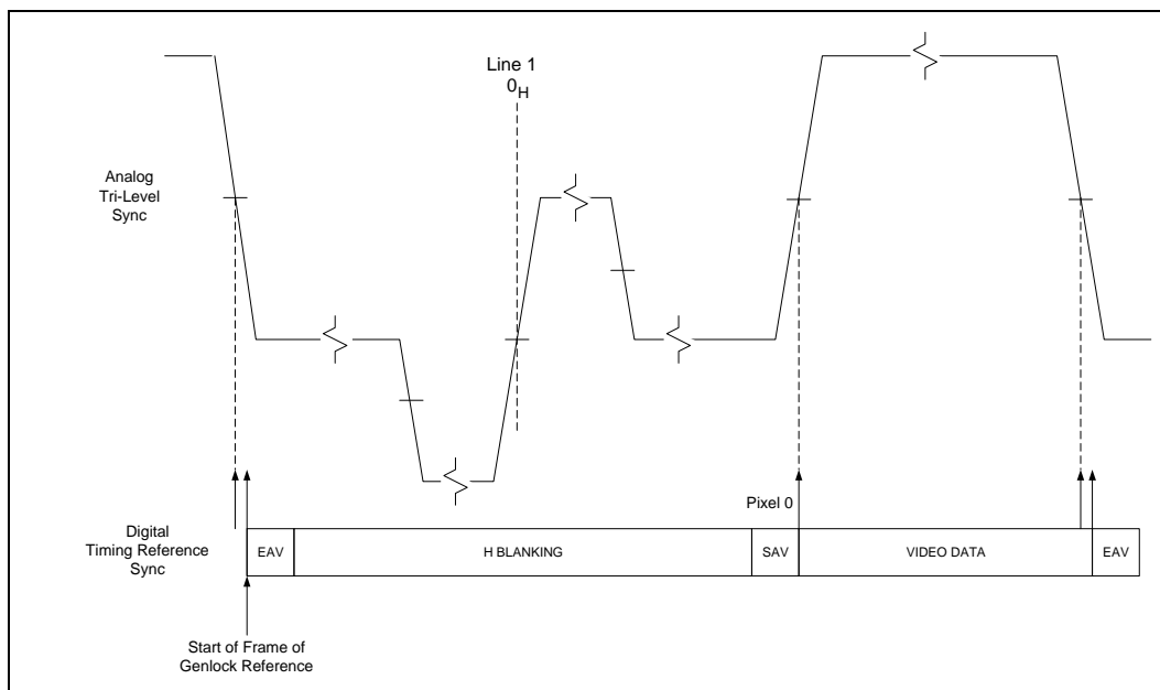
Figure 4-1: Default Tri-Level Genlock Reference Timing
