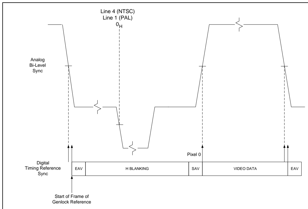
Figure 4-2: Default Bi-Level Genlock Reference Timing
