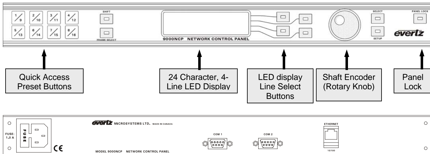
Figure 4-1: 9000NCP Front and Rear Views
