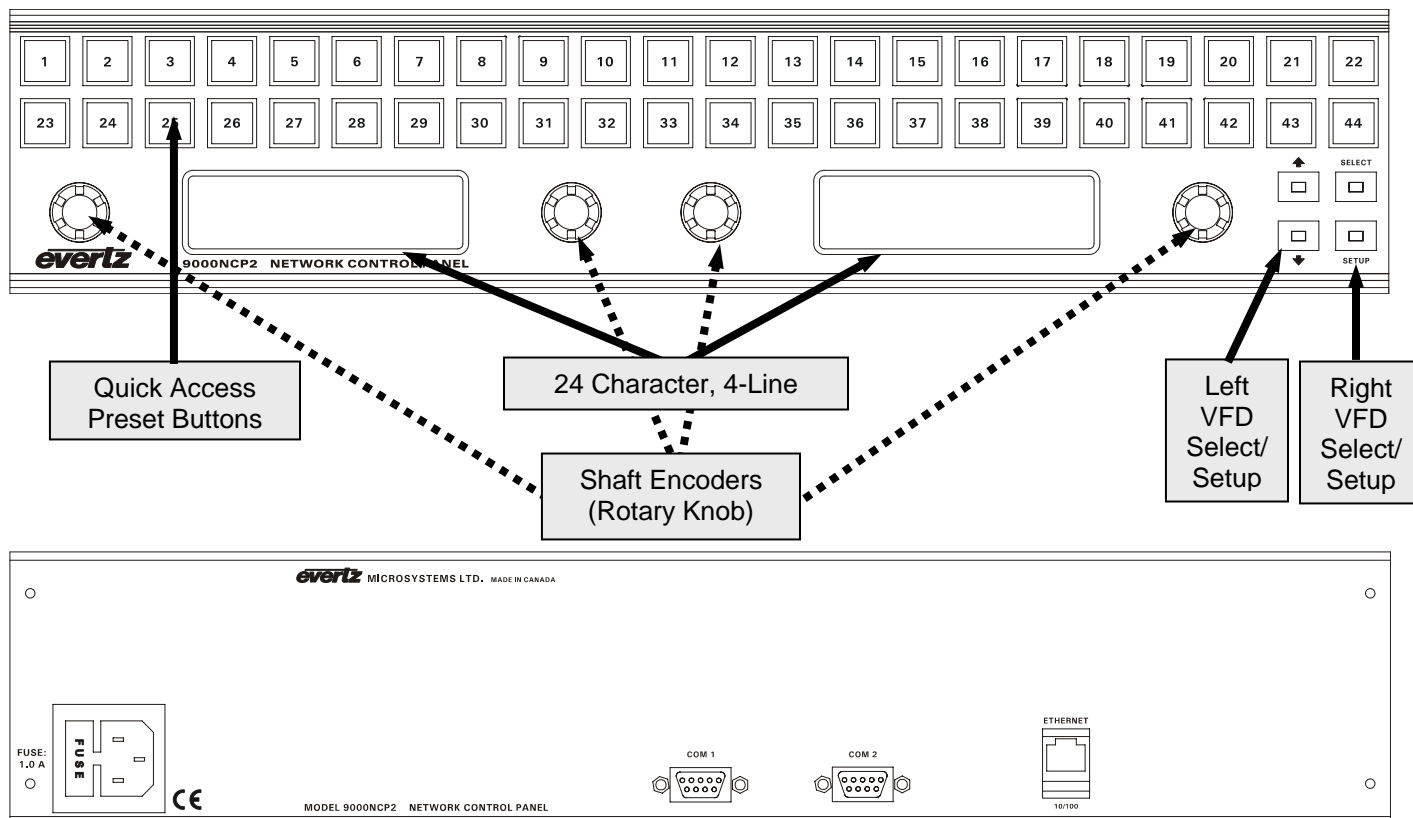
Figure 5-1: 9000NCP2 Front and Rear Views
