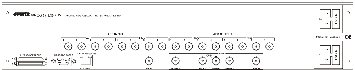
Figure 2-5: HD9725LGA Rear Panel
