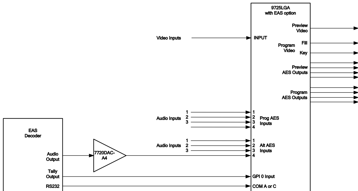
Figure 6-1: EAS Decoder Connection
