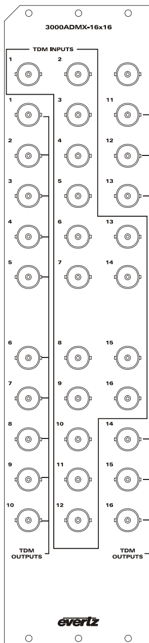
Figure 2-15: 3000ADMX-16x16 Rear Plate
