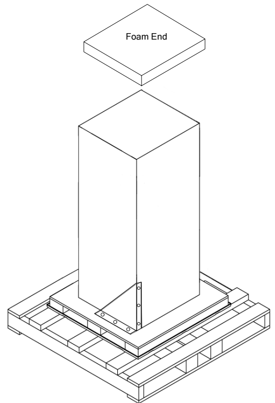
Figure 1-2: EQX with Shipping Panels Removed
