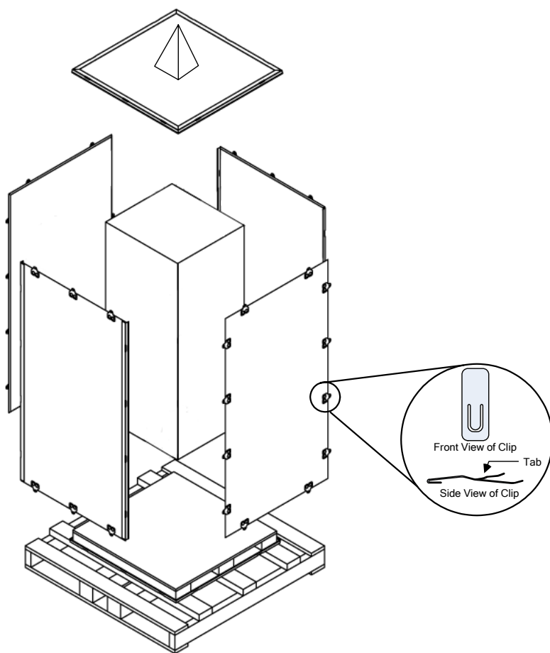
Figure 1-1: EQX Shipping Container
