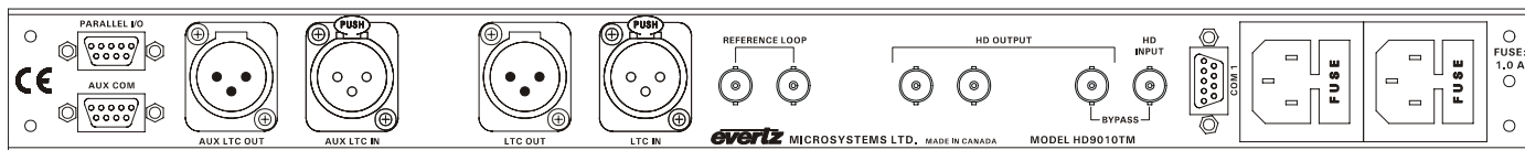
Figure 2-1: HD9010TM-IRIG Rear Panel
