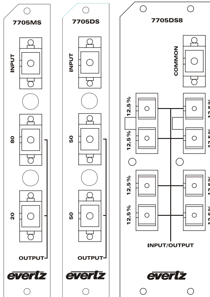
Figure 9: 7705MS and 7705DS Rear Panels
