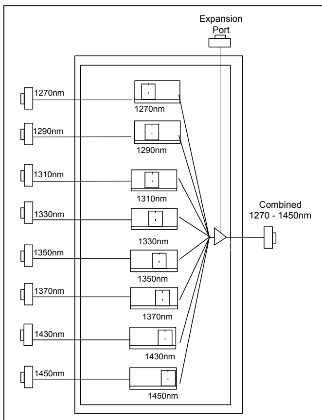
Figure 7: 7705CWDM-8LB Block Diagram
