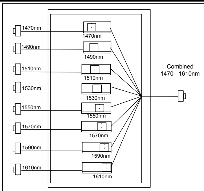
Figure 6: 7705CWDM-8 Block Diagram
