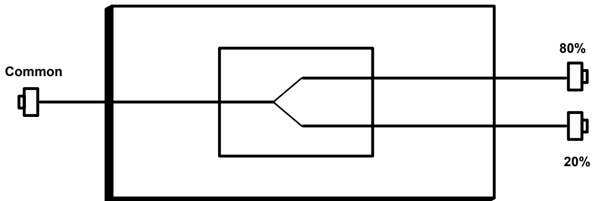
Figure 3: 7705MS Block Diagram
