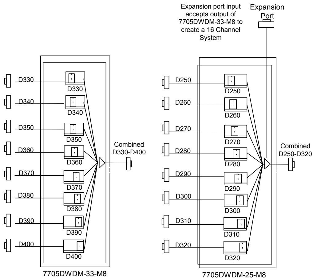
Figure 8: 7705DWDM Block Diagrams
