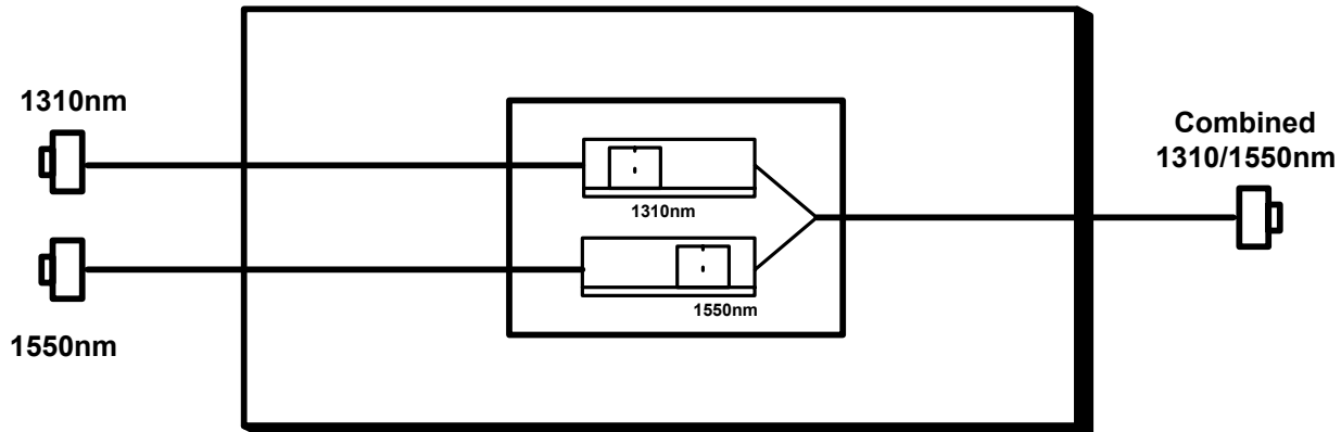
Figure 1: 7705WDM13/15 and 7705WDM Block Diagram
