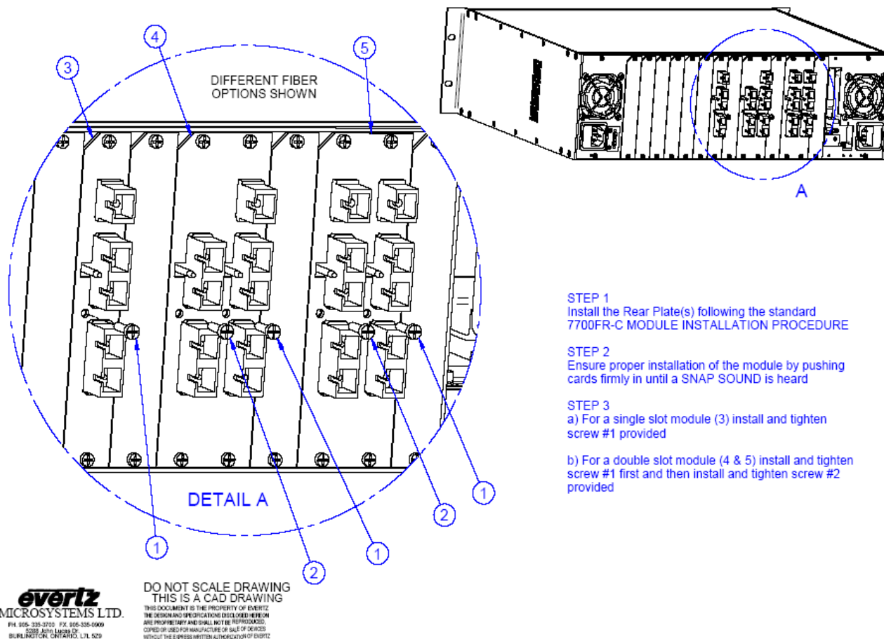
Figure 10: Dual Slot Card Retention Mechanism
