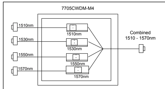
Figure 5: 7705CWDM-4 Block Diagram
