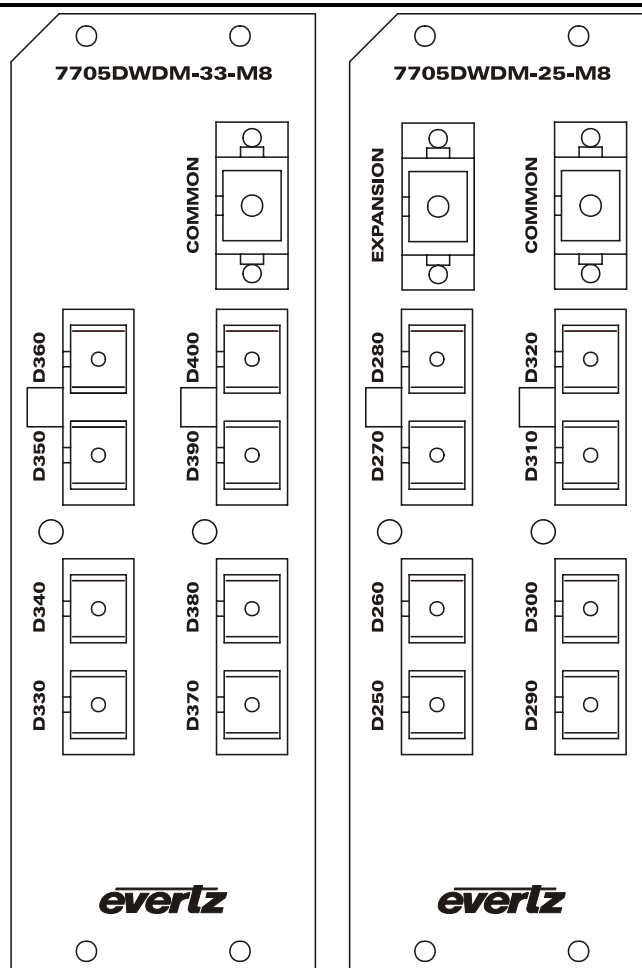
Figure 11: 7705WDM, 7705CWDM and 7707DWDM* Rear Panels
