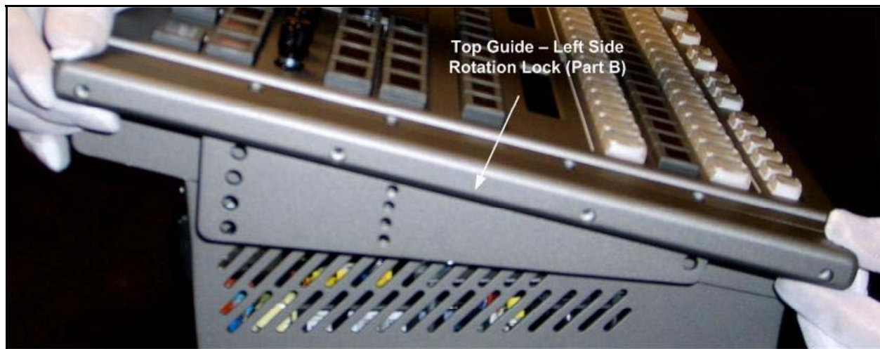
Figure 3-3: Attaching the Top Guide Rotation Lock – Left Side
