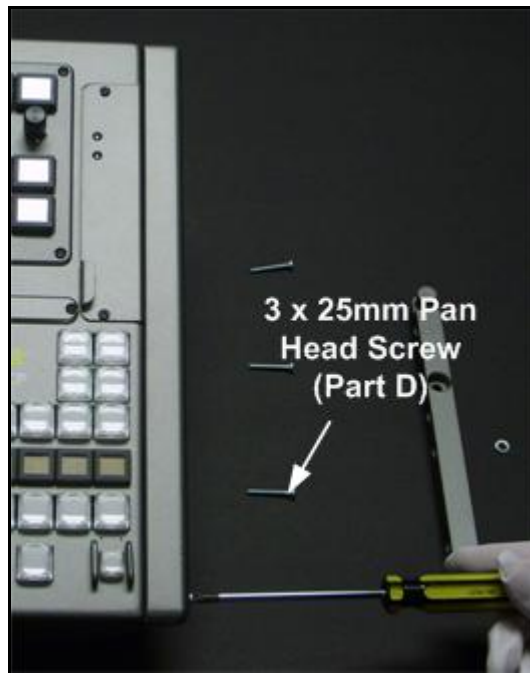
Figure 3-2: Securing the Top Guide Rotation Lock – Right Side
