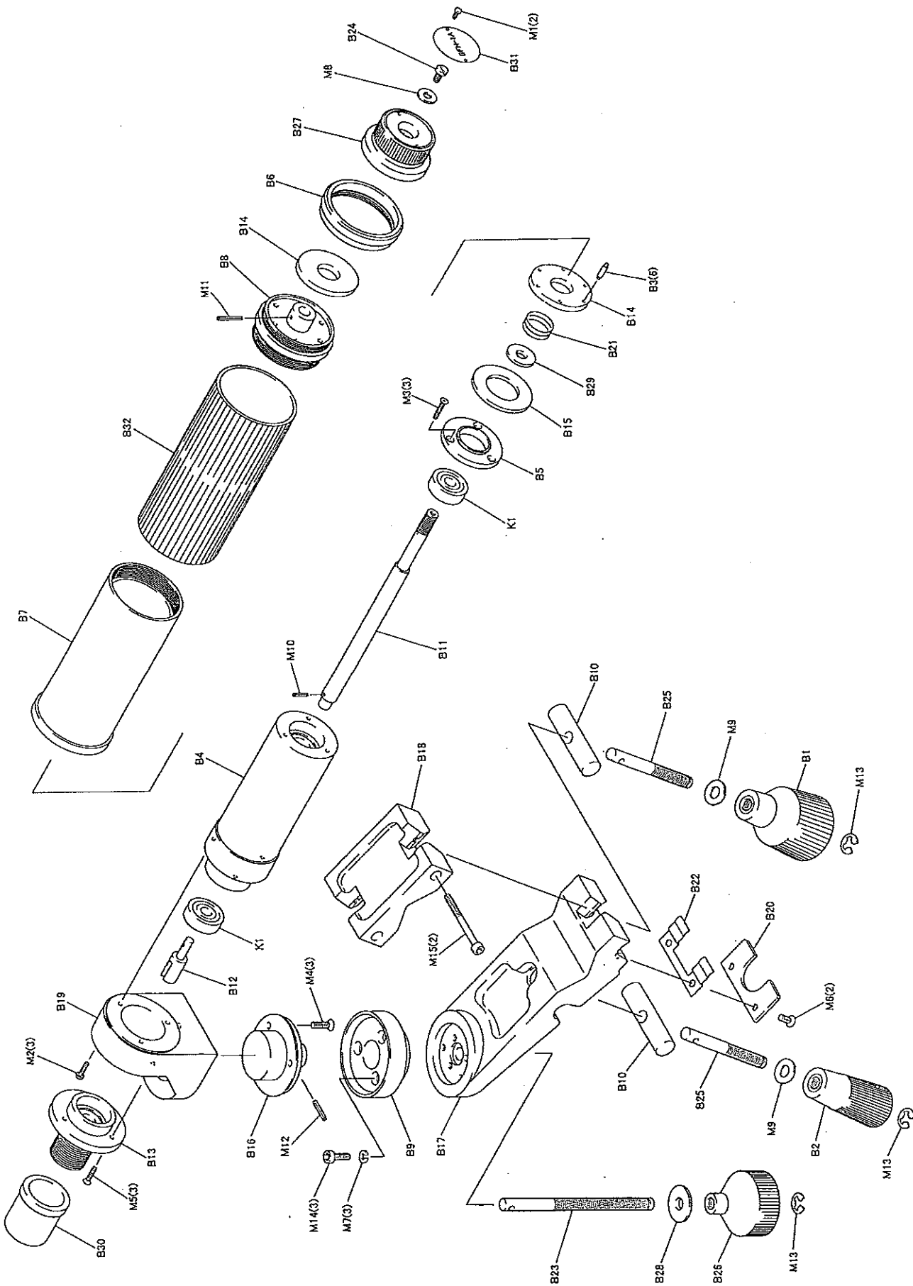
Fig. 1 Focus grip BFH-1A
