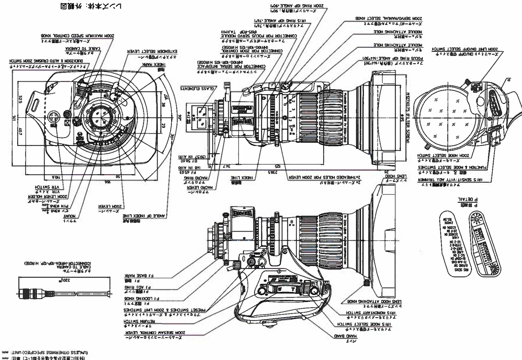
③ 天本体：外觀圖 Outline drawing HA13×4.5BERM-M58B
