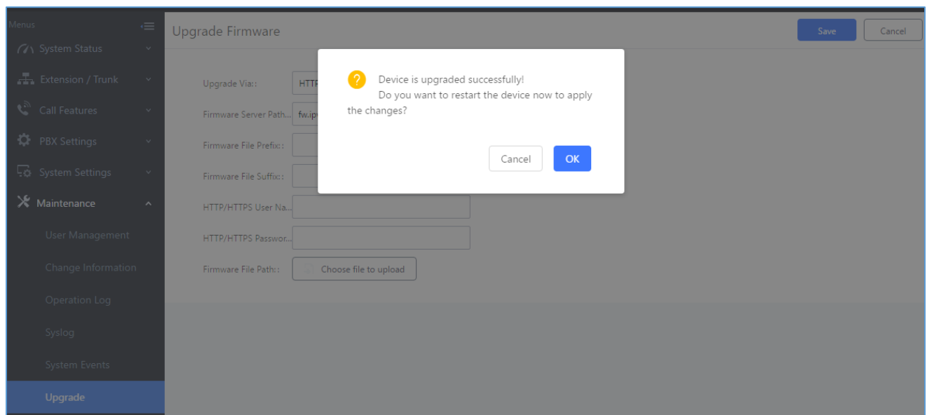
Figure 334: Reboot UCM6200
