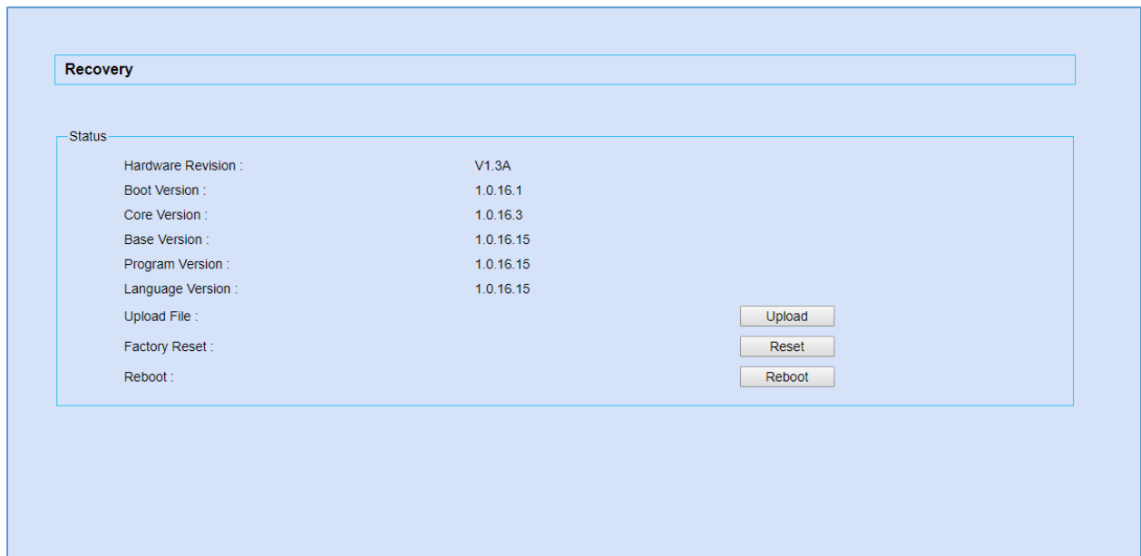
Figure 344: Recovery Mode
