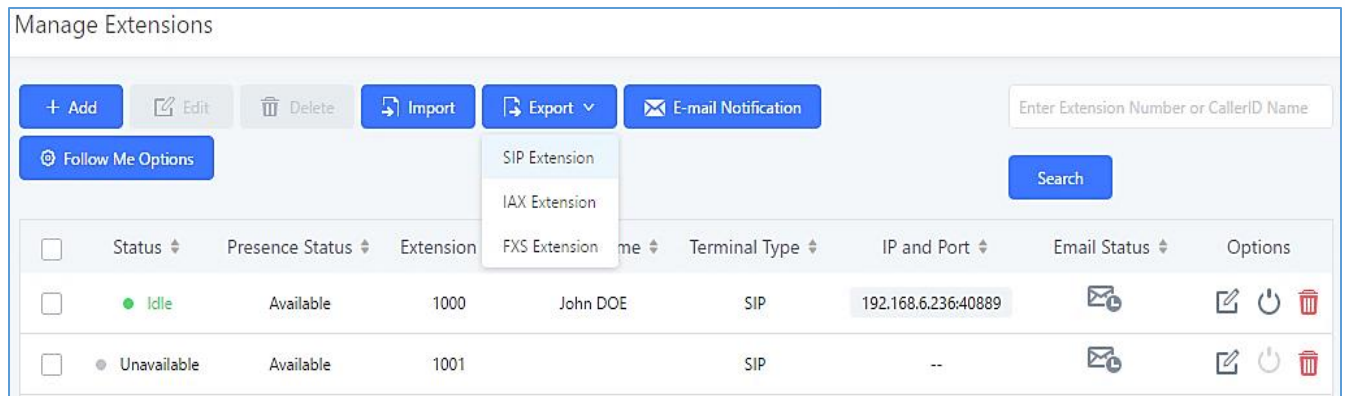
Figure 85: Export Extensions
