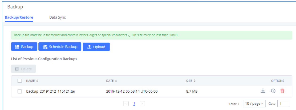
Figure 336: Backup / Restore
