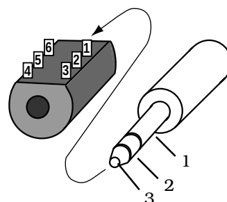
JACK socket Corresponding plug: -Type: JACKFLJCN -Ref.: T1004861
