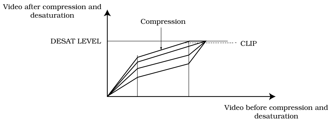
RESPONSE TO THE COMPRESSION AND DESATURATION STAGES
