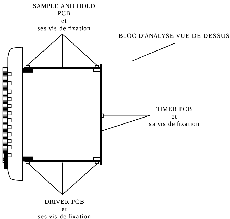
DÉPOSE DES CARTES "TIMER", "DRIVER", "SAMPLE AND HOLD"
