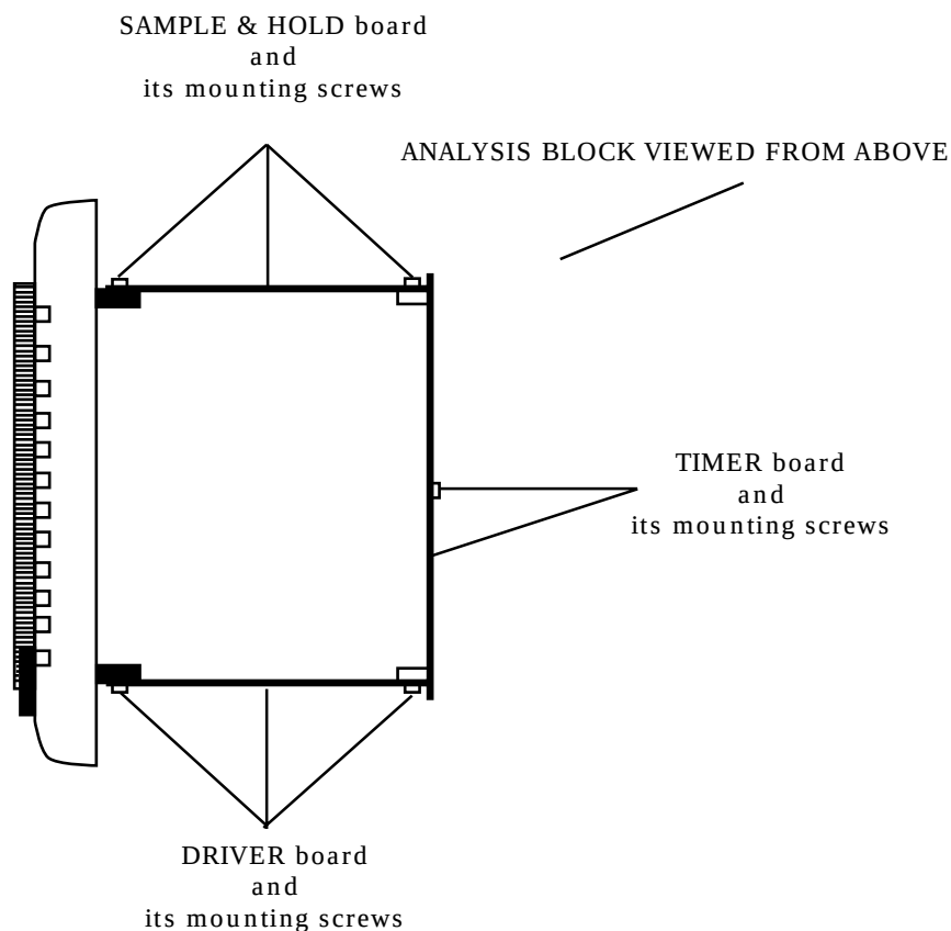
REMOVING THE DRIVER, TIMER AND SAMPLE & HOLD BOARDS
