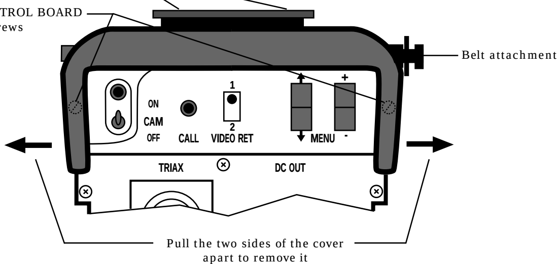
REMOVING THE REAR CONTROL BOARD
