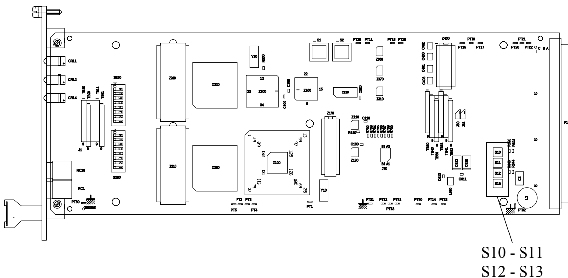
Carte"APCM" version 1
