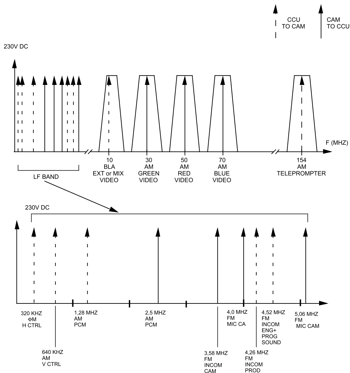
Distribution of frequency spectrums along cable
