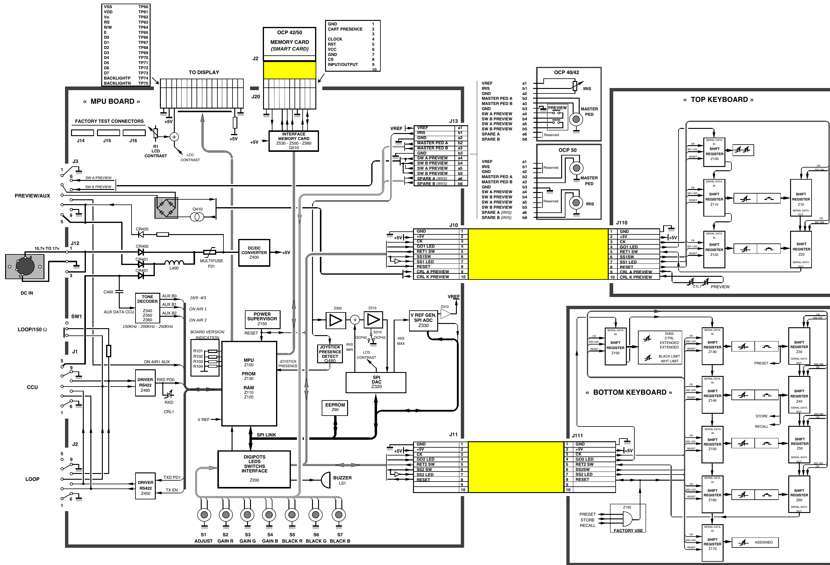
OCP 42/OCP 50 BLOCK-DIAGRAM
