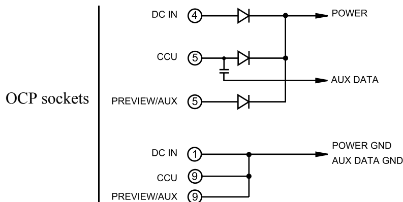
Figure 1 : Connection of the OCP power supplies
