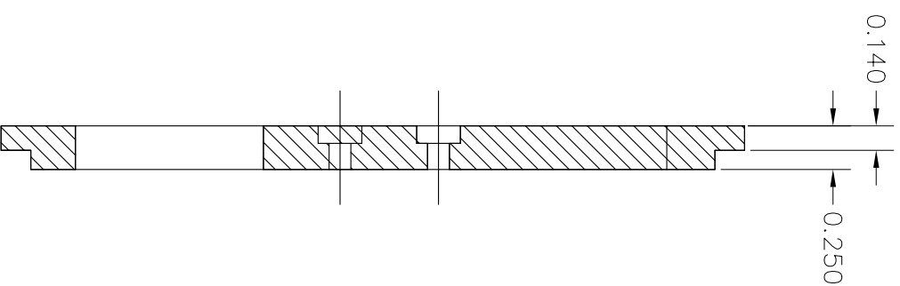
SECTION VIEW
