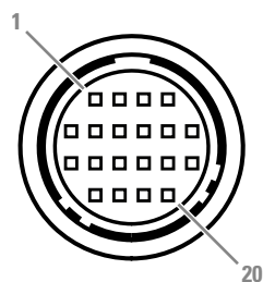
20-pin Hirose female connector (panel view)
