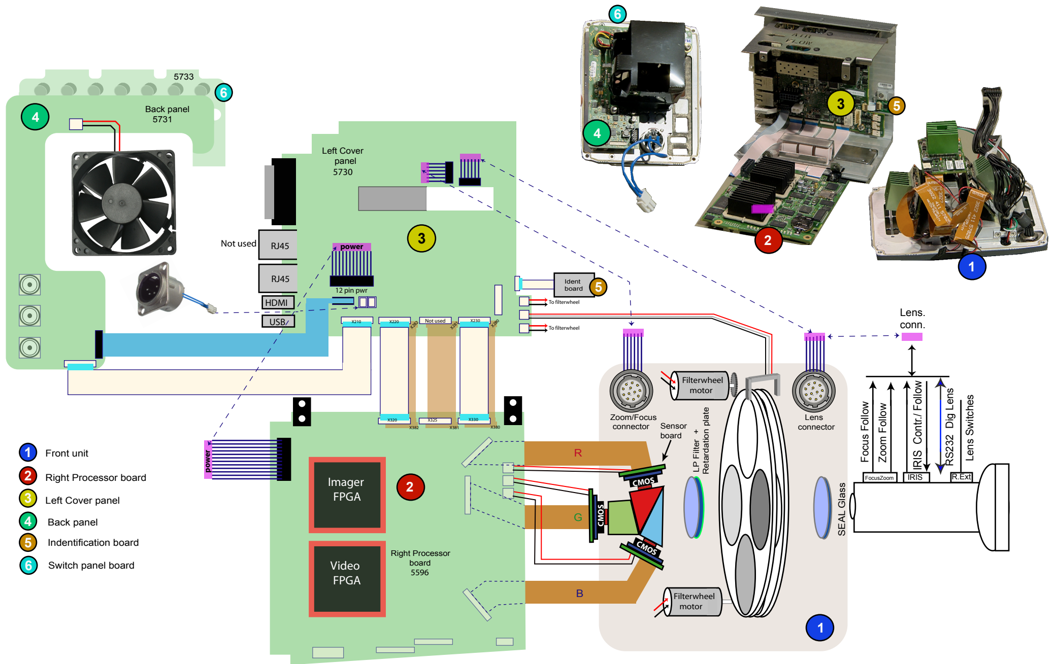
LDX Compact Main Diagram
