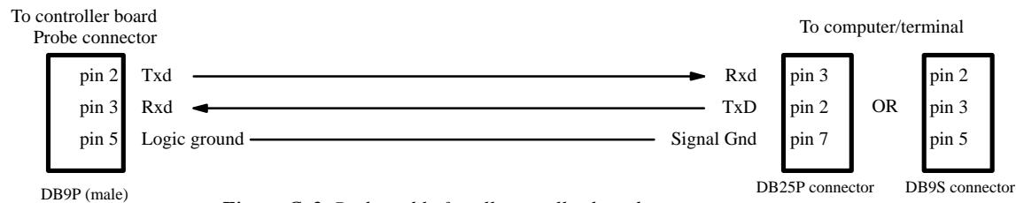
Figure C-2. Probe cable for all controller boards.
