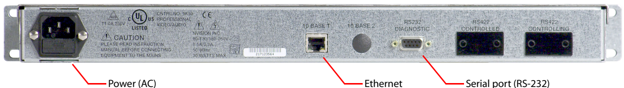
Figure 2-2. NV9604 Rear
