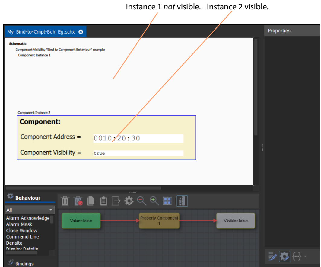
Fig. 4-51: Exercising Screen.
