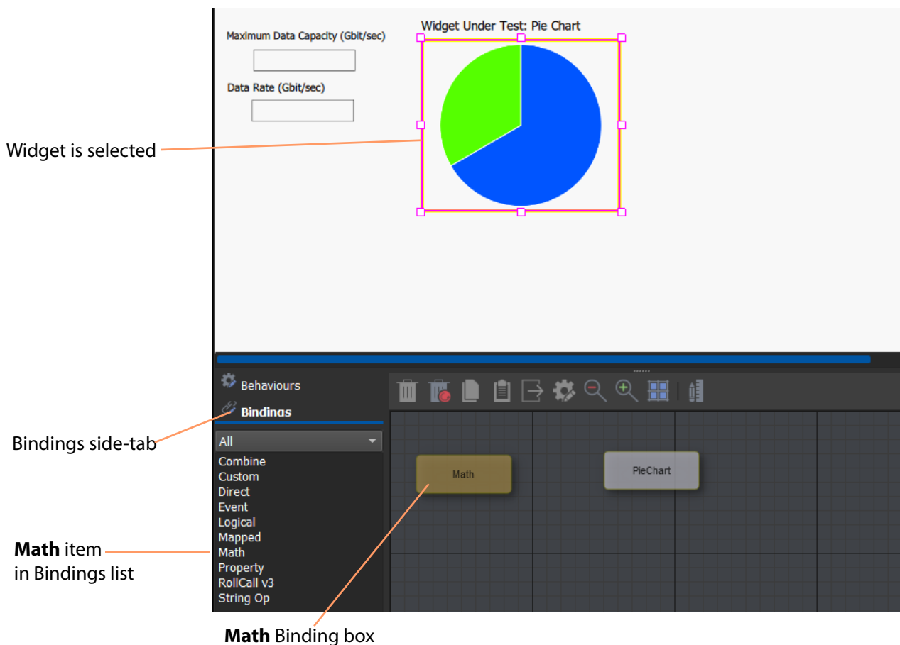
Fig. 3-9: Math Binding
