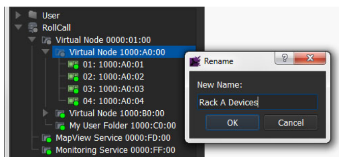
Fig. 8-34: Rename Dialog
