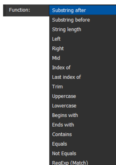
Fig. 5-8: String Functions
