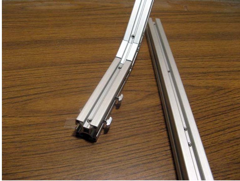
Figure 40. Middle Straight Support Bolt Orientation
