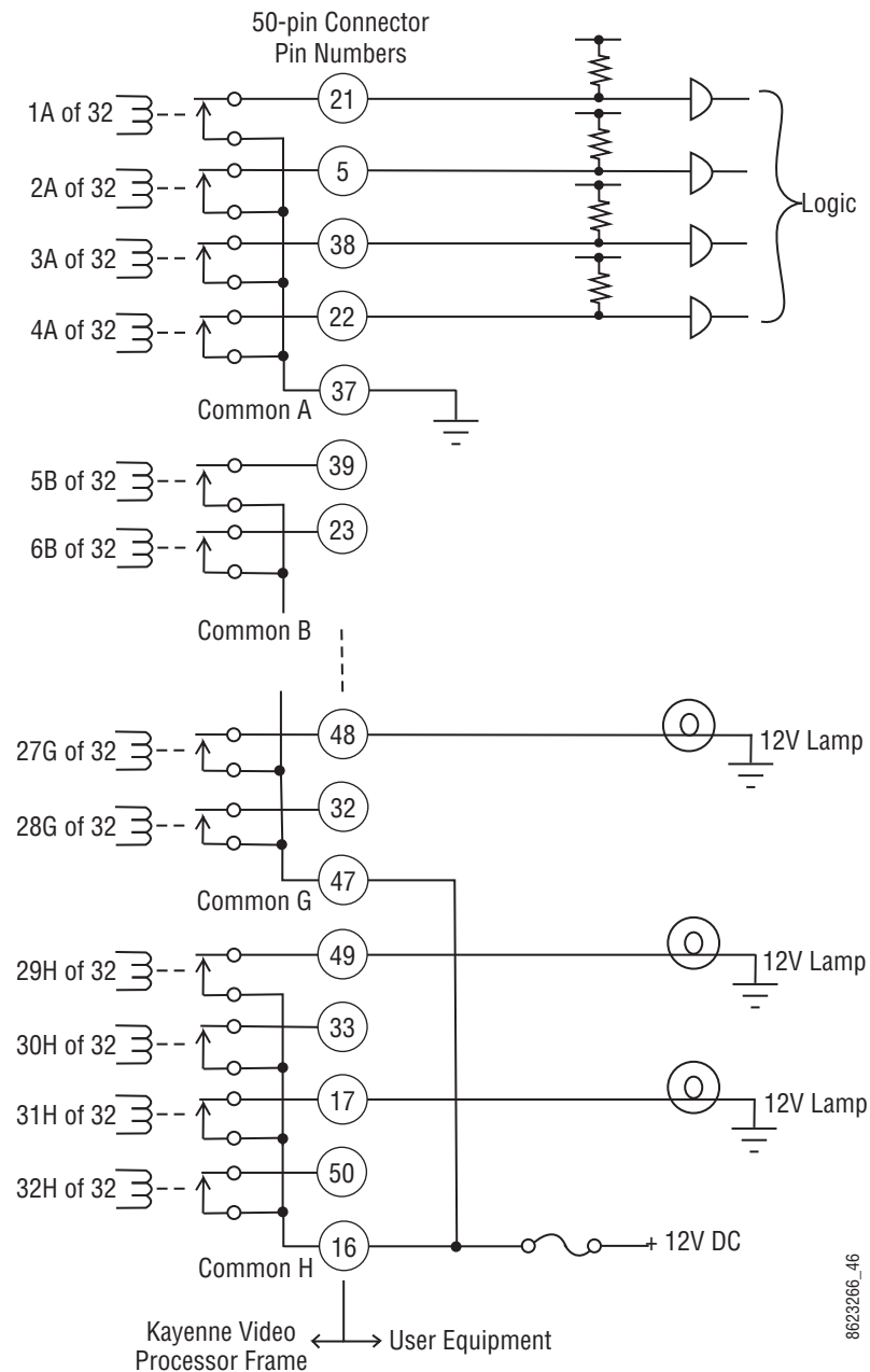
Figure 99. Tally and GPI Output Connection Example
