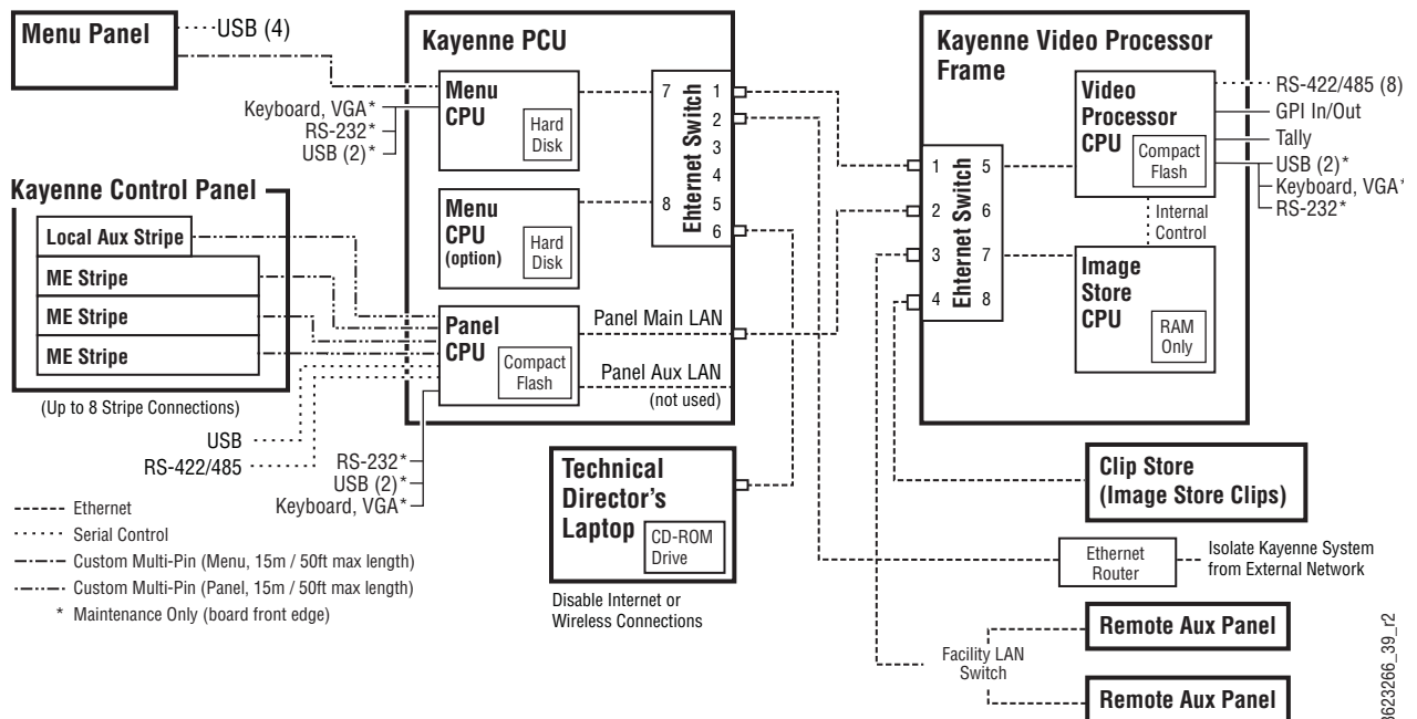
Figure 87. Kayenne System Communications Overview
