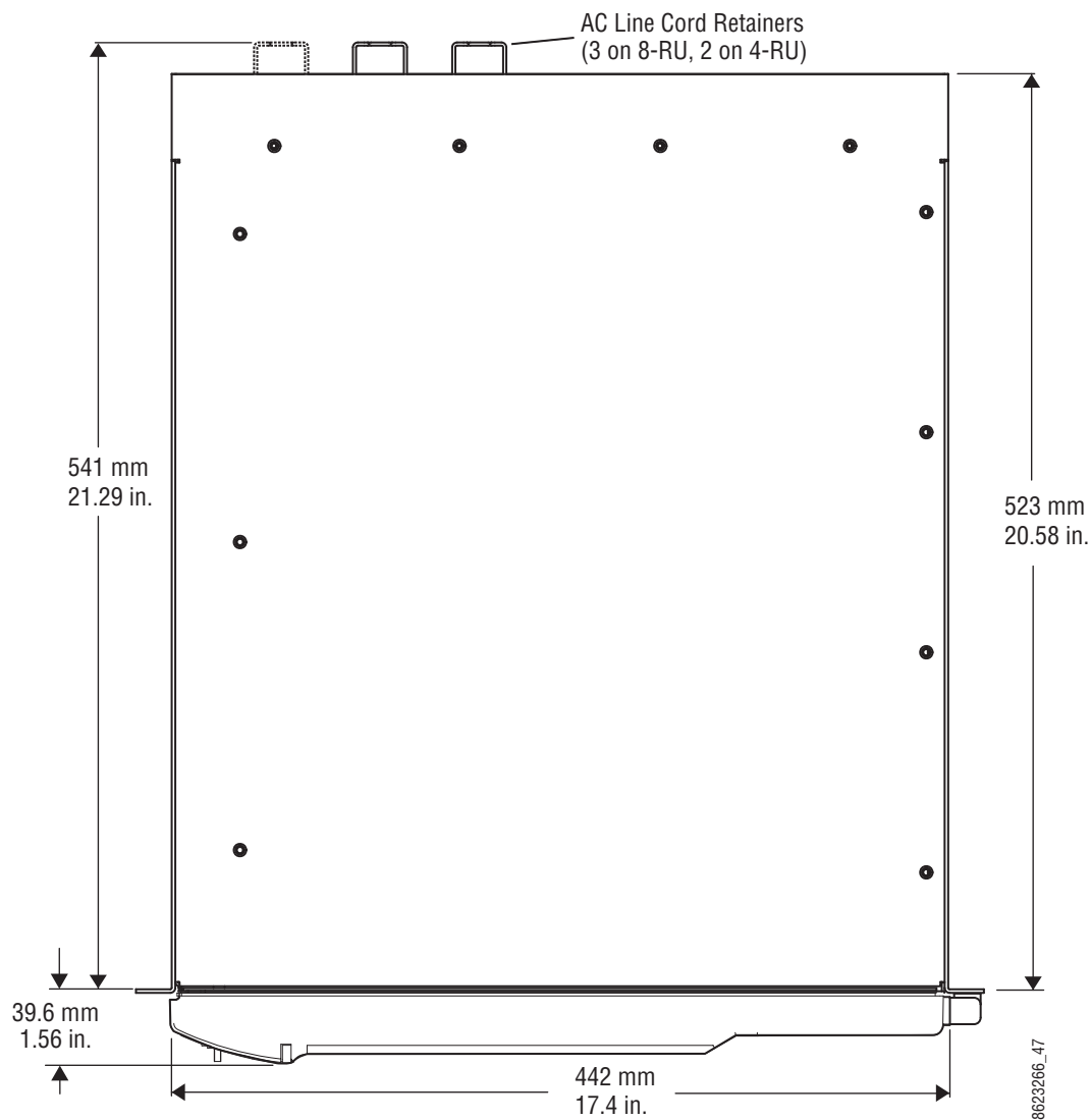
Figure 74. Kayenne 8-RU and 4-RU Frame Dimensions (Top View)
