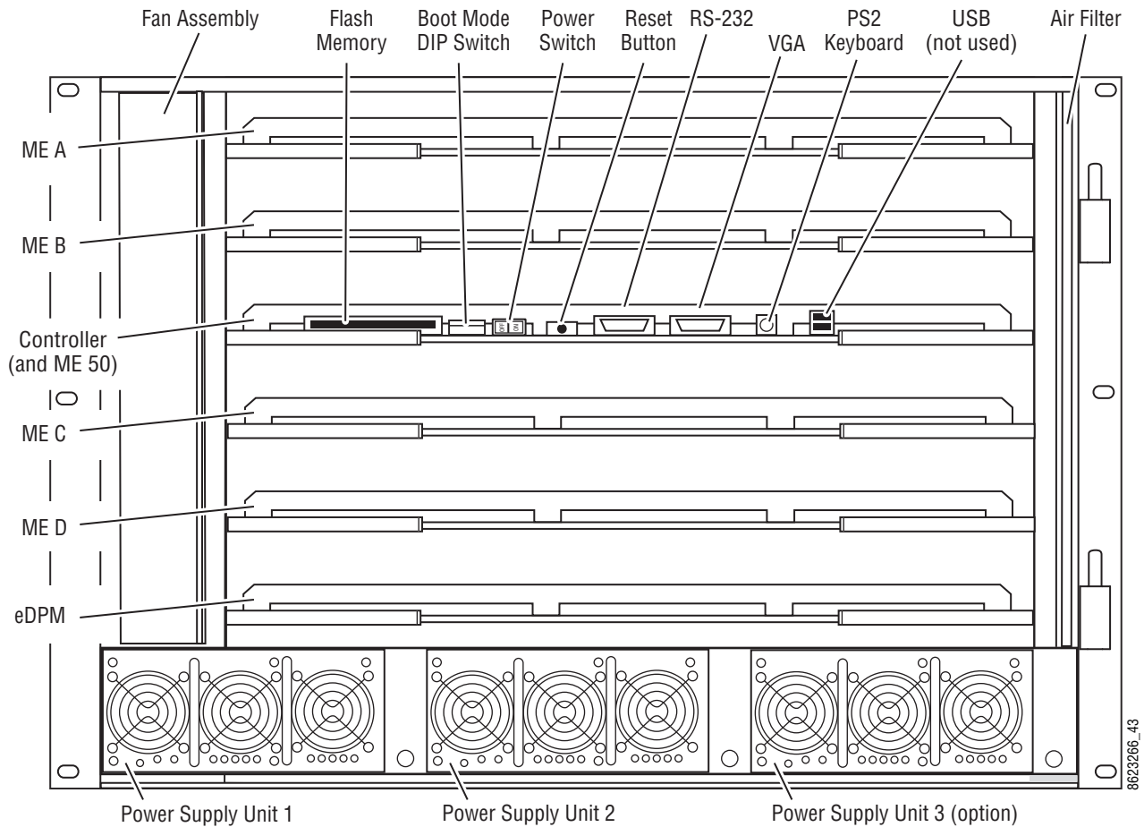
Figure 76. Kayenne 8-RU Frame, Front View with Door Removed
