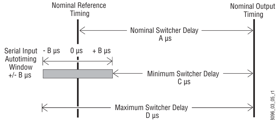
Figure 95. Switcher Timing Diagram
