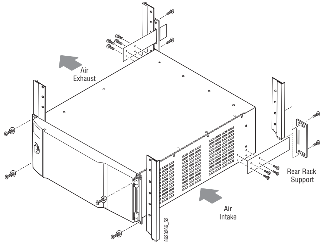
Figure 79. Kayenne 4-RU Frame Rack Installation and Cooling Airflow
