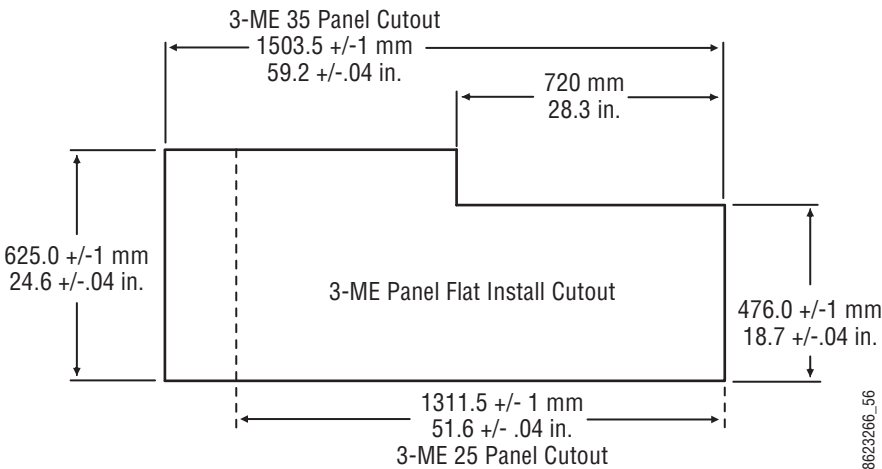
Figure 48. 3-ME Control Panel Cutout Dimensions, Flat Installation
