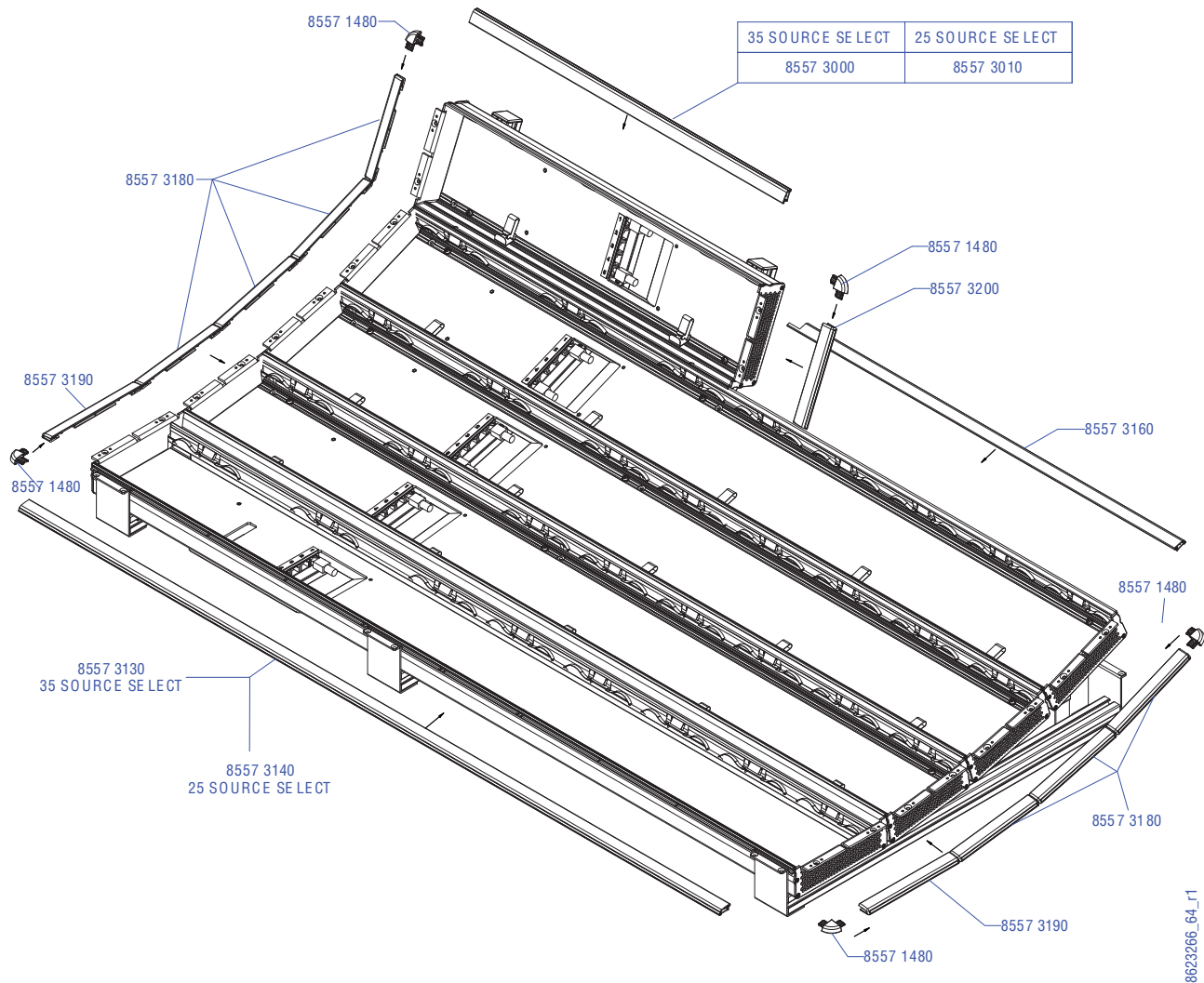
Figure 33. Kayenne 4-ME Control Panel Trim
