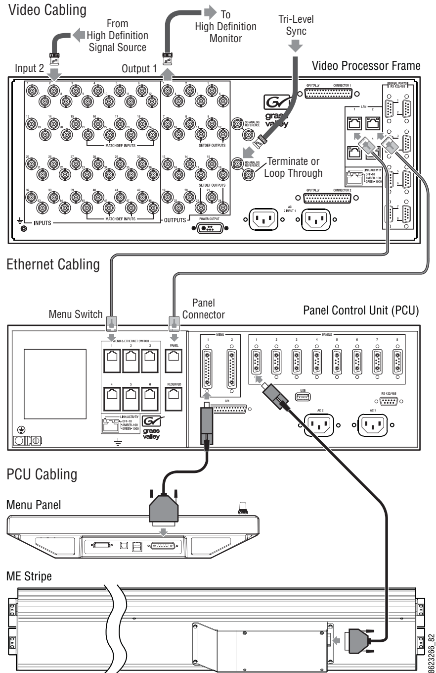
Figure 10. Kayenne Bench Test Cabling
