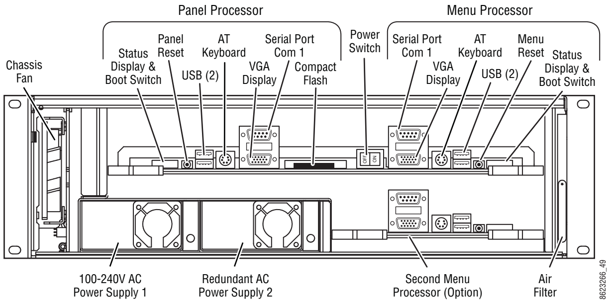
Figure 85. Panel Control Unit, Front View with Door Removed
