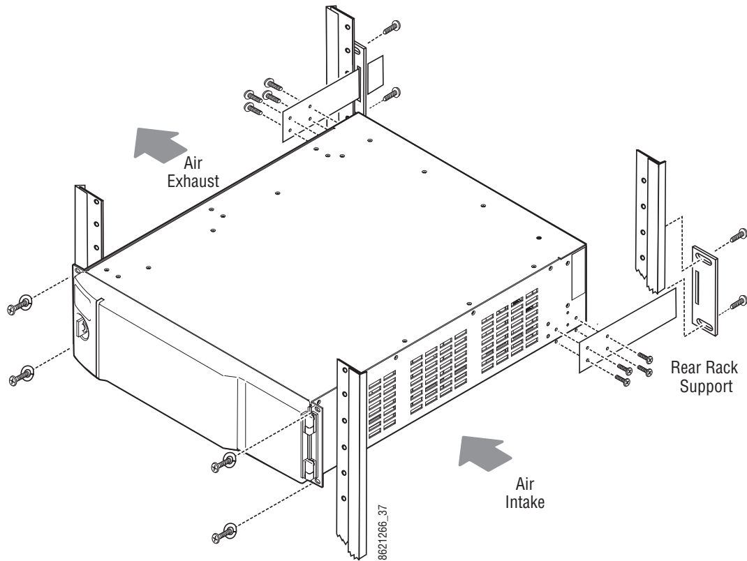
Figure 84. Panel Control Unit Rack Installation and Cooling Airflow
