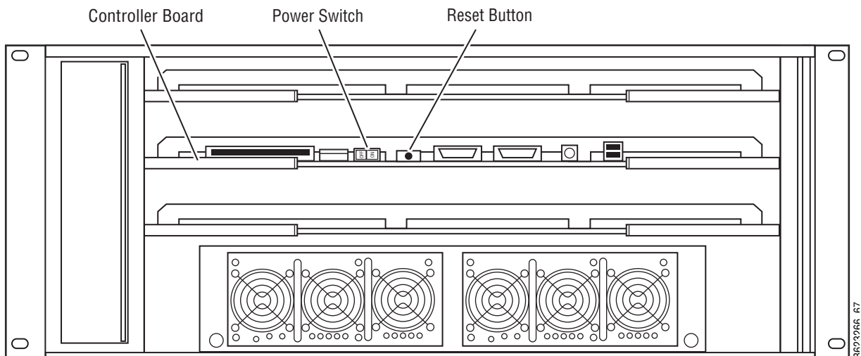
Figure 209. 4-RU Video Processor Frame Reset Button and Power Switch
