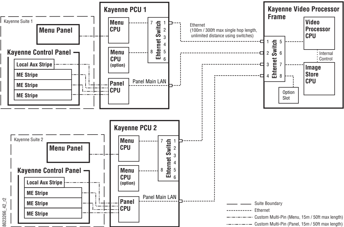
Figure 90. Two Suites Using Two PCUs
