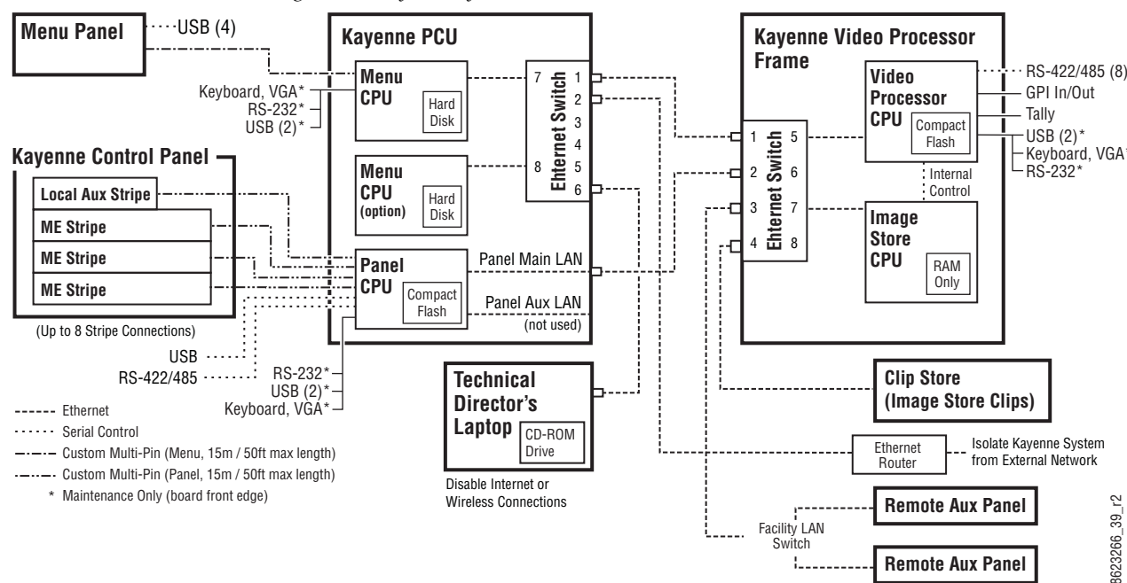
Figure 91. Kayenne System Communications Overview
