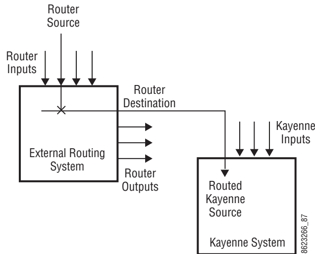
Figure 205. Router Source, Router Destination, and Routed Kayenne Source
