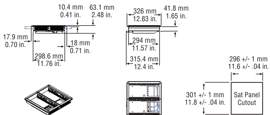
Figure 68. Double Module Satellite Panel Installation Dimensions
