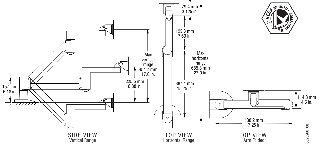
Figure 72. Articulated Arm Range of Motion Dimensions
