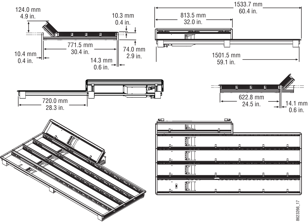
Figure 34. 4-ME 35 Control Panel Dimensions, Flat Installation
