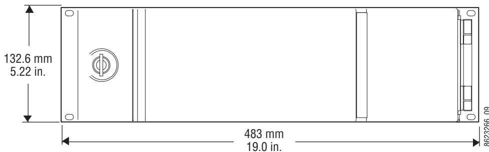
Figure 82. Panel Control Unit Dimension (Front View)
