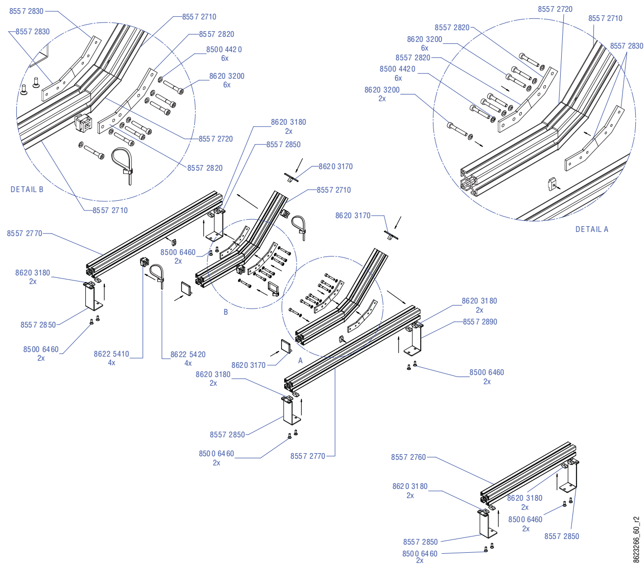
Figure 56. 2-ME Support Structure, Flat Installation
