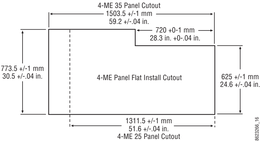
Figure 35. 4-ME Control Panel Cutout Dimensions, Flat Installation
