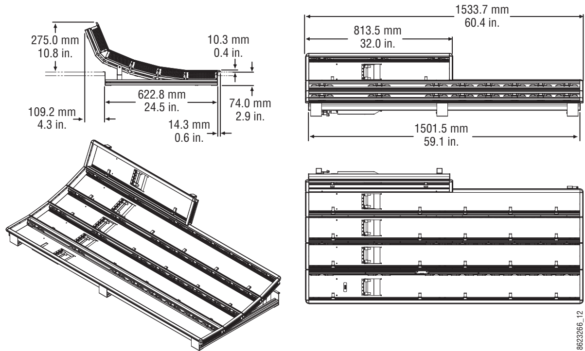
Figure 16. 4-ME 35 Control Panel Dimensions, Curved Installation
