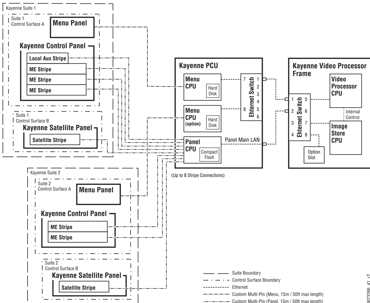
Figure 89. Two Suites with Two Control Surfaces Using One PCU
