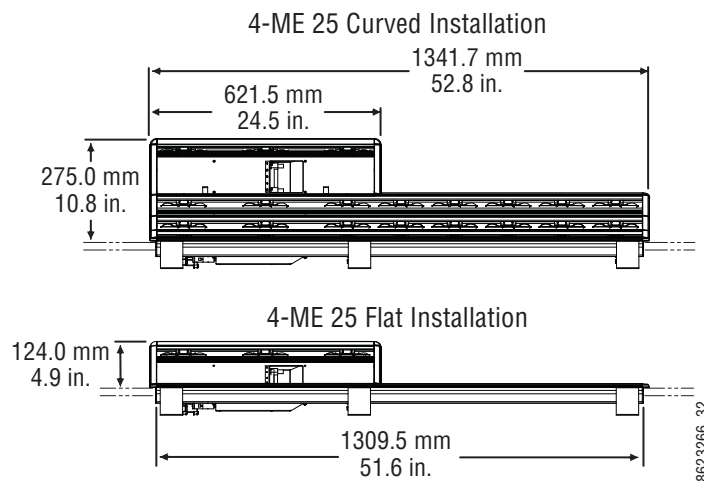
Figure 43. 4-ME 25 Control Panel Dimensions
