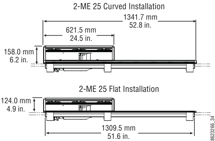
Figure 60. 2-ME 25 Control Panel Dimensions
