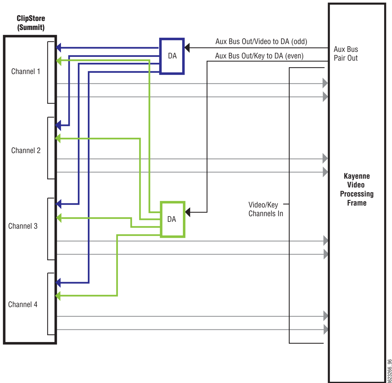
Figure 94. ClipStore Connection Using Distribution Amplifiers
