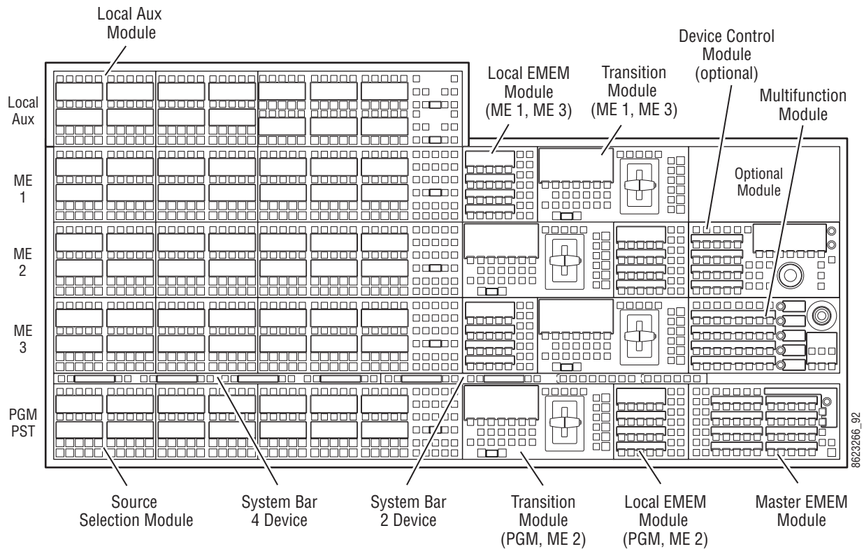
Figure 32. Kayenne 4-ME Control Panel Recommended Module Placement
