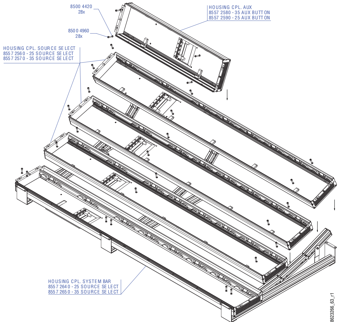
Figure 29. 4-ME Curved Control Panel Tray Assembly
