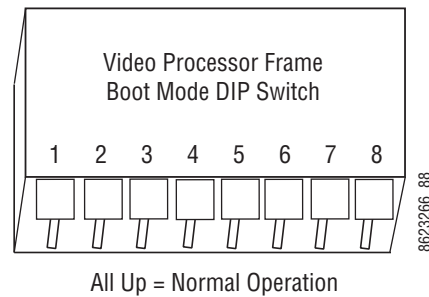
Figure 229. Kayenne Control Processor Board - Boot Mode Switch Setting
