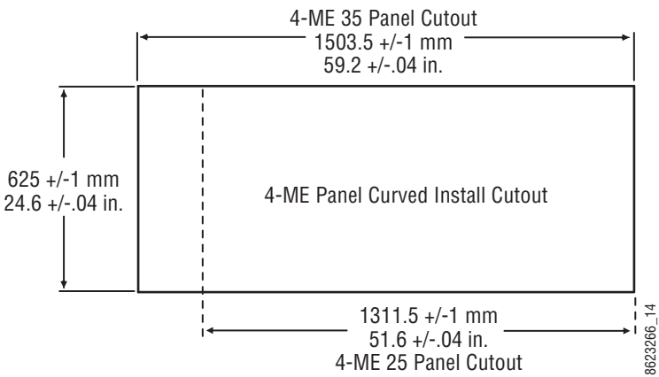
Figure 17. 4-ME Control Panel Cutout Dimensions, Curved Installation
