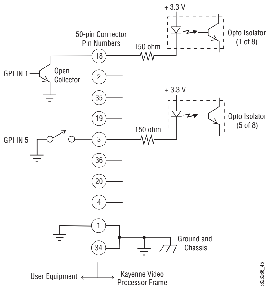
Figure 98. GPI Input Connections (Typical 2 of 8 Connections)
