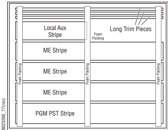
Control Surface Crate, Top Layer
