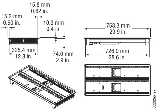
Figure 61. 1-ME 15 Control Panel Dimensions, Flat Installation
