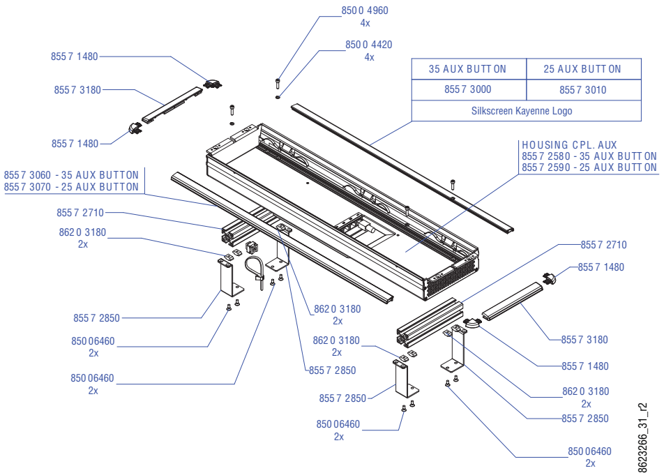
Figure 65. Local Aux Stripe Support Structure, Tray, and Trim
