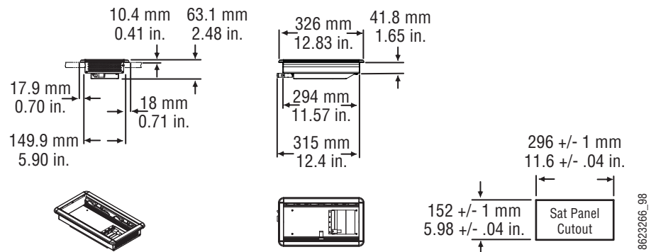
Figure 66. Single Module Satellite Panel Installation Dimensions
