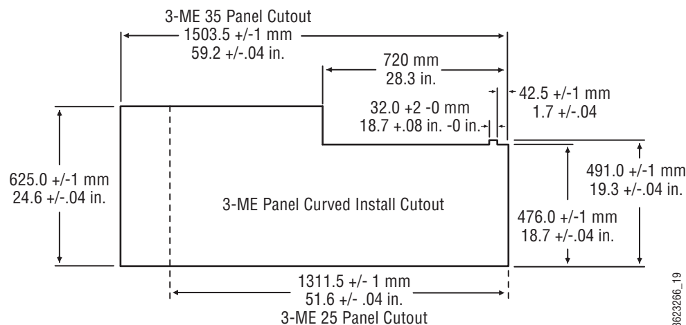
Figure 45. 3-ME Control Panel Cutout Dimensions, Curved Installation
