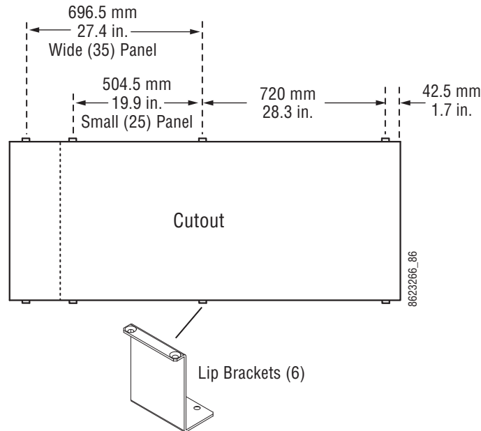
Figure 30. Control Panel Mounting Detail
