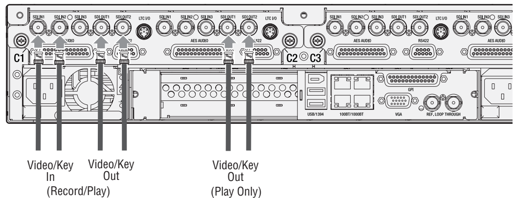
Figure 92. ClipStore Backplane Connections
