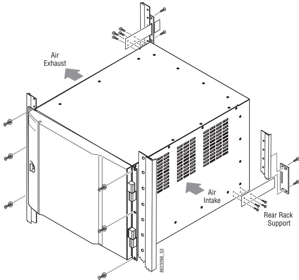
Figure 75. Kayenne 8-RU Frame Rack Mounting and Cooling Airflow
