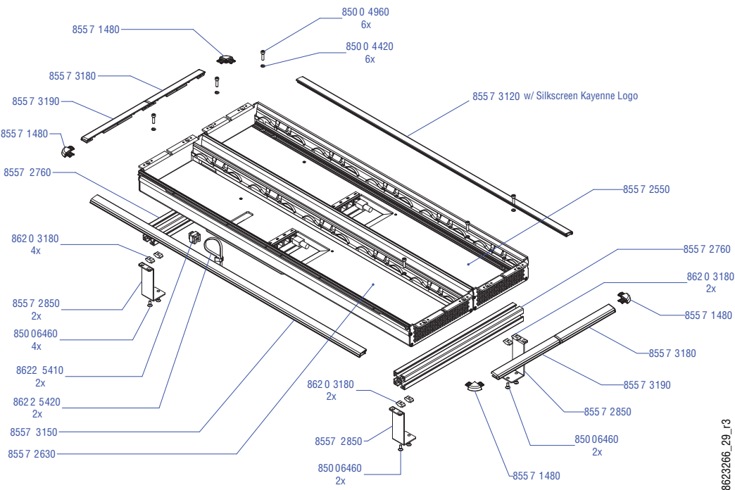
Figure 63. 1-ME Support Structure and Trim, Flat Installation
