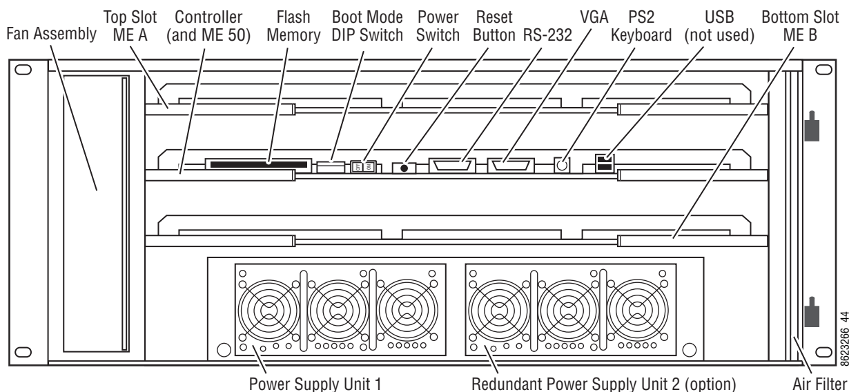
Figure 80. Kayenne 4-RU Frame, Front View with Door Removed
