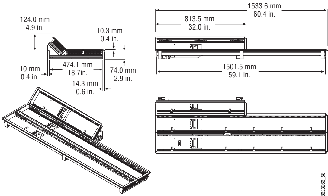
Figure 54. 2-ME 35 Control Panel Dimensions, Flat Installation
