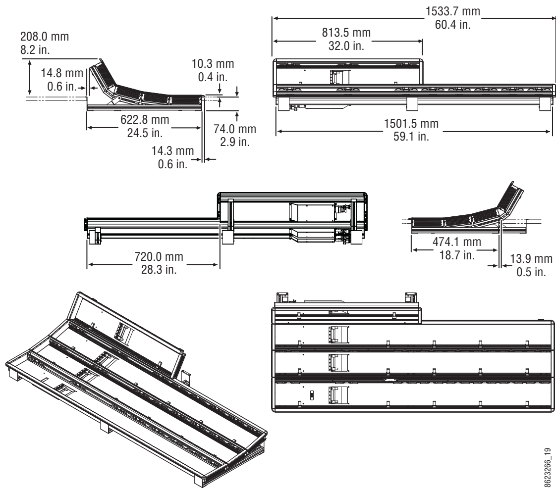
Figure 44. 3-ME 35 Control Panel Dimensions, Curved Installation
