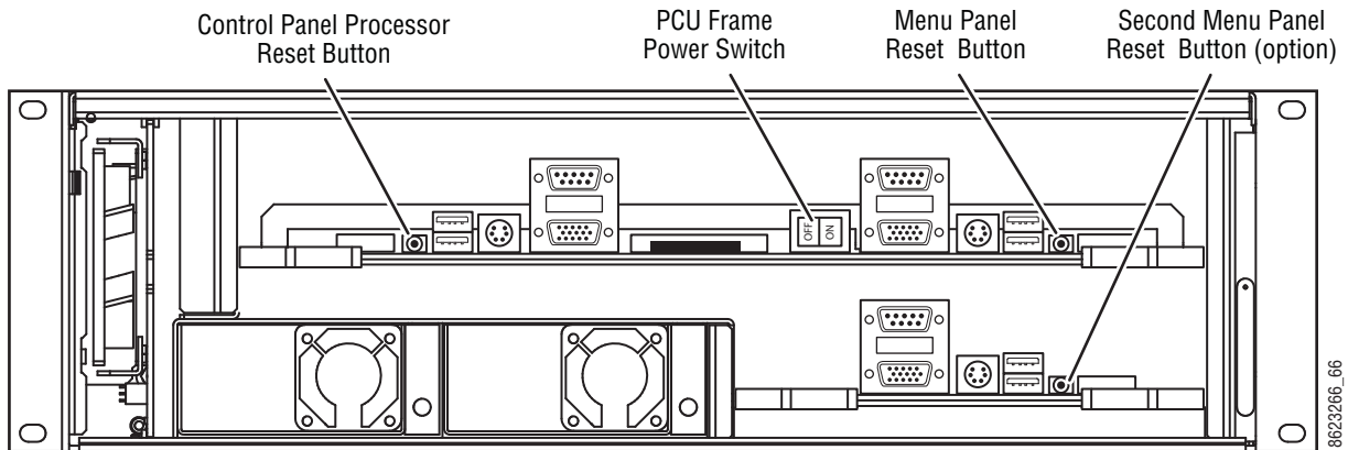
Figure 210. PCU Reset Buttons and Power Switch
