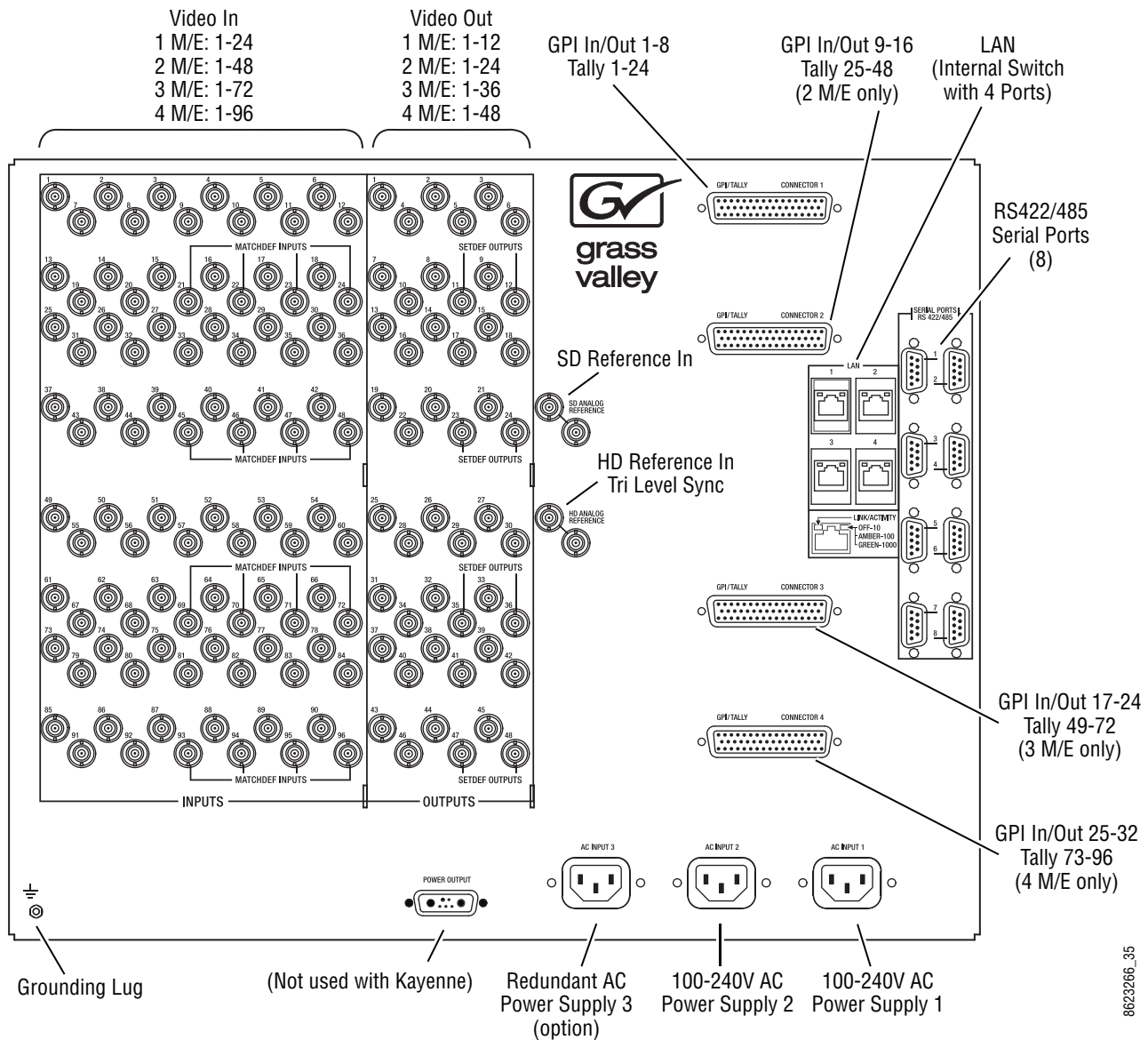
Figure 77. Kayenne 8-RU Frame, Backplane View
