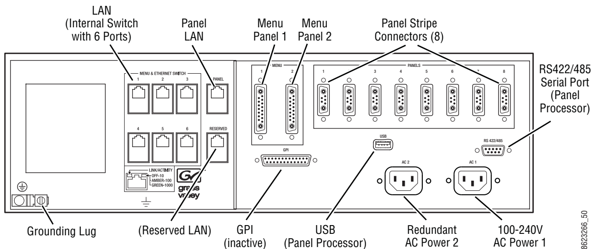
Figure 86. Panel Control Unit, Backplane View
