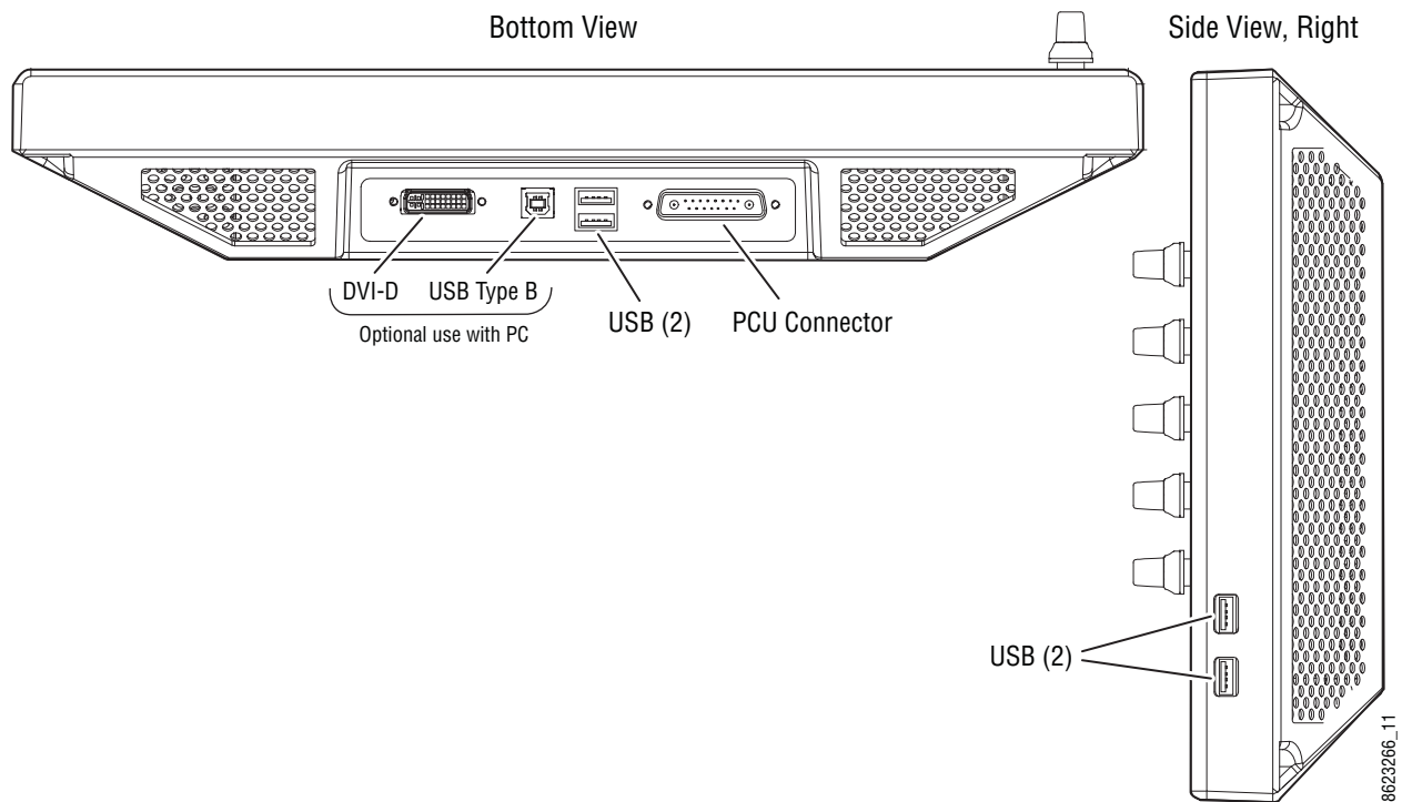
Figure 71. Menu Panel Connections
