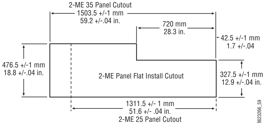
Figure 55. 2-ME Control Panel Cutout Dimensions, Flat Installation
