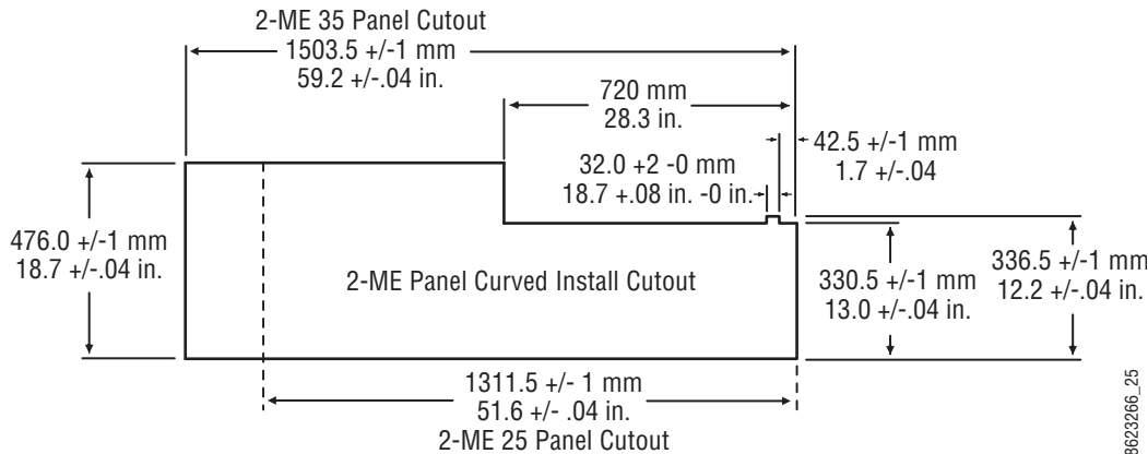
Figure 52. 2-ME Control Panel Cutout Dimensions, Curved Installation
