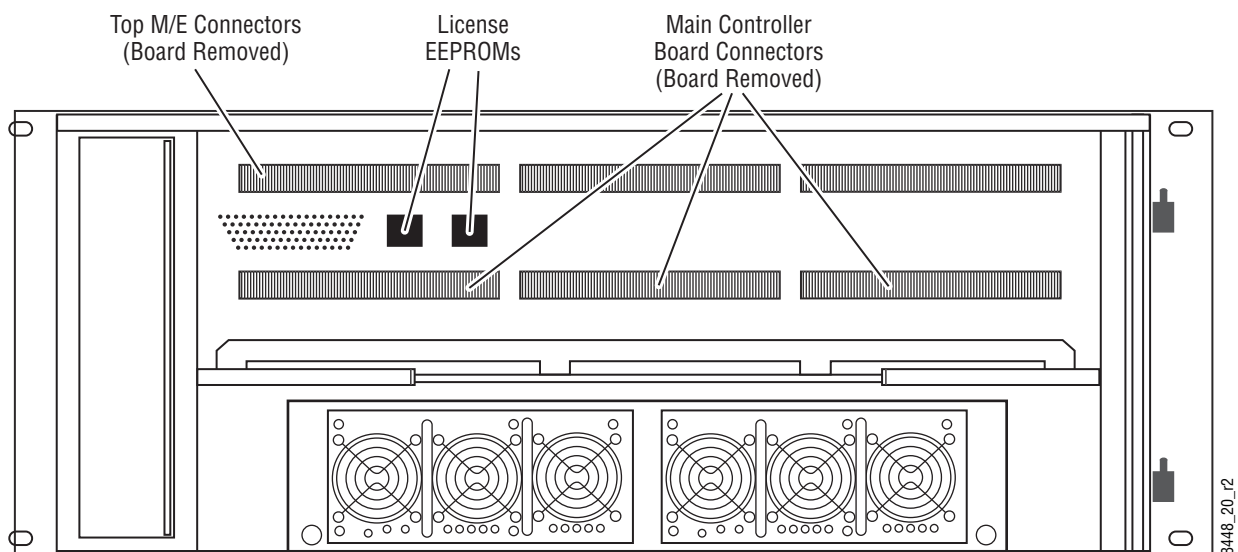
Figure 230. License EEPROMs in 4-RU Frame, Top Two Boards Removed
