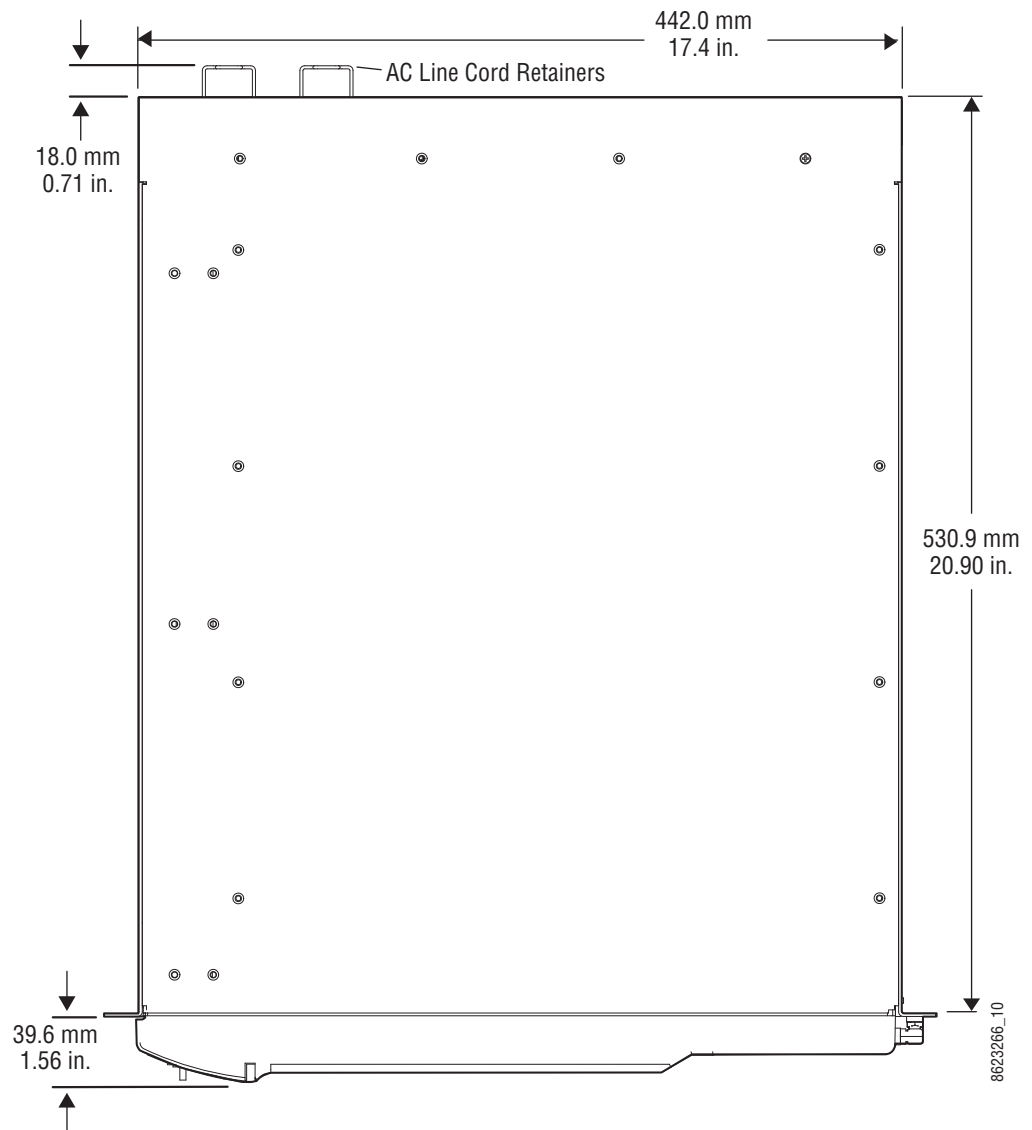
Figure 83. Panel Control Unit Dimensions (Top View)
