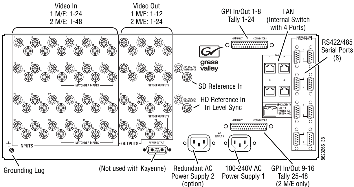
Figure 81. Kayenne 4-RU Frame, Backplane View
