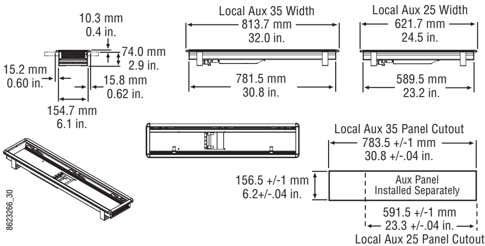
Figure 64. Local Aux Stripe Separate Installation Dimensions
