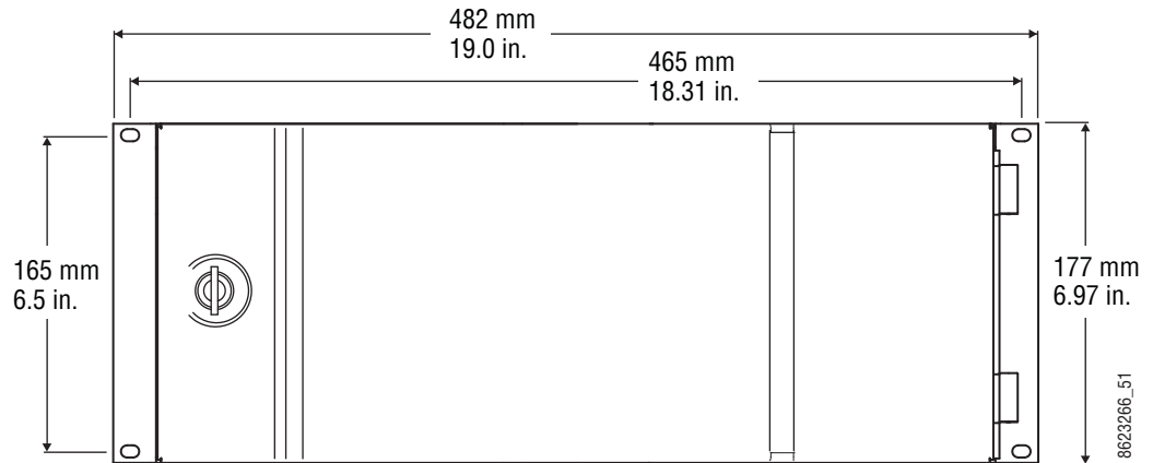
Figure 78. Kayenne 4-RU Frame Dimensions (Front View)
