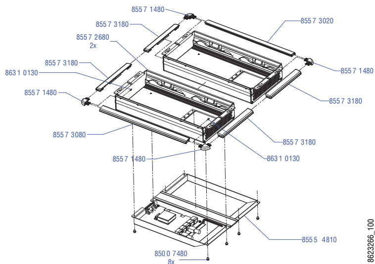
Figure 69. Double Module Satellite Panel Tray and Trim
