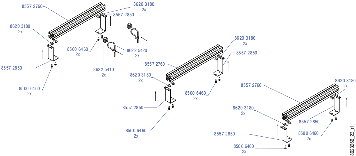
Figure 59. 2-ME Support Structure, Flat Installation, w/o Local Aux Stripe
