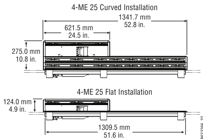
Figure 43. 4-ME 25 Control Panel Dimensions
