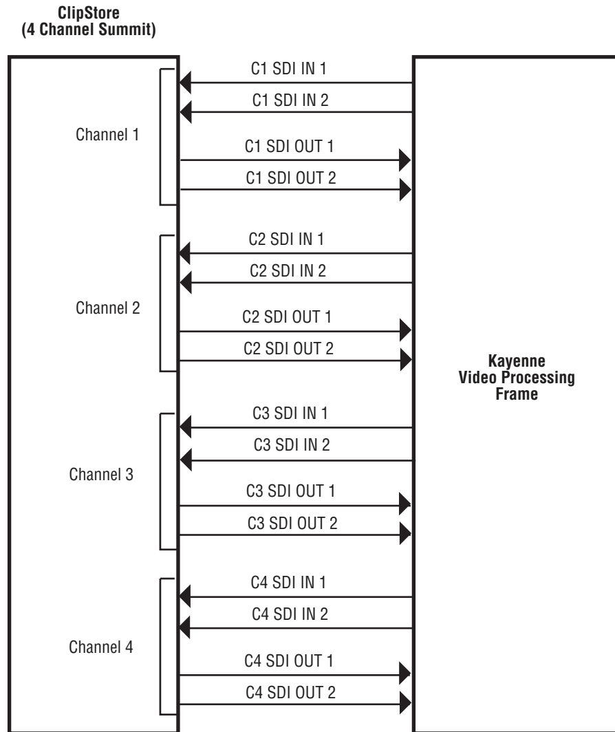
Figure 93. ClipStore Direct Connection
