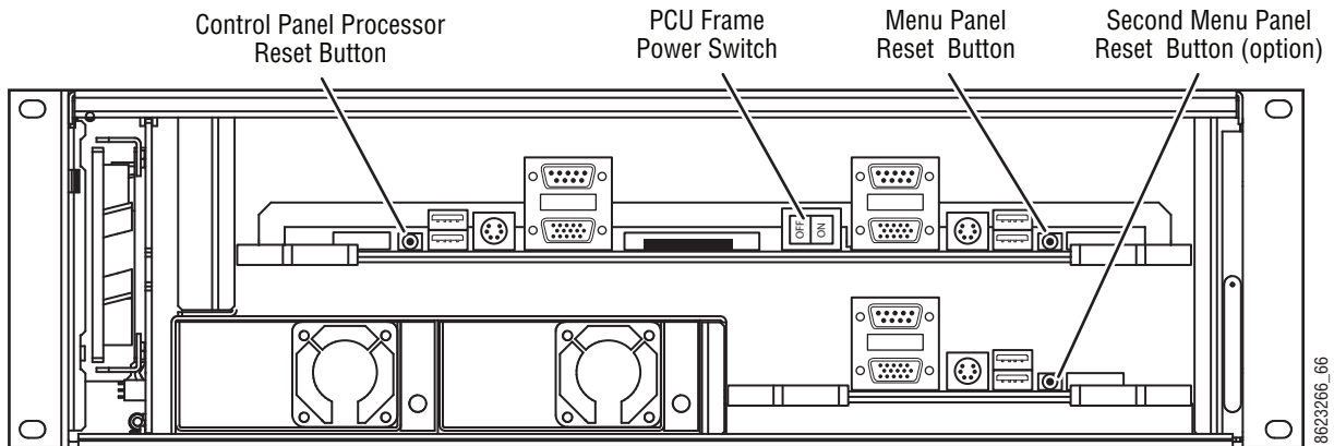
Figure 217. PCU Reset Buttons and Power Switch
