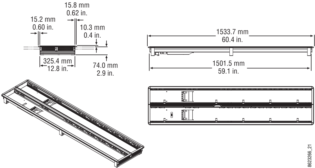
Figure 57. 2-ME 35 Control Panel Dimensions, Flat Installation
