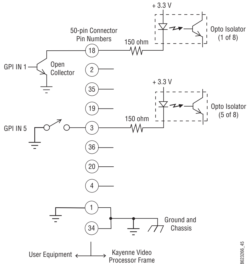
Figure 98. GPI Input Connections (Typical 2 of 8 Connections)
