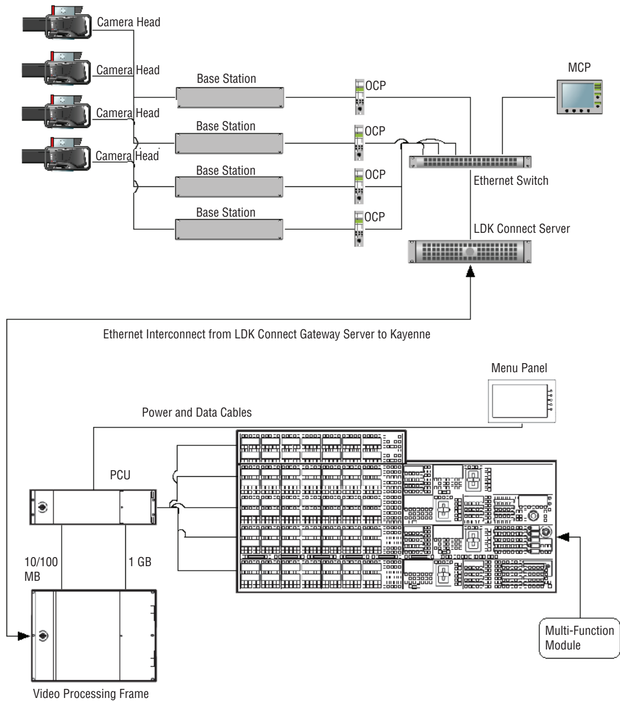
Figure 145. Kayenne System Interconnection with Camera Gateway
