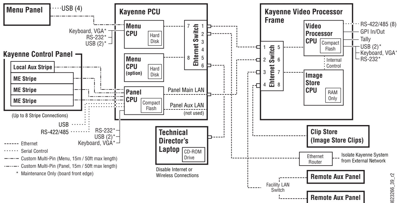
Figure 91. Kayenne System Communications Overview
