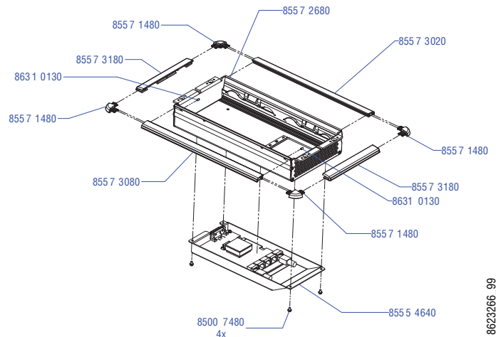
Figure 67. Single Module Satellite Panel Tray and Trim
