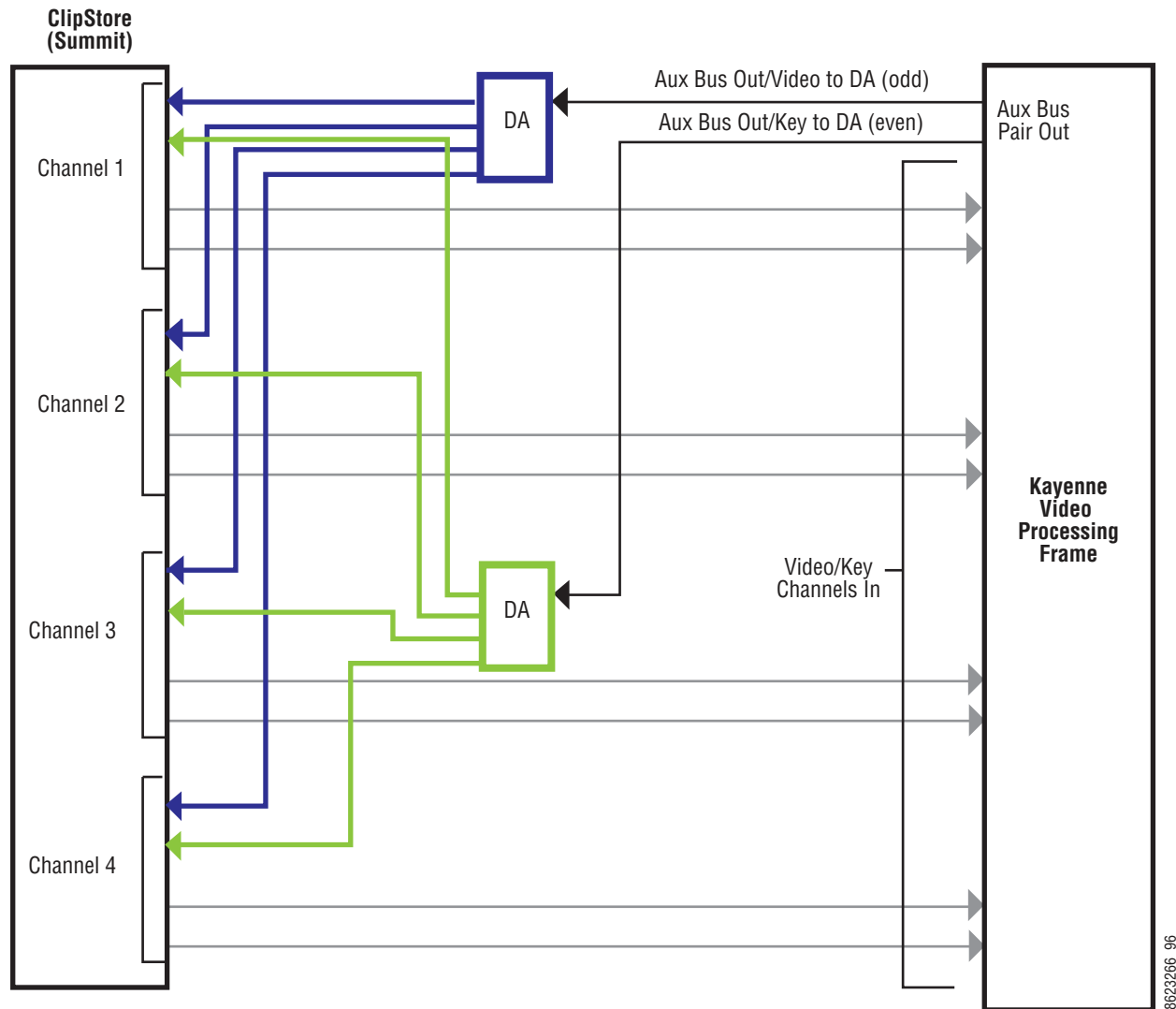
Figure 94. ClipStore Connection Using Distribution Amplifiers
