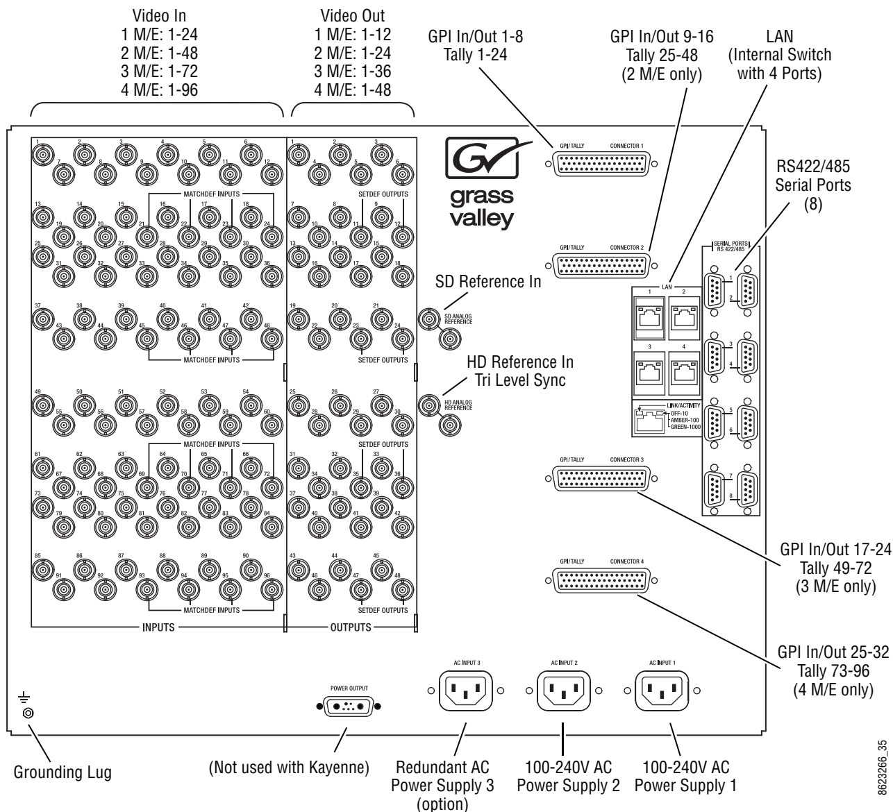
Figure 77. Kayenne 8-RU Frame, Backplane View
