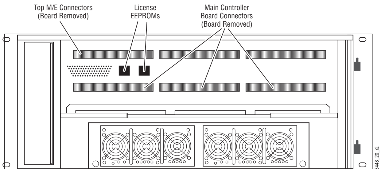
Figure 237. License EEPROMs in 4-RU Frame, Top Two Boards Removed
