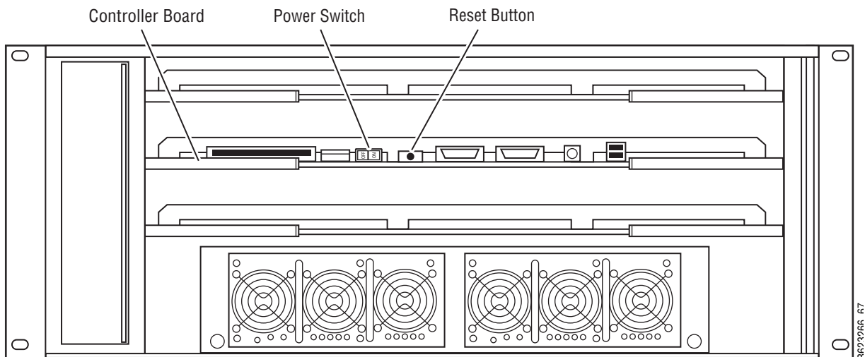
Figure 216. 4-RU Video Processor Frame Reset Button and Power Switch
