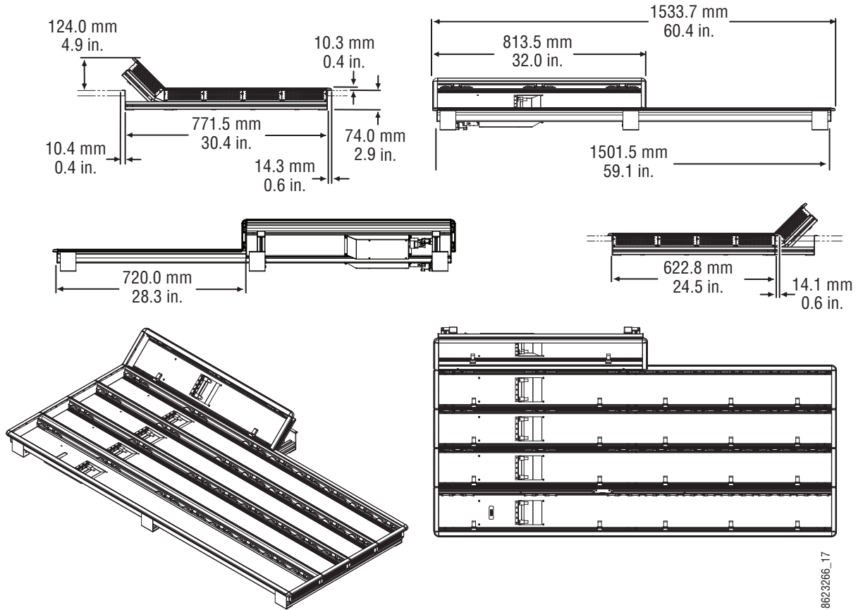
Figure 34. 4-ME 35 Control Panel Dimensions, Flat Installation
