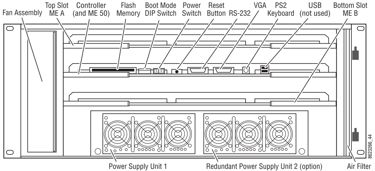
Figure 80. Kayenne 4-RU Frame, Front View with Door Removed
