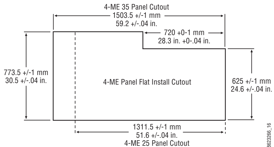
Figure 35. 4-ME Control Panel Cutout Dimensions, Flat Installation
