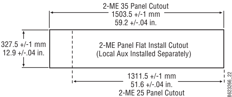
Figure 58. 2-ME Control Panel Cutout Dimensions, Flat Installation
