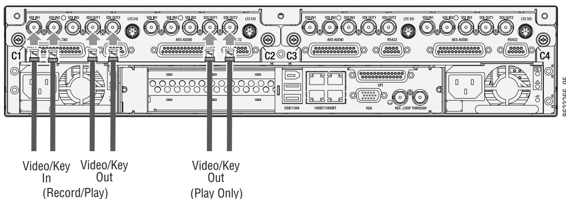
Figure 92. ClipStore Backplane Connections
