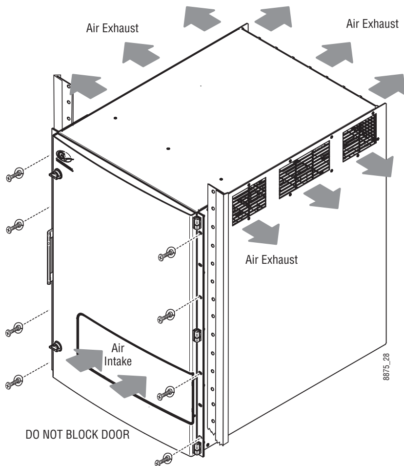
15-RU Rack Mounting and Cooling Airflow
