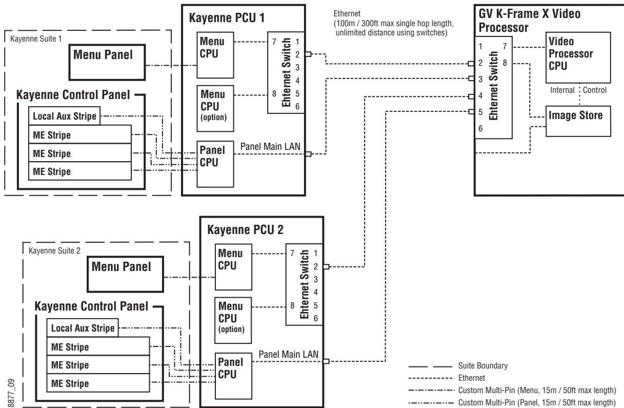
GV K-Frame X/Kayenne Two Suites Using Two PCUs
