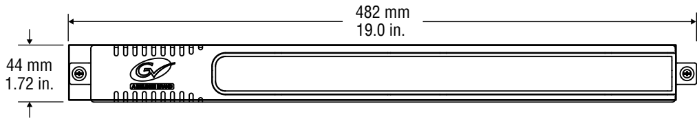
Front View Cover Removed
