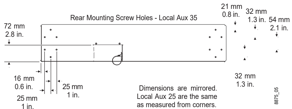
Local Aux Panel Rear Dimensions
