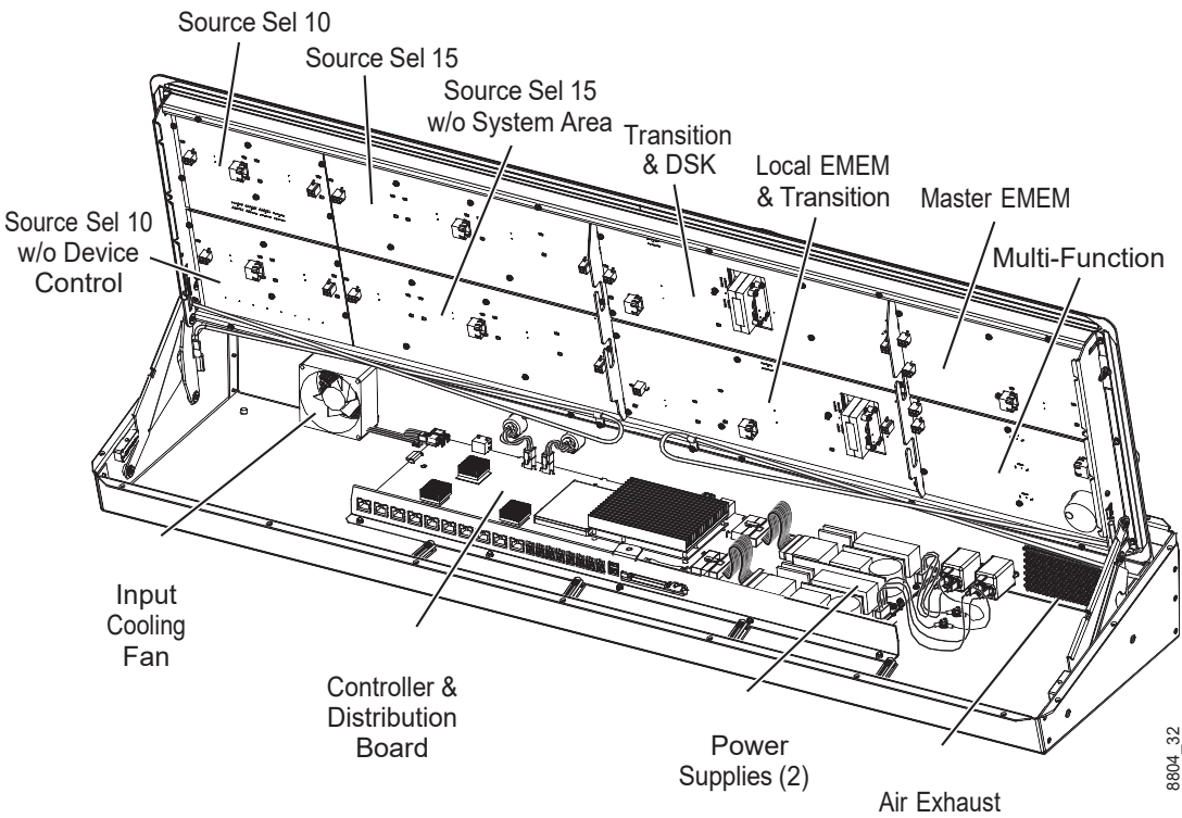
Karrera 2-ME Panel Open, Air Guide Removed
