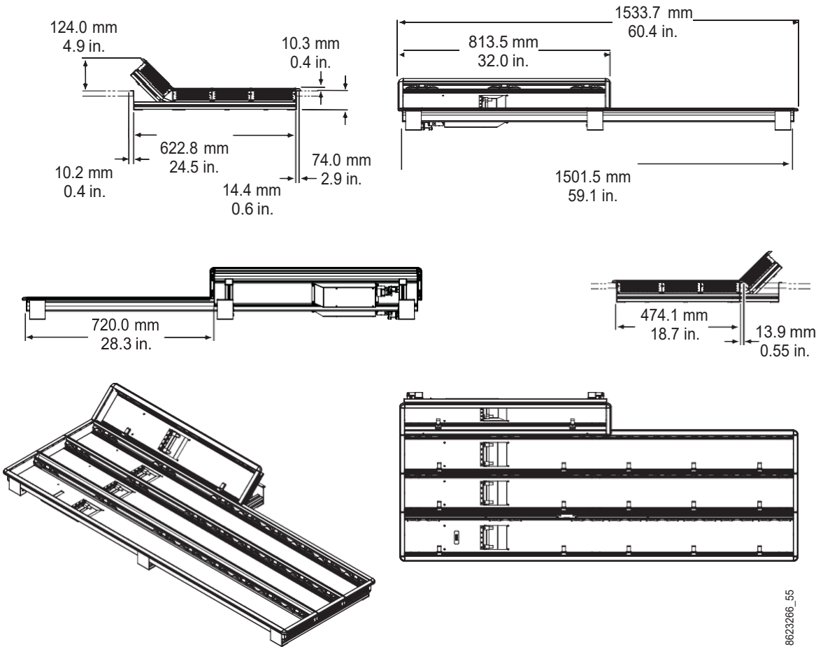
3-M/E 35 Control Panel Dimensions, Flat Installation
