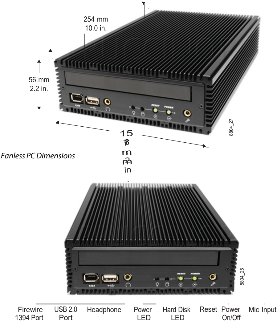
Fanless PC Front Connectors
