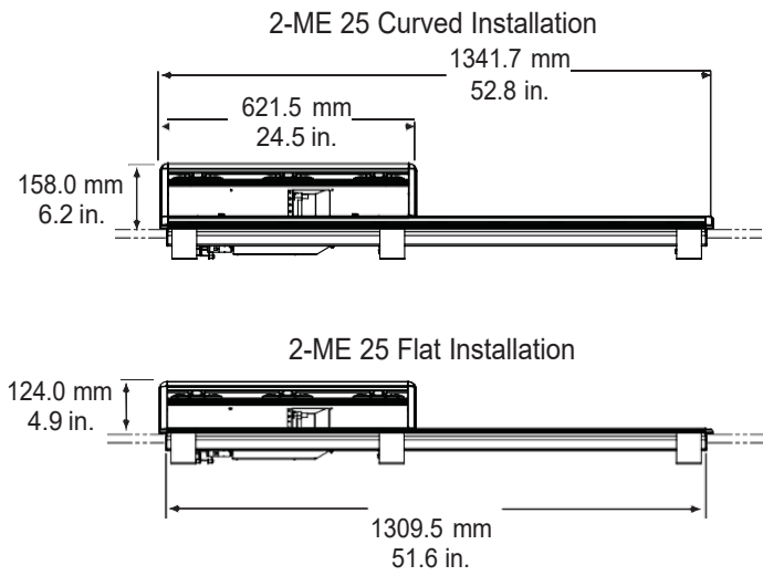
2-M/E 25 Control Panel Dimensions
