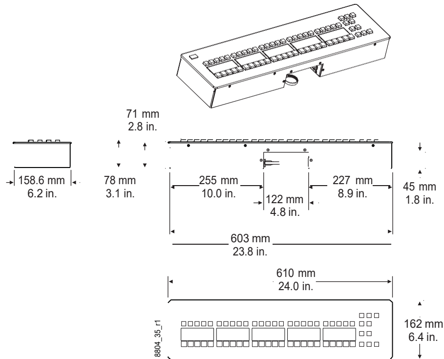
Local Aux 25 Panel Dimensions
