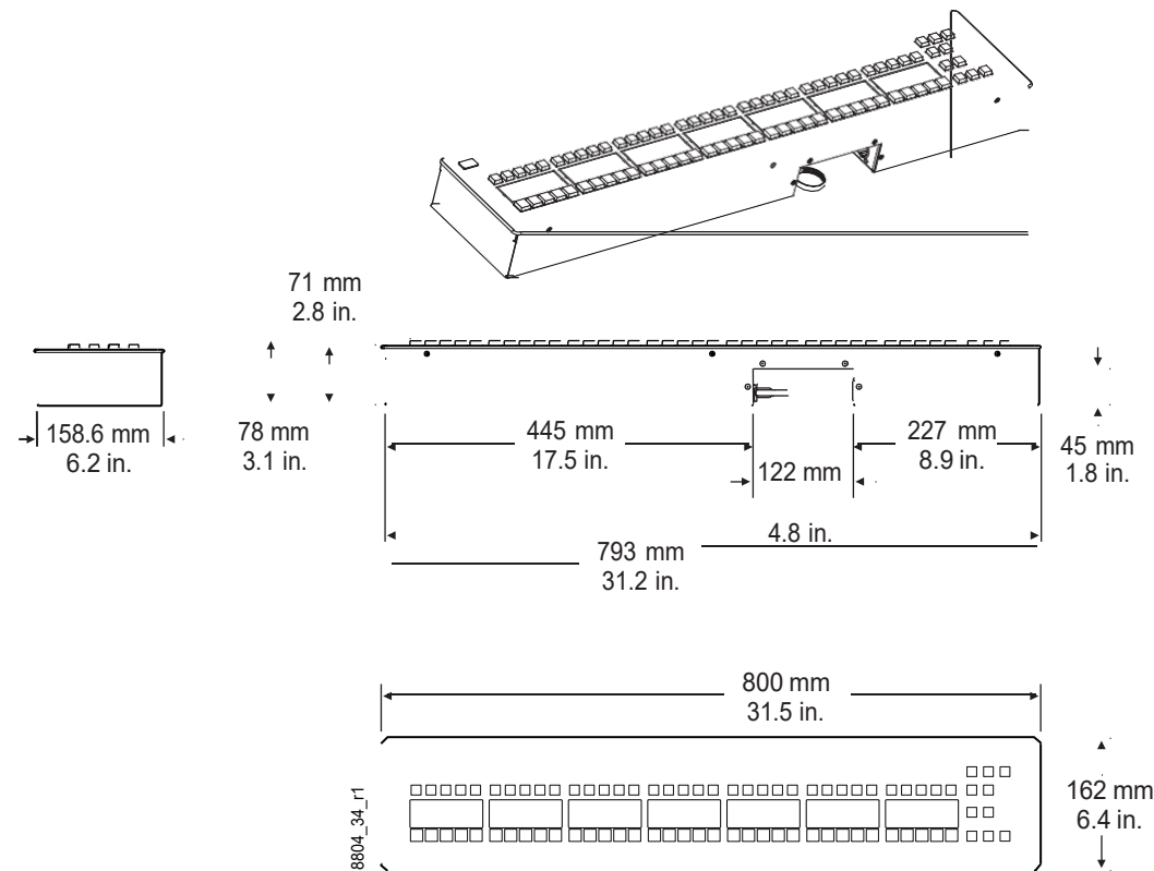
Local Aux 35 Panel Dimensions
