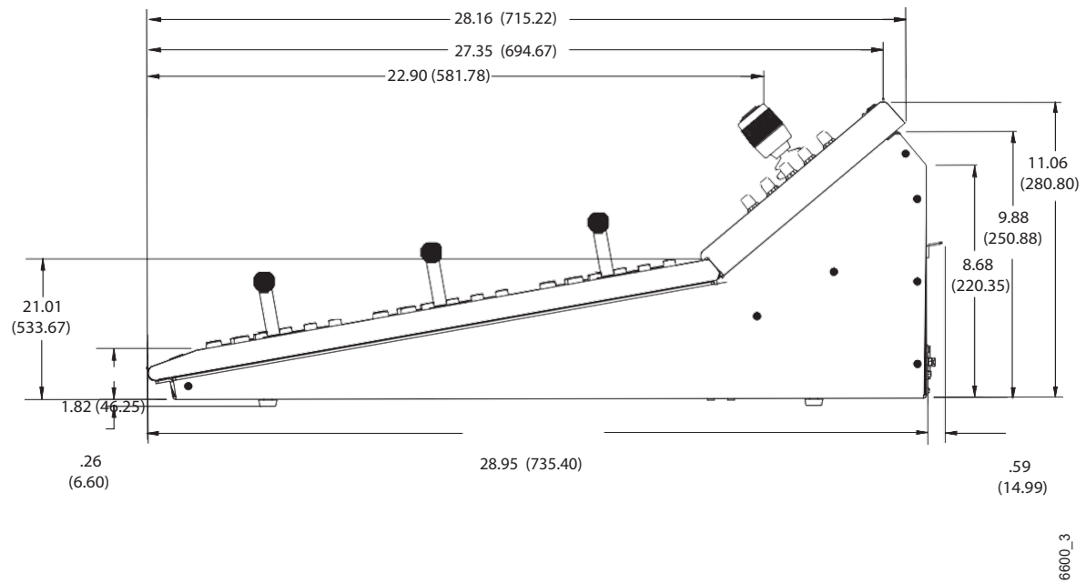
3-M/E GV Korona Control Panel Side Dimensions
