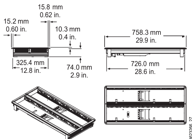
1-M/E 15 Control Panel Dimensions, Flat Installation
