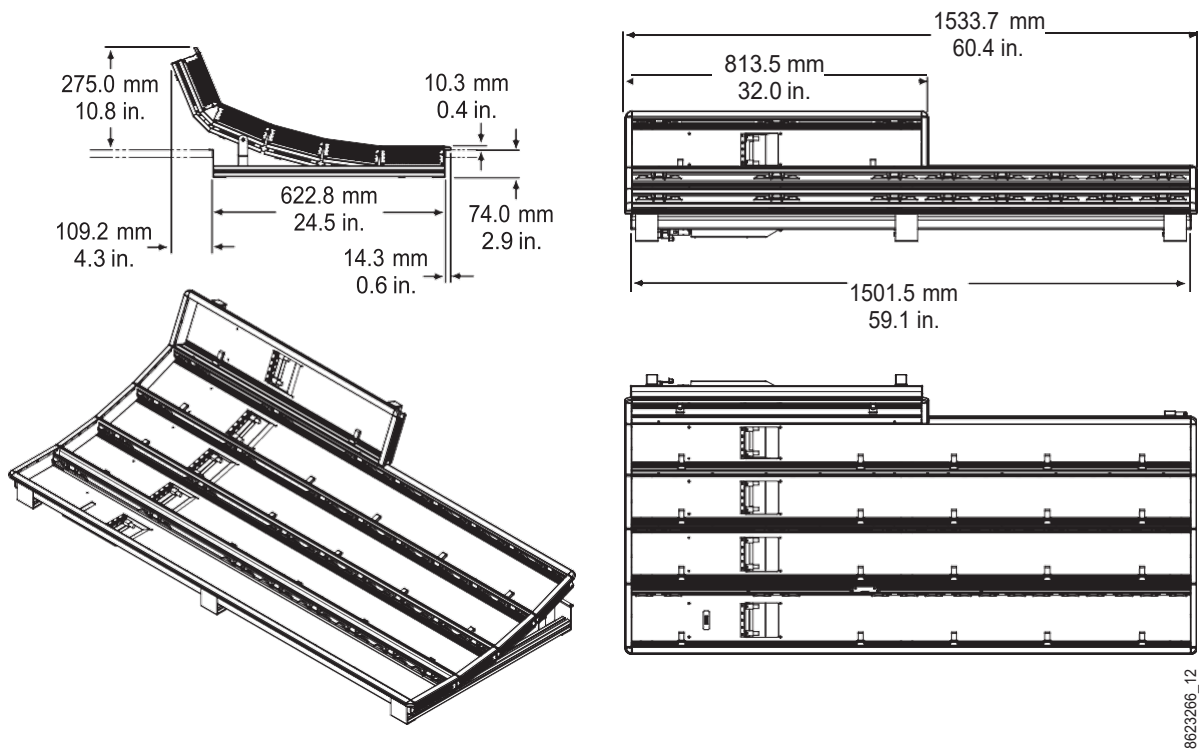
4-M/E 35 Control Panel Dimensions, Curved Installation
