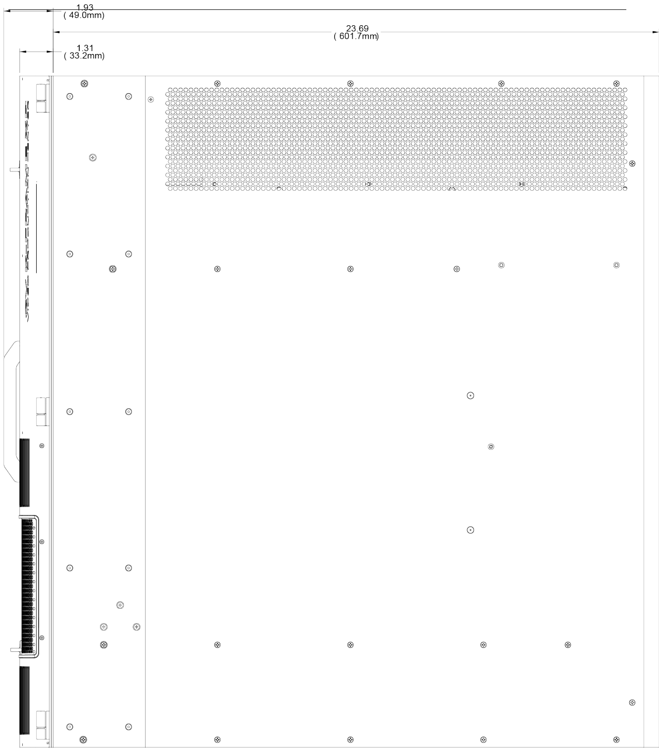
15-RU Dimensions (Side View)
