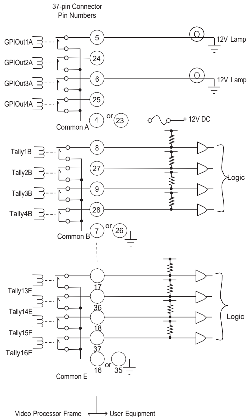
Relay Tally and GPI Output Connection Example
