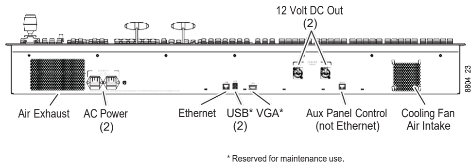
3-M/E Karrera Control Panel Rear Connections
