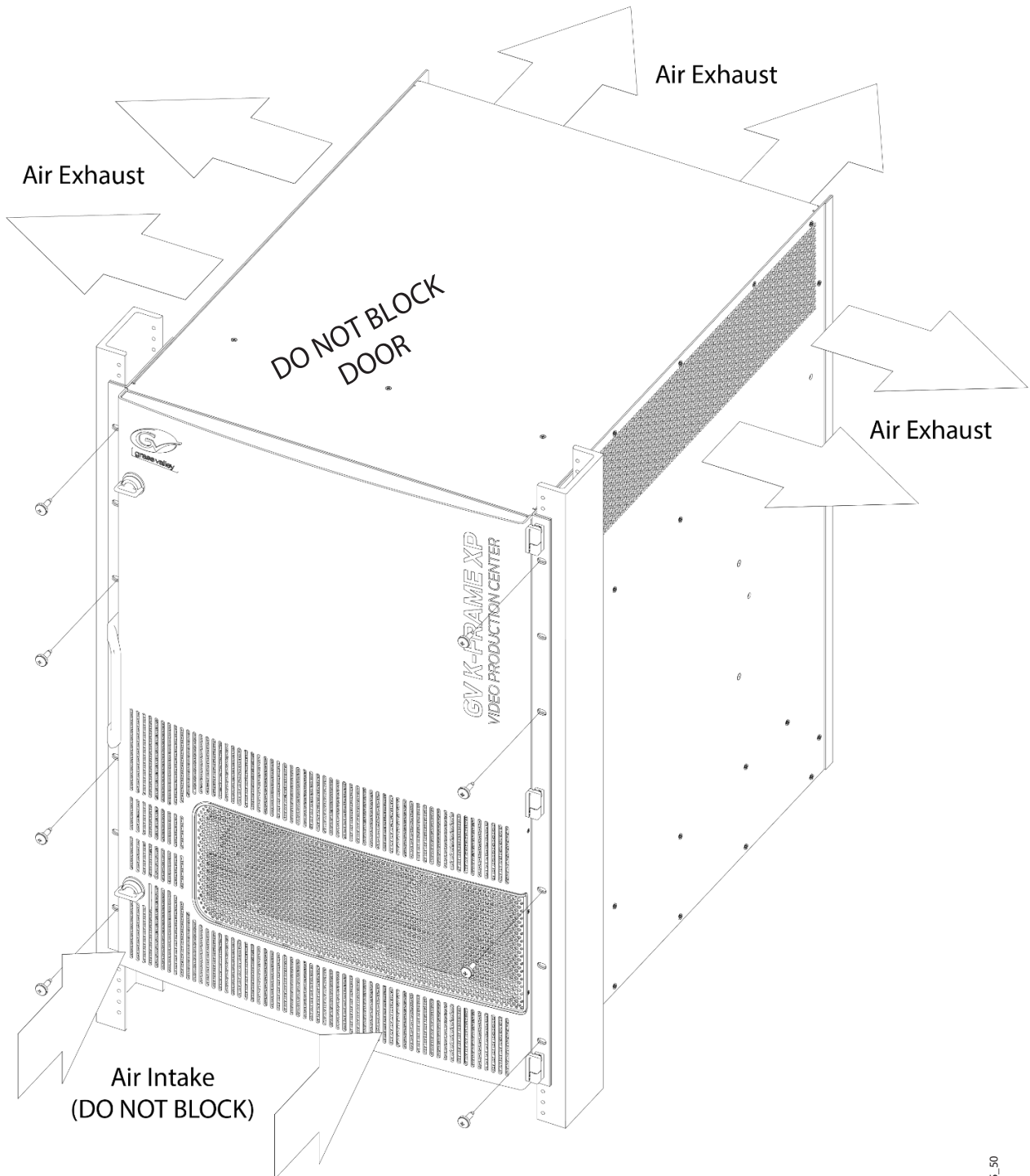
15-RU Rack Mounting and Cooling Airflow
