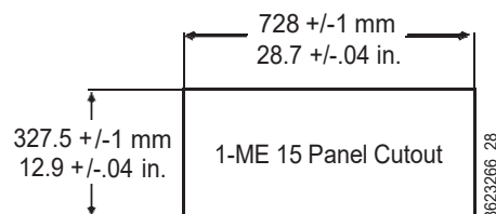
1-M/E 15 Control Panel Cutout Dimensions, Flat Installation
