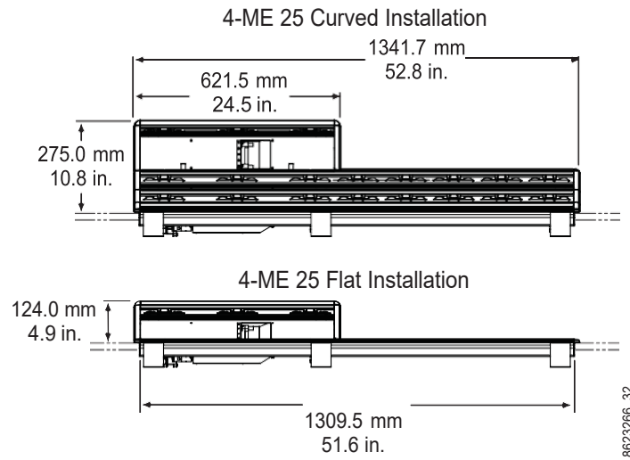
4-M/E 25 Control Panel Dimensions
