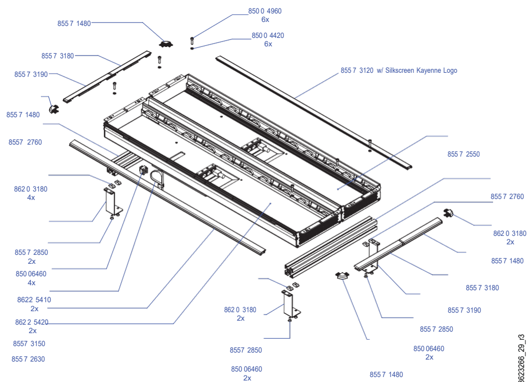
1-M/E Support Structure and Trim, Flat Installation
