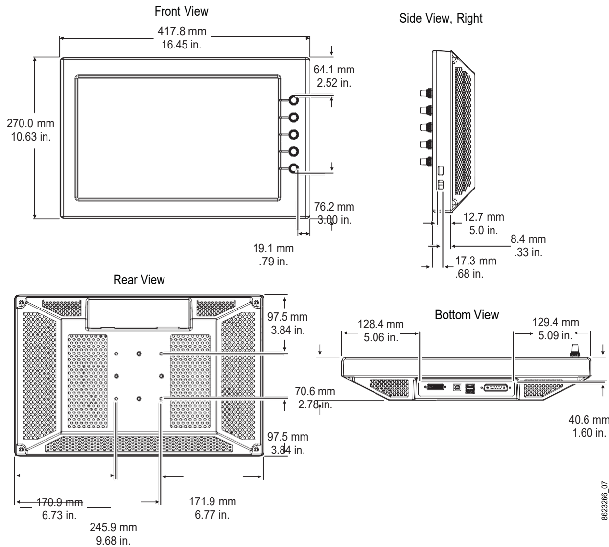
Menu Panel Dimensions
