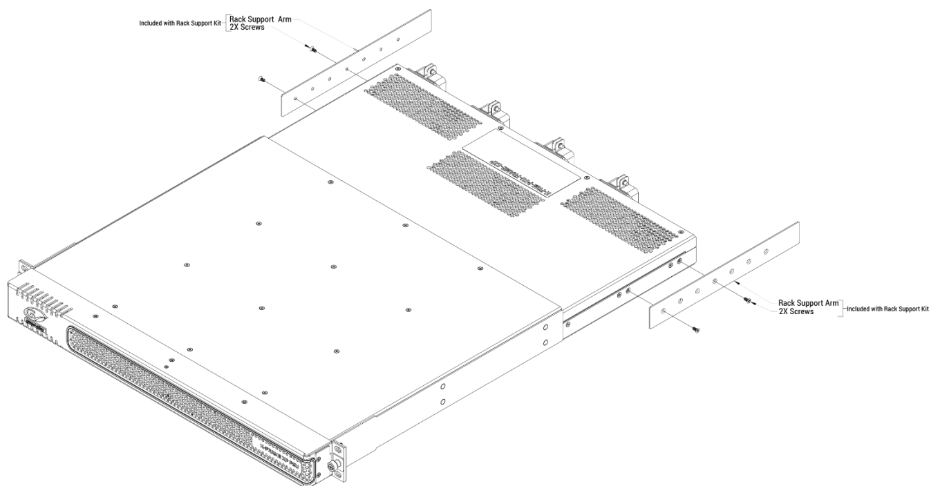
Power Supply Rack Installations and Cooling Airflow
