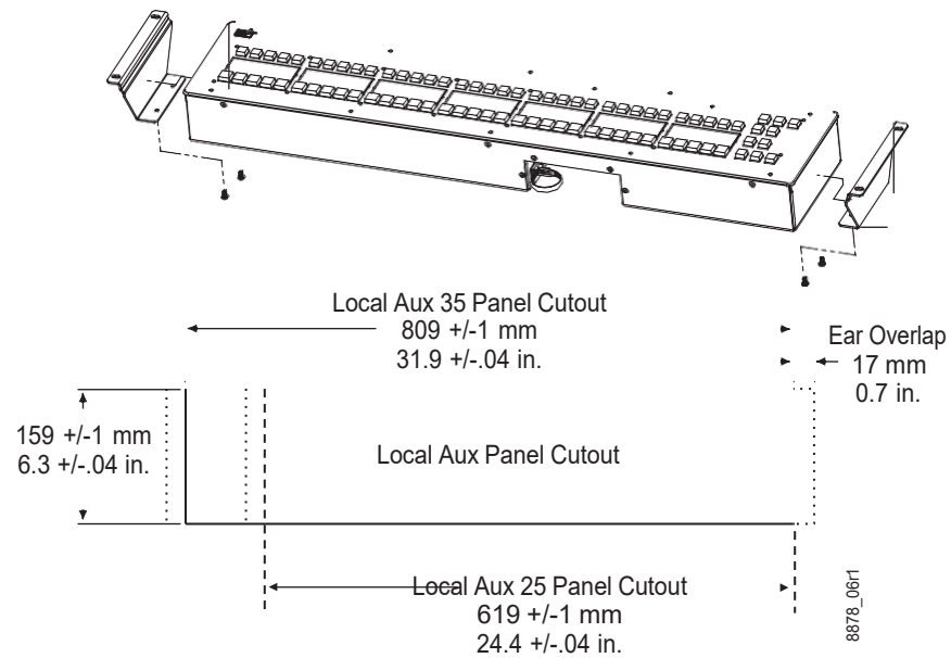
Local Aux Panel Cutout Dimensions
