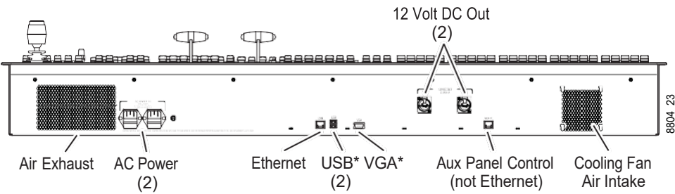
2-M/E Karrera Control Panel Rear Connections
