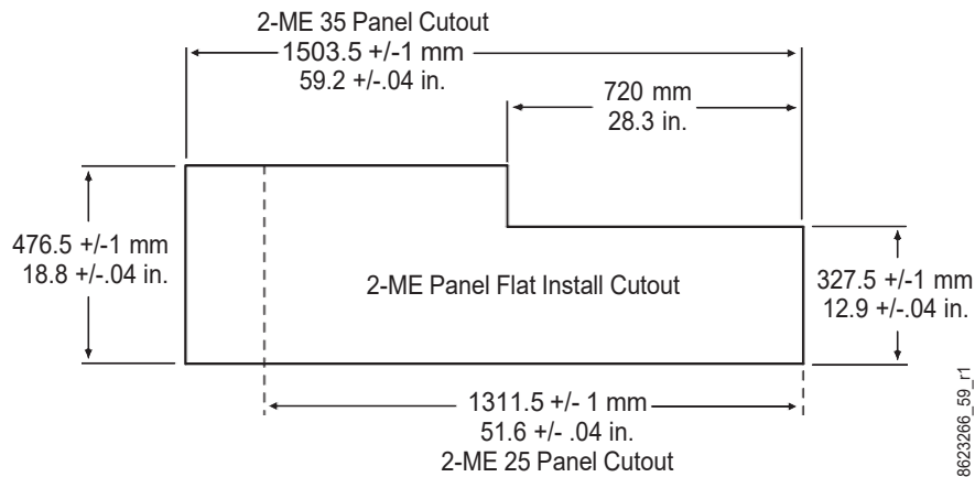
2-M/E Control Panel Cutout Dimensions, Flat Installation
