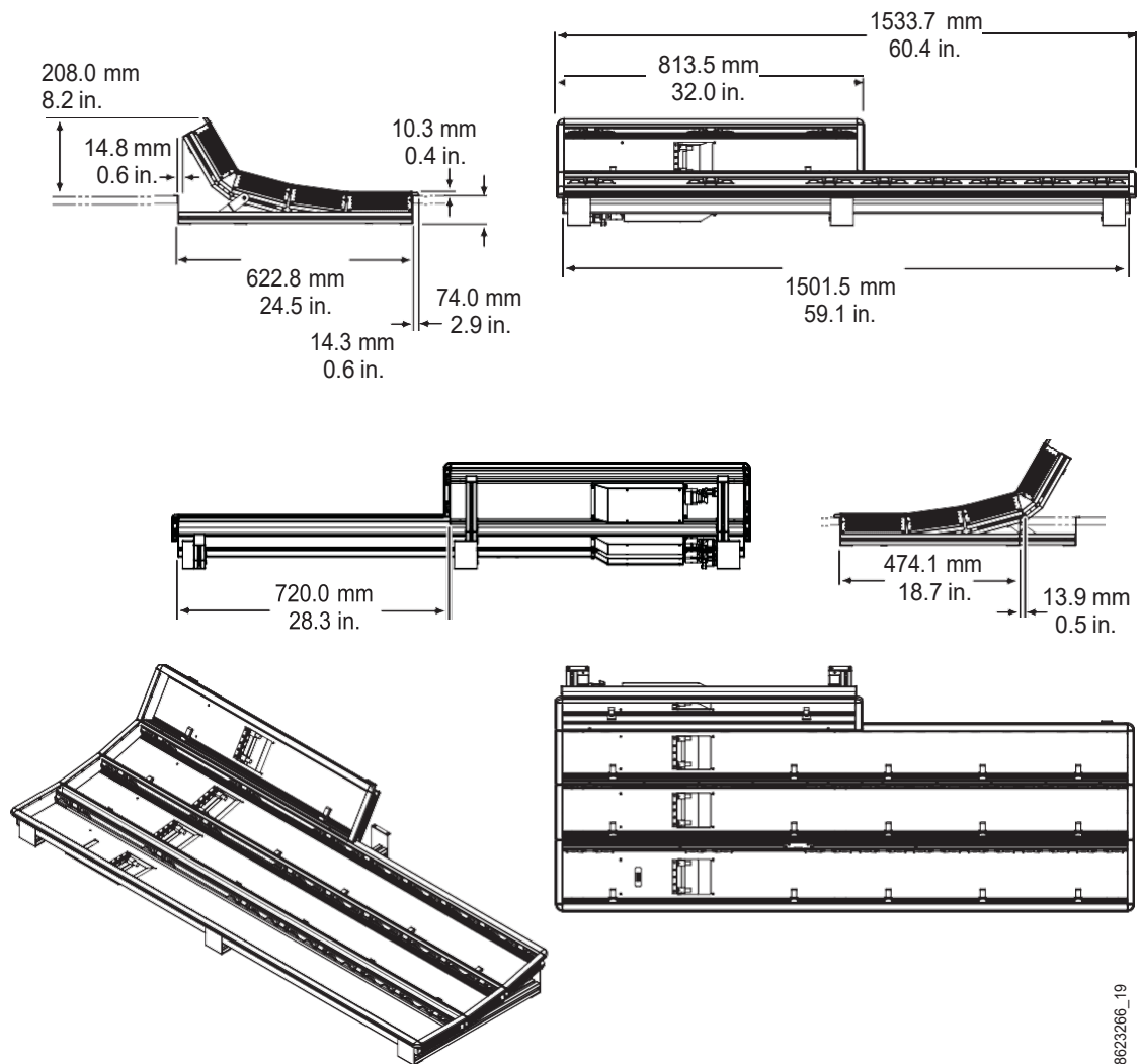
3-M/E 35 Control Panel Dimensions, Curved Installation
