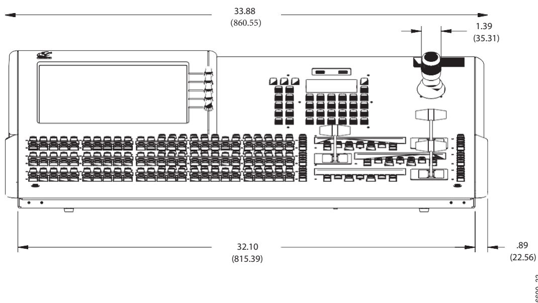
3-M/E GV Korona Control Panel Front Dimensions
