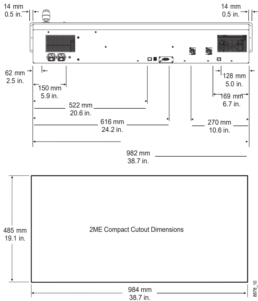
2-M/E Compact Karrera Control Panel Cutout Dimensions
