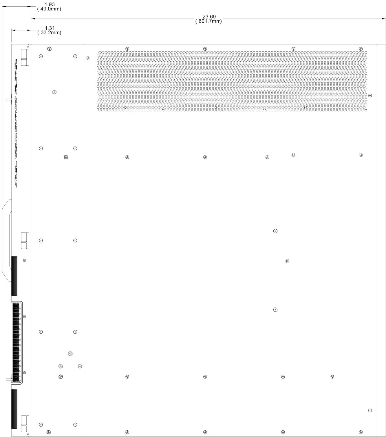
PowerSupplyFrameDimensions (TopView)
