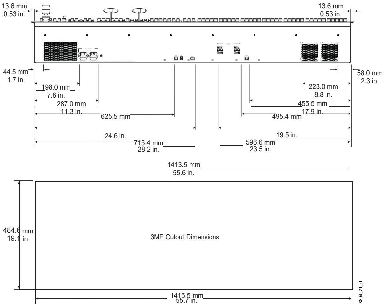
3-M/E Karrera Control Panel Cutout Dimensions
