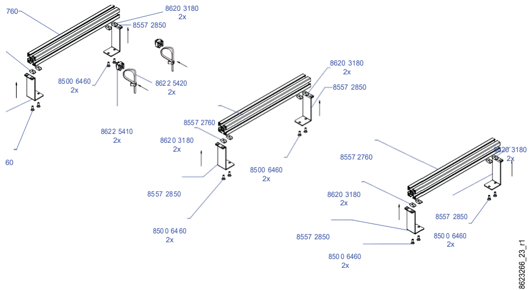
2-M/E Support Structure, Flat Installation, w/o Local Aux Stripe
