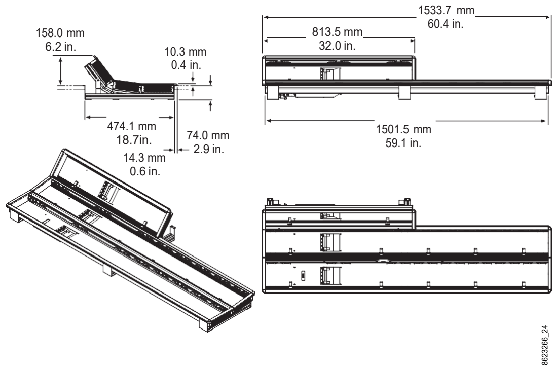
2-M/E 35 Control Panel Dimensions, Curved Installation
