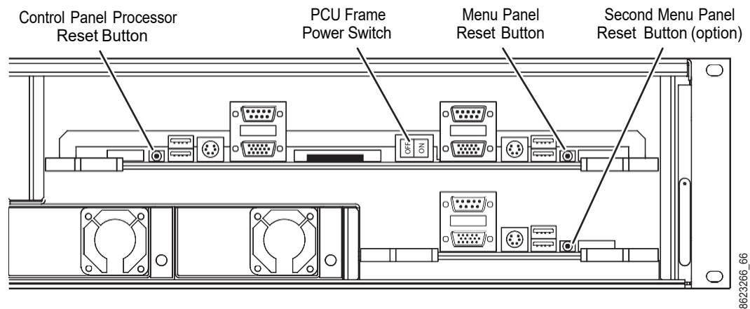
PCU Reset Buttons and Power Switch
