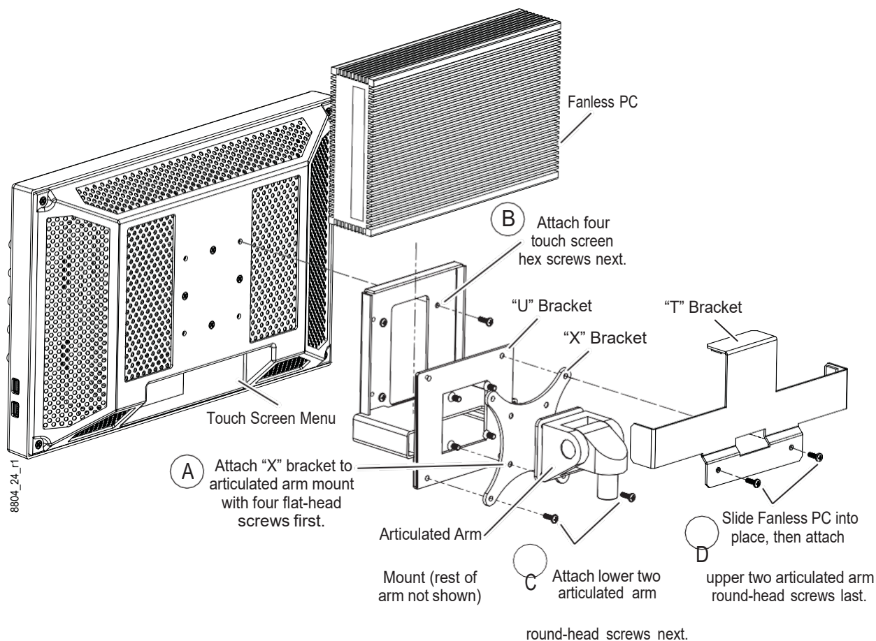
Fanless PC Mounting Bracket Assembly
