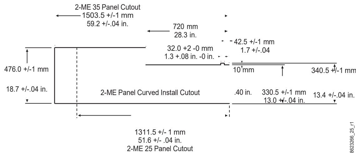
2-M/E Control Panel Cutout Dimensions, Curved Installation
