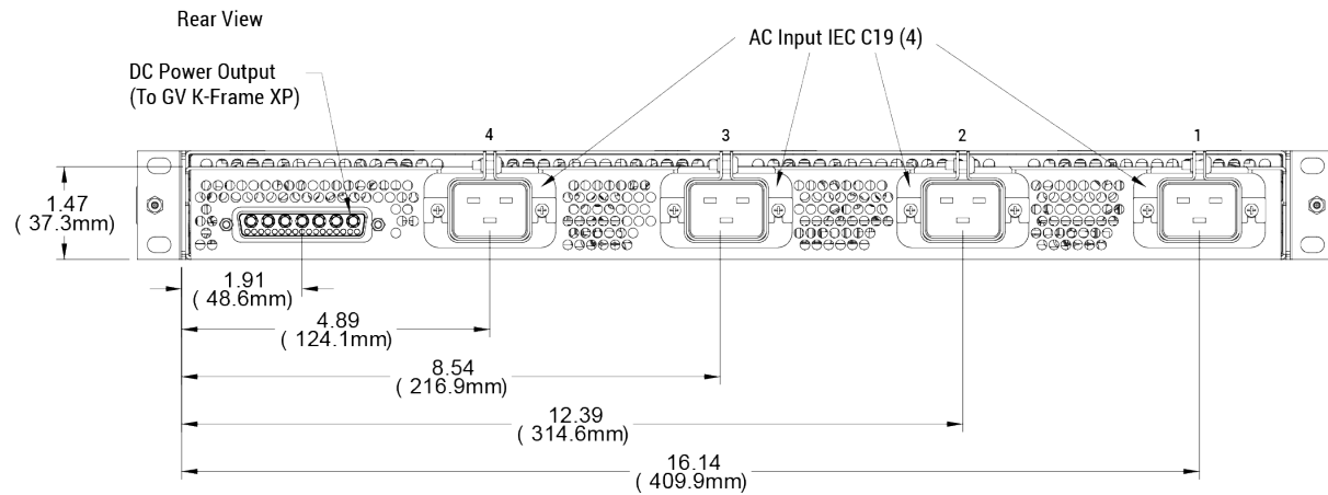
PowerSupplyFrameDimensions (Front and Rear Views)
