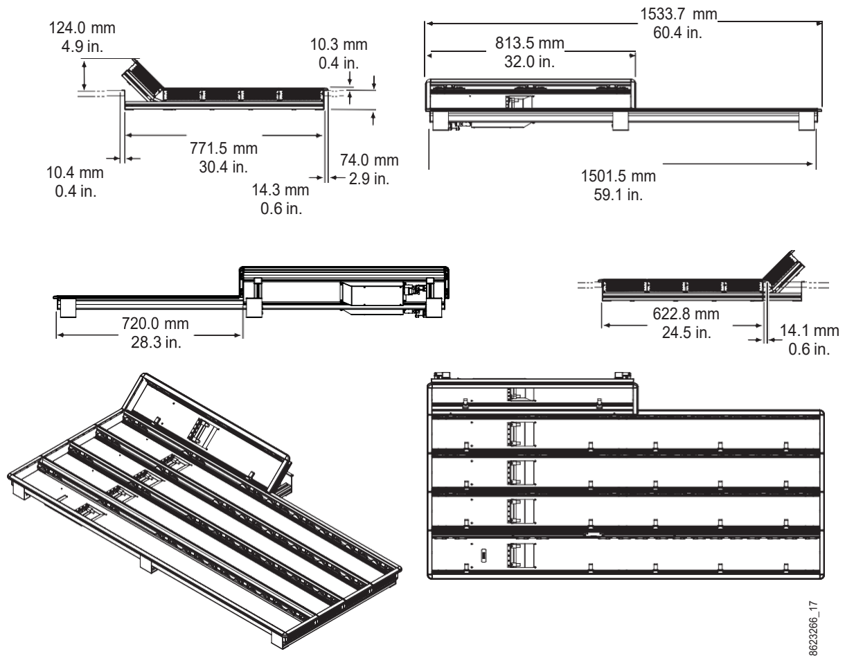
4-M/E 35 Control Panel Dimensions, Flat Installation
