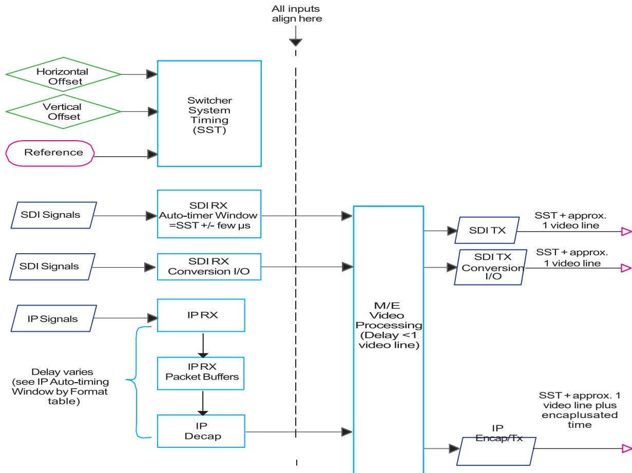
SDI/IP Switcher Signal Flow
