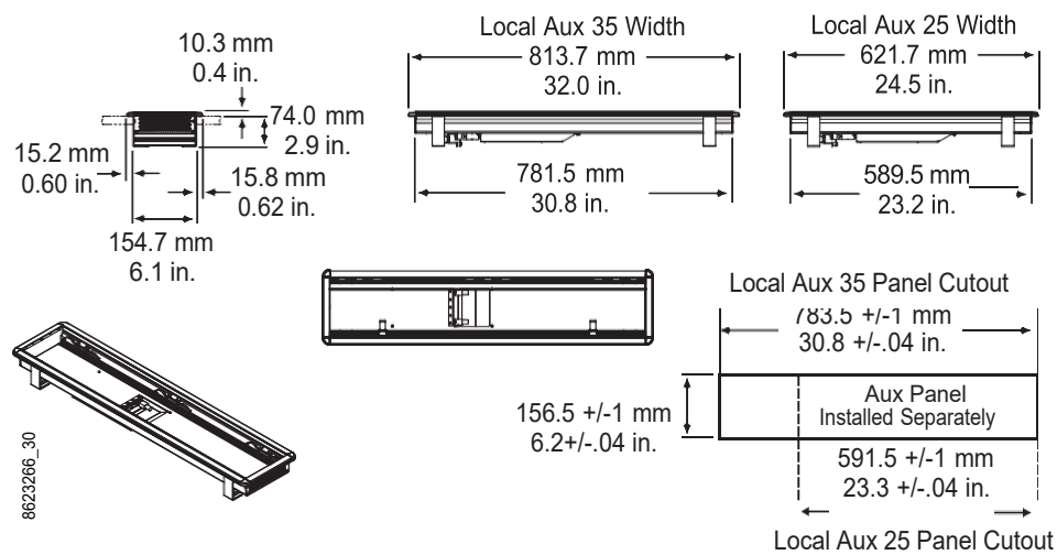
Local Aux Stripe Separate Installation Dimensions
