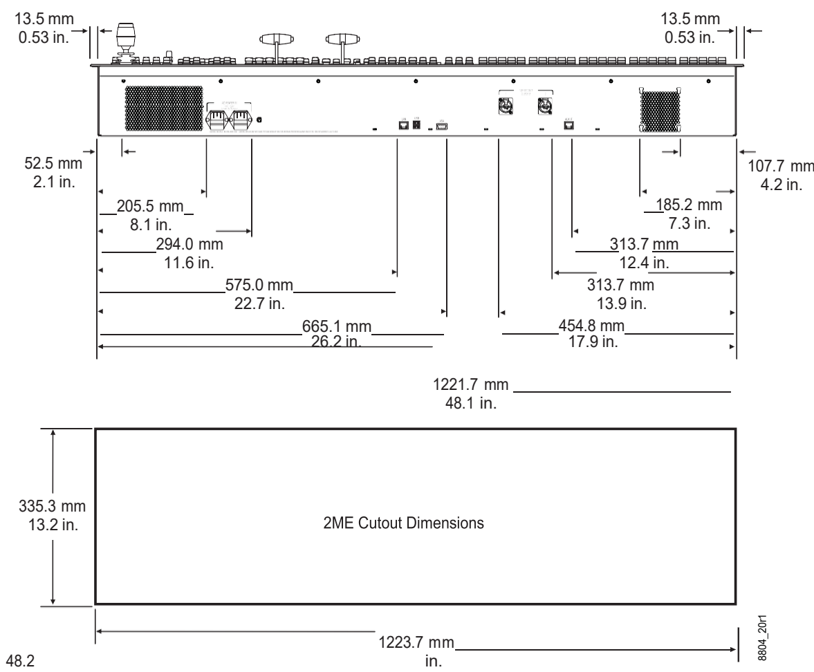
2-M/E Karrera Control Panel Cutout Dimensions
