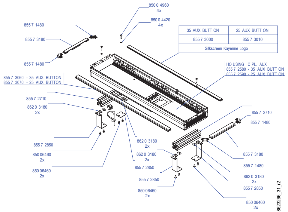
Local Aux Stripe Support Structure, Tray, and Trim
