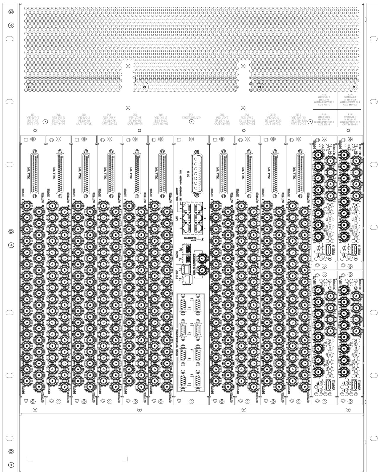
15-RU, Rear View IP/Gearbox/Conversion
