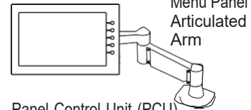
Menu Panel
