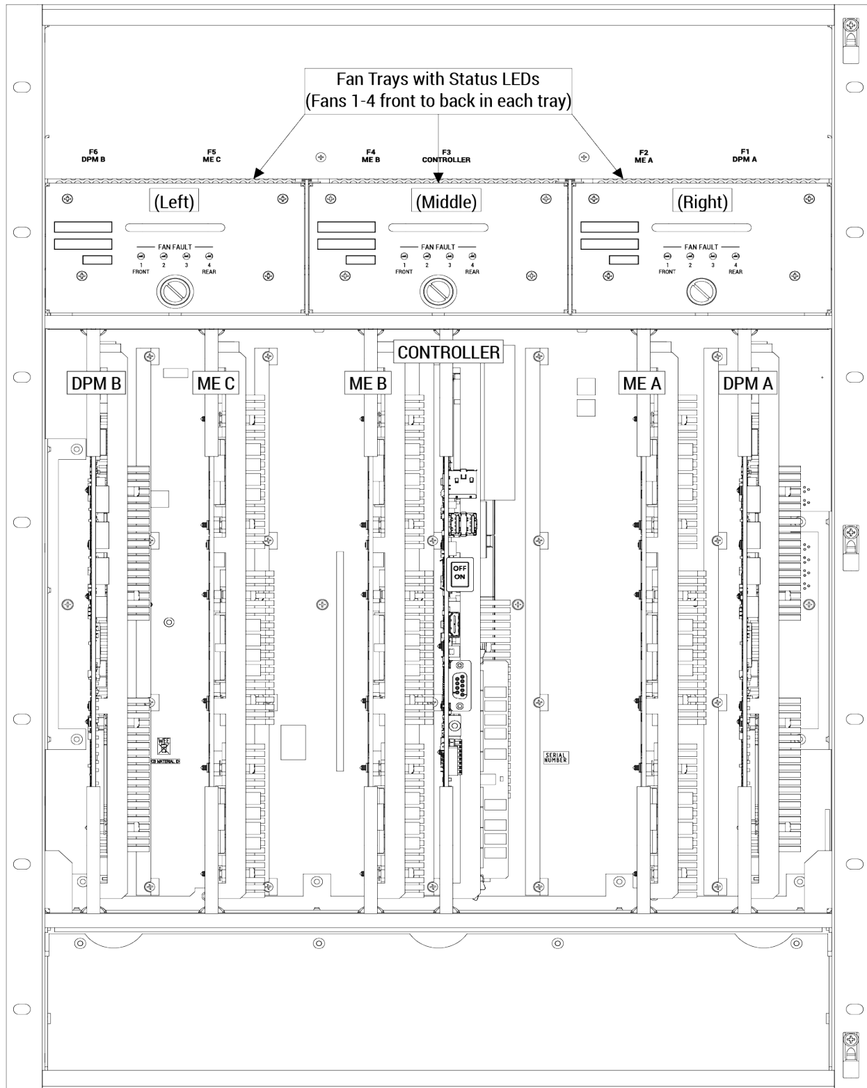
15-RU, Front View with Door Removed
