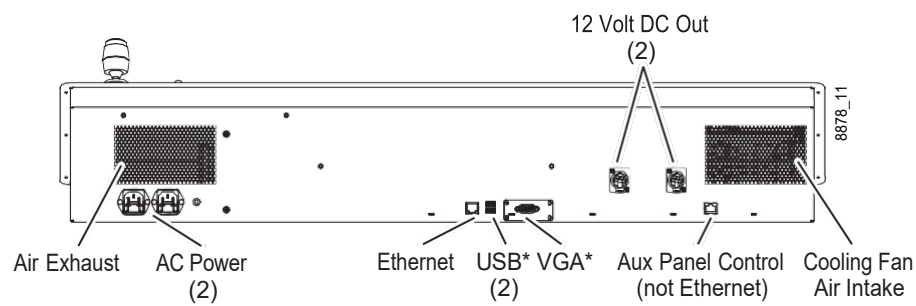
2-M/E Compact Karrera Control Panel Rear Connections
