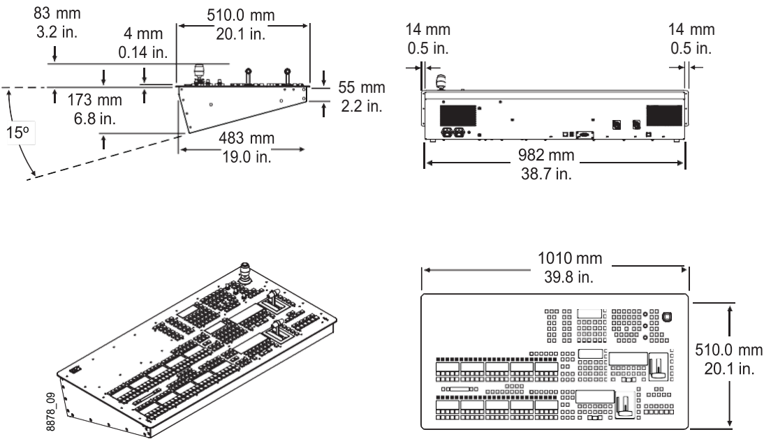
2-M/E Compact Karrera Control Panel Dimensions
