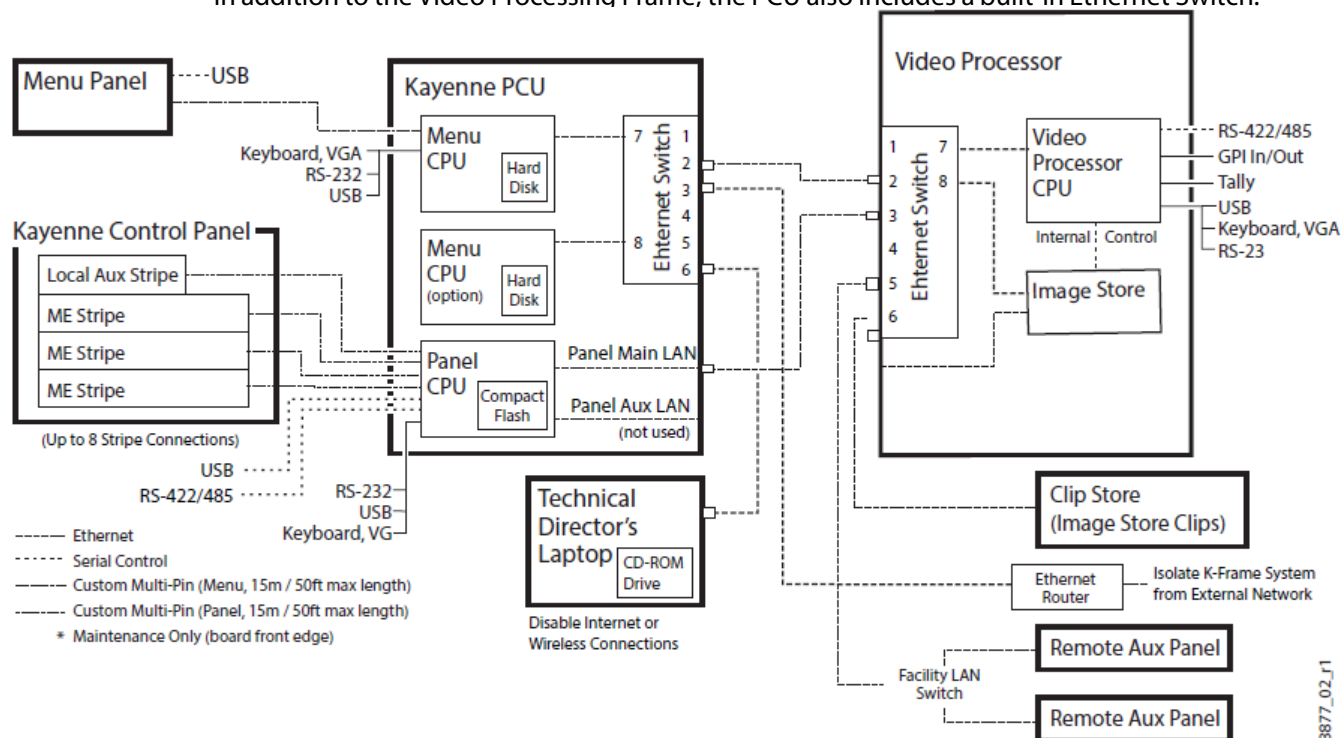
Kayenne GV K-Frame XP System Communications Overview
