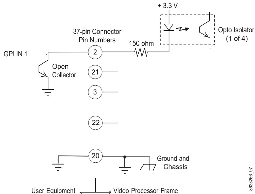
GPI Input Connections (Typical 1 of 4 Connections)
