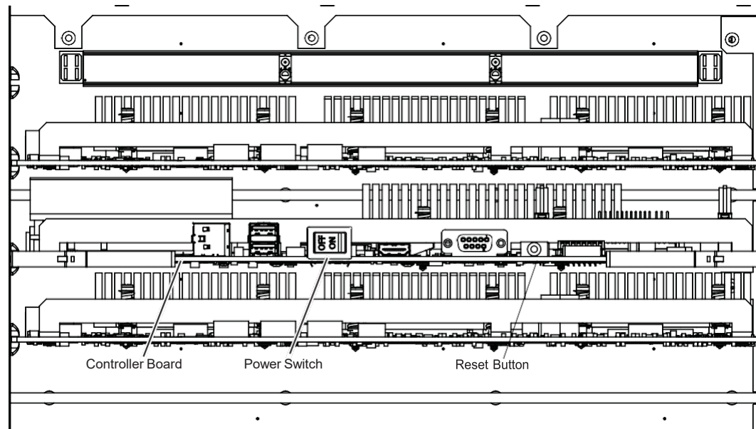
6-RU Video Processor Frame Reset Button and Power Switch
