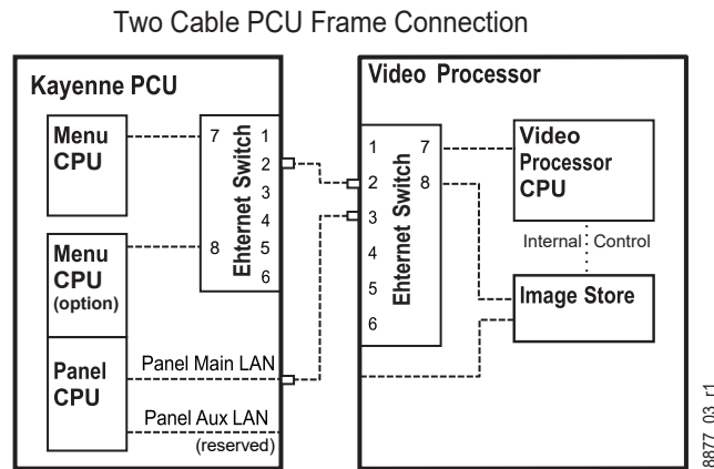
PCU to Kayenne GV K-Frame XP Network Connection Methods
