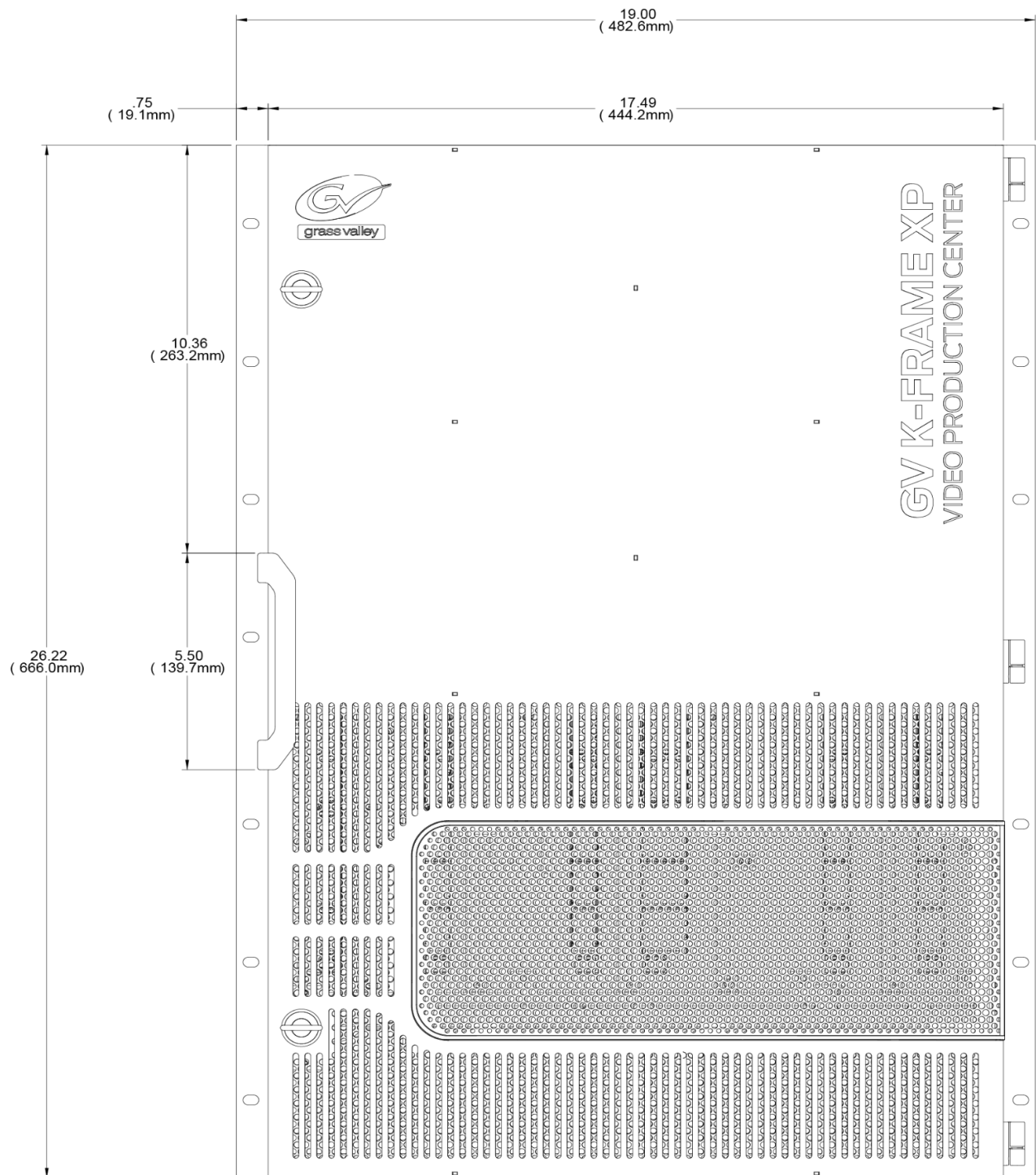
15-RU Dimensions (Front View)
