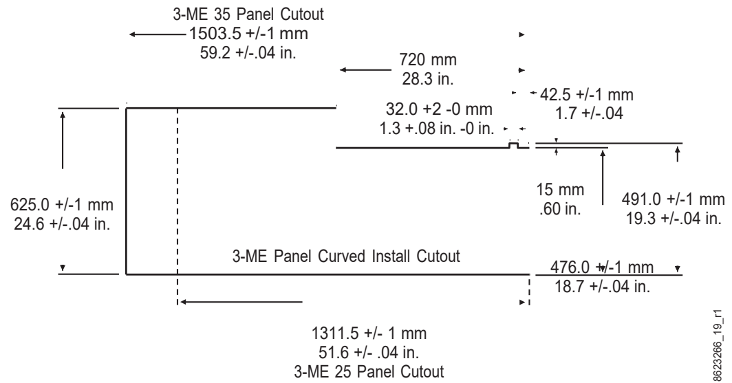
3-M/E Control Panel Cutout Dimensions, Curved Installation
