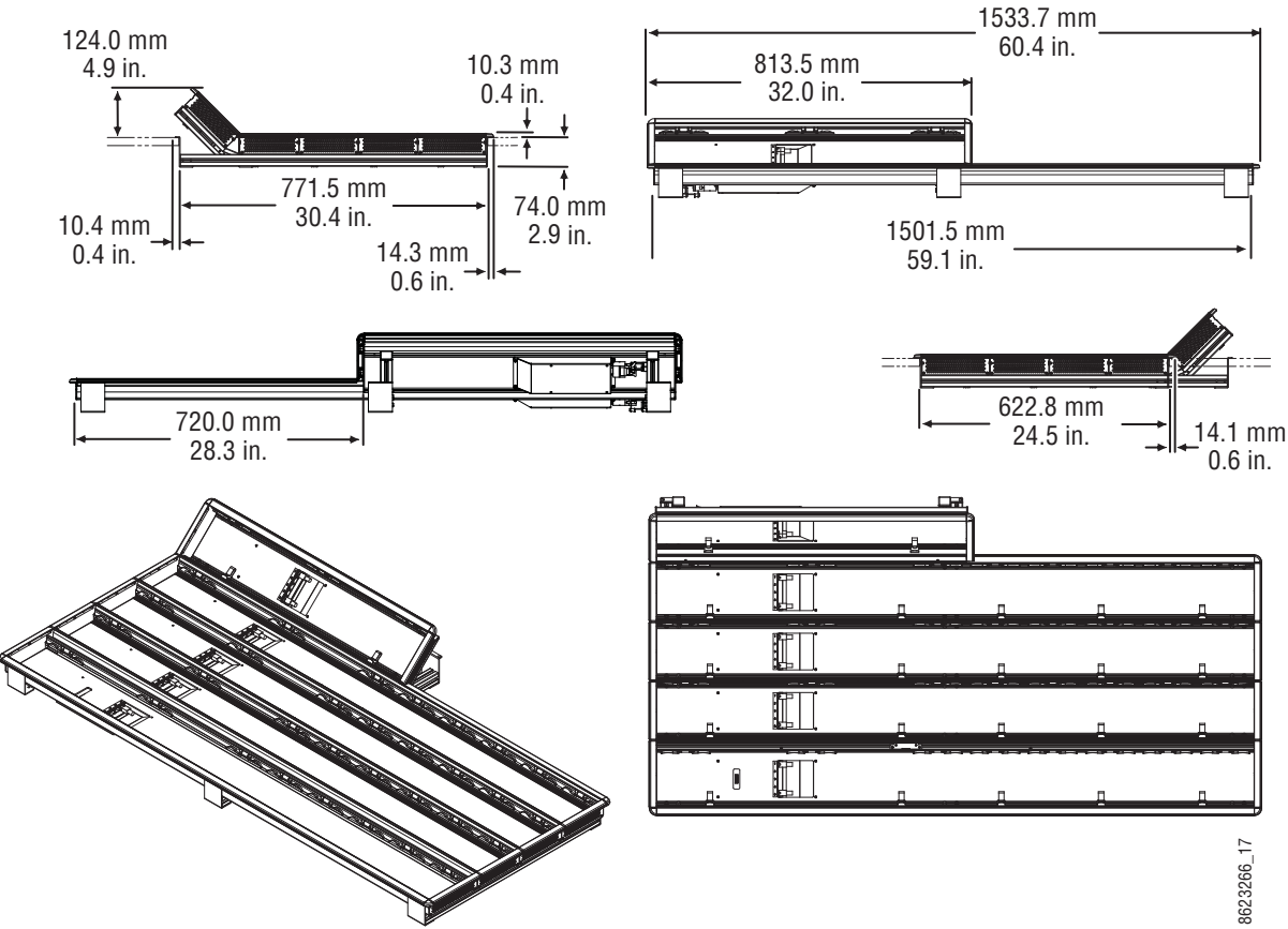
Figure 15. 4-ME 35 Control Panel Dimensions, Flat Installation
