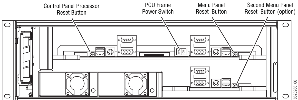
Figure 155. PCU Reset Buttons and Power Switch
