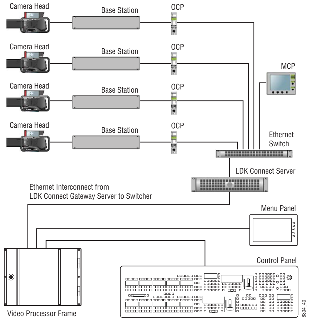
Figure 114. Kayenne System Interconnection with Camera Gateway
