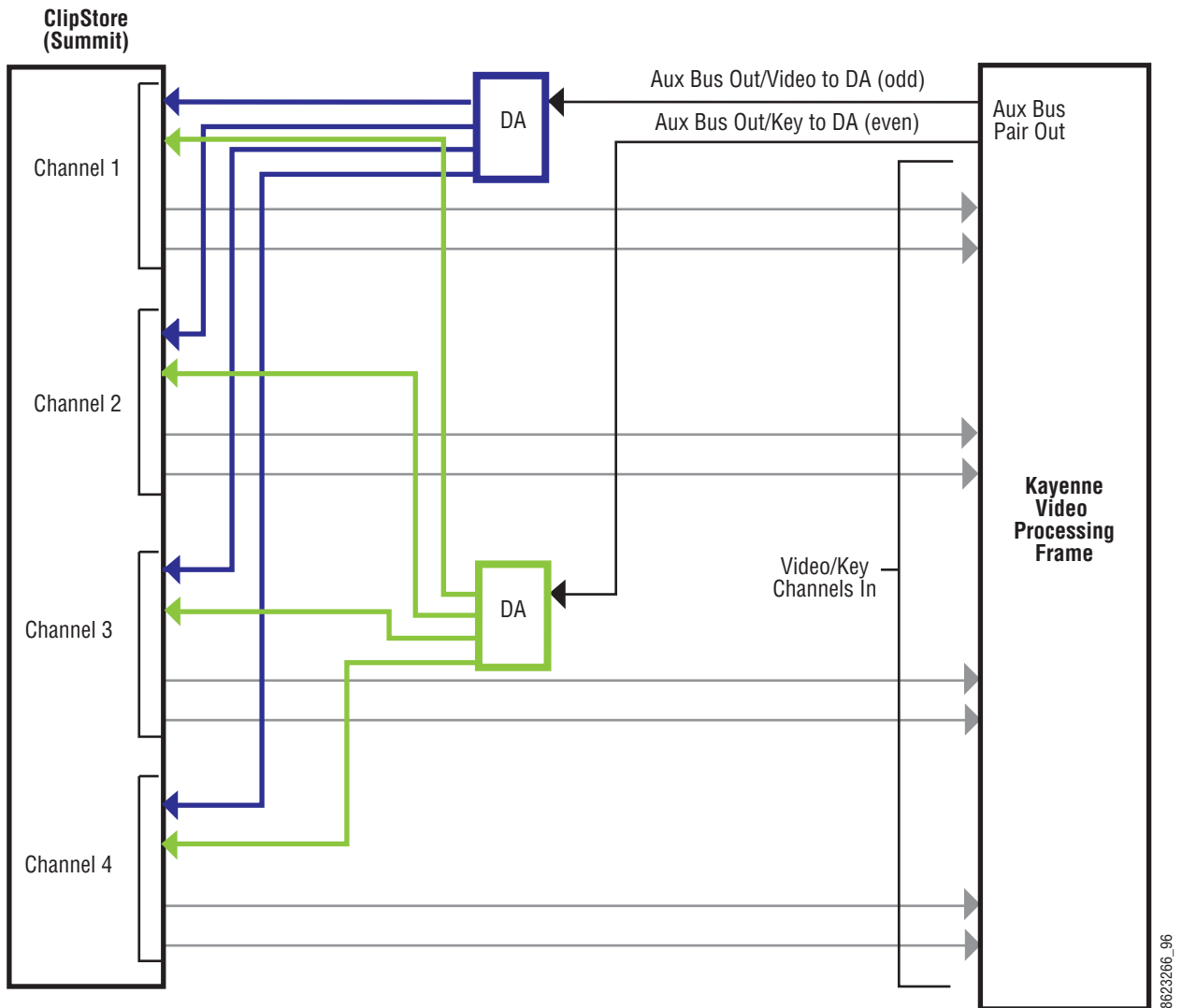
Figure 70. ClipStore Connection Using Distribution Amplifiers
