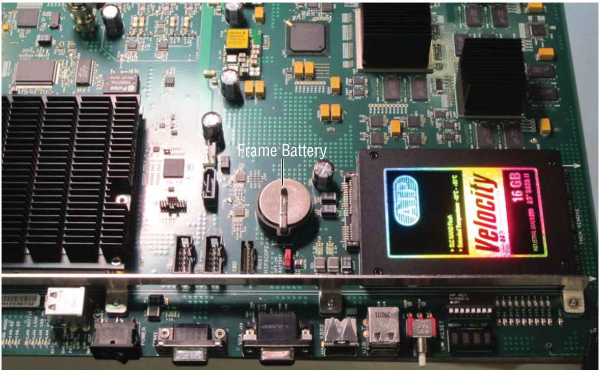
Figure 172. Video Processor Frame Controller Board with Battery Indicated
