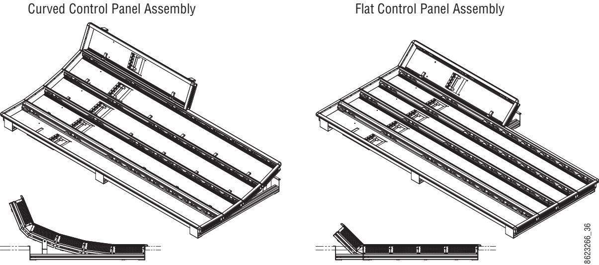
Figure 6. Curved and Flat Control Surface Installations
