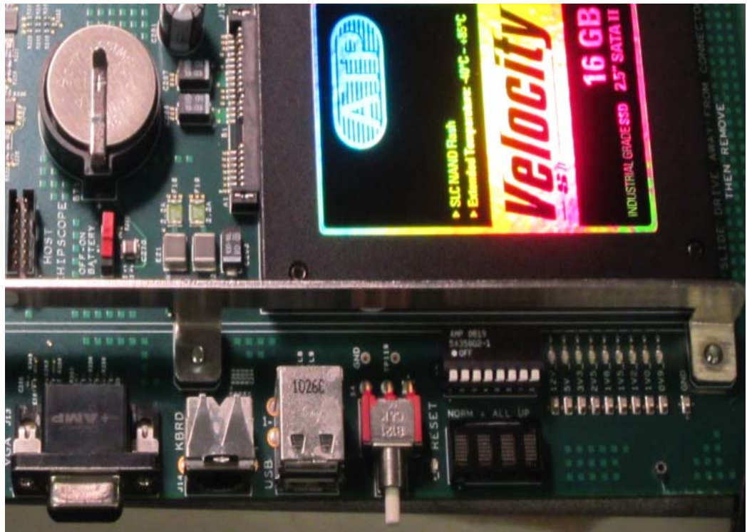
Figure 171. K-Frame Control Processor Board - S2 Boot Mode Dipswitch Location
