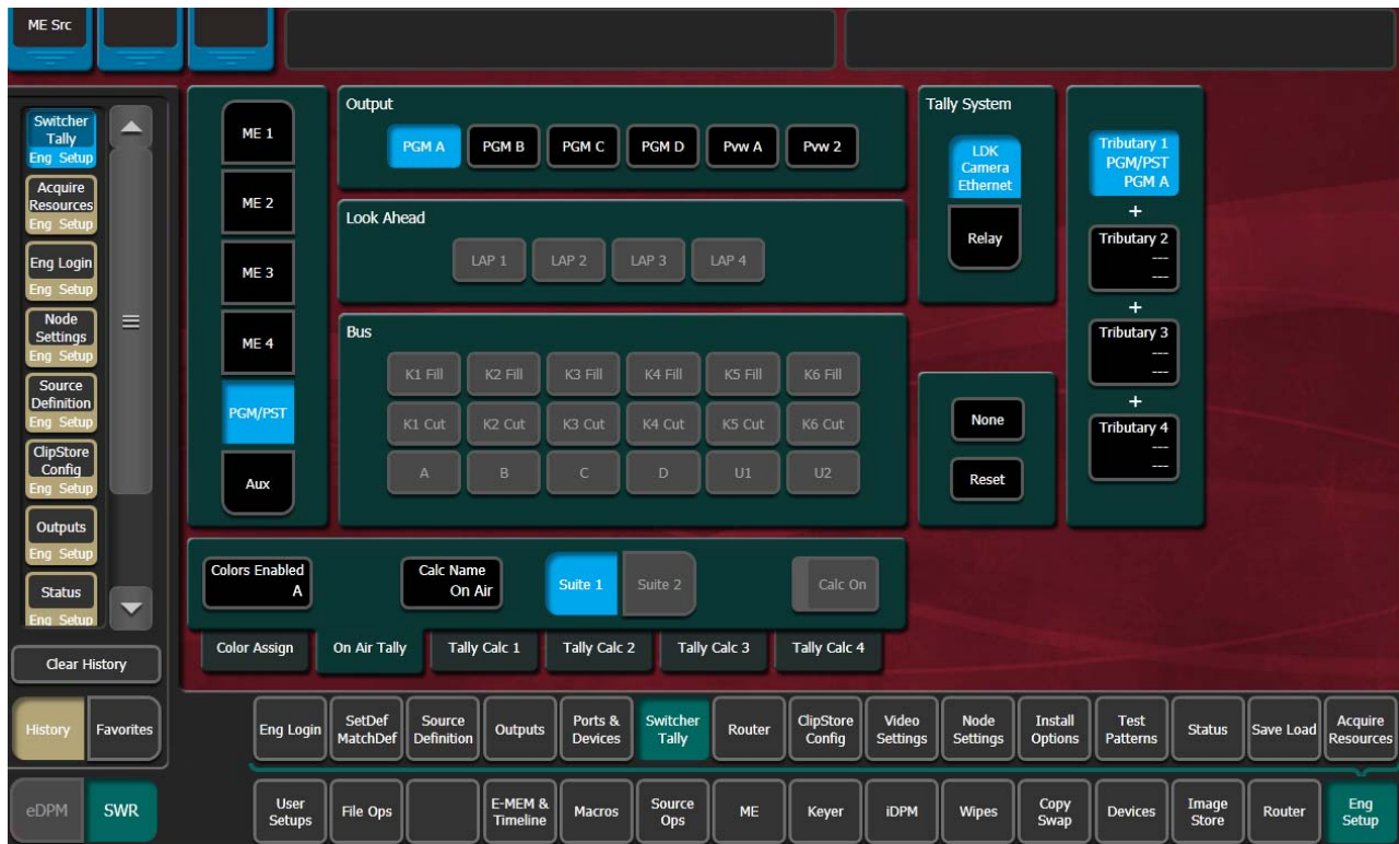
Figure 119. Switcher Tally LDK Camera Ethernet Menu
