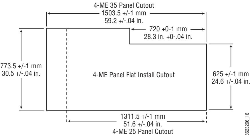
Figure 16. 4-ME Control Panel Cutout Dimensions, Flat Installation
