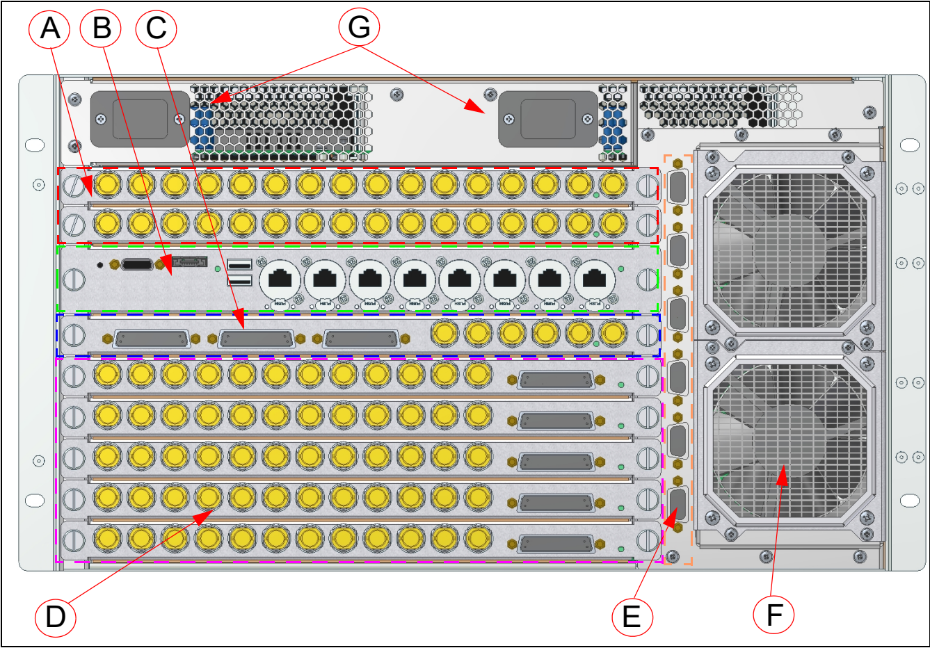
6RU Mainframe Rear Fin Locations and Connectors
