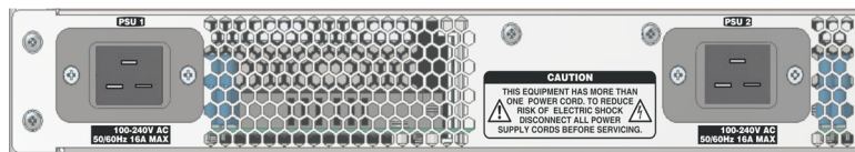
Mains Inputs to the Kahuna 6400 - 6RU Mainframe
