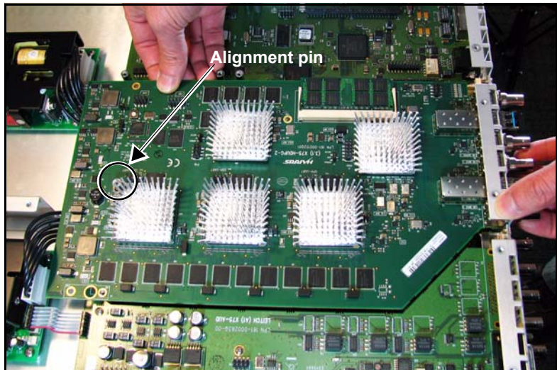
Figure C-17. Positioning the X85 Module
