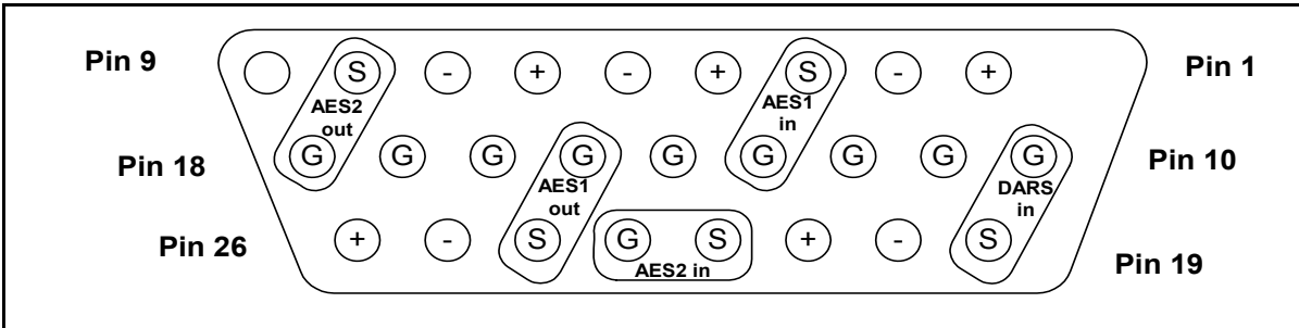
Figure A-6. X75OPTCAB-8-C Connector Pinout
