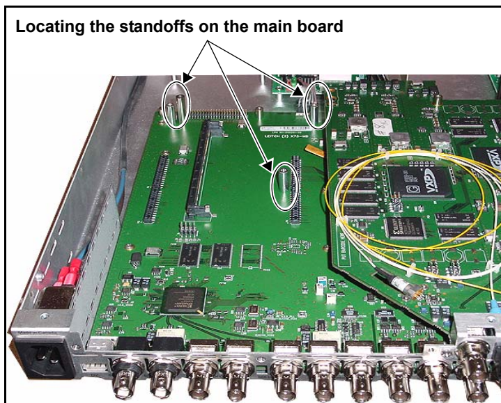
Figure C-5. Locating Main Board Standoffs
