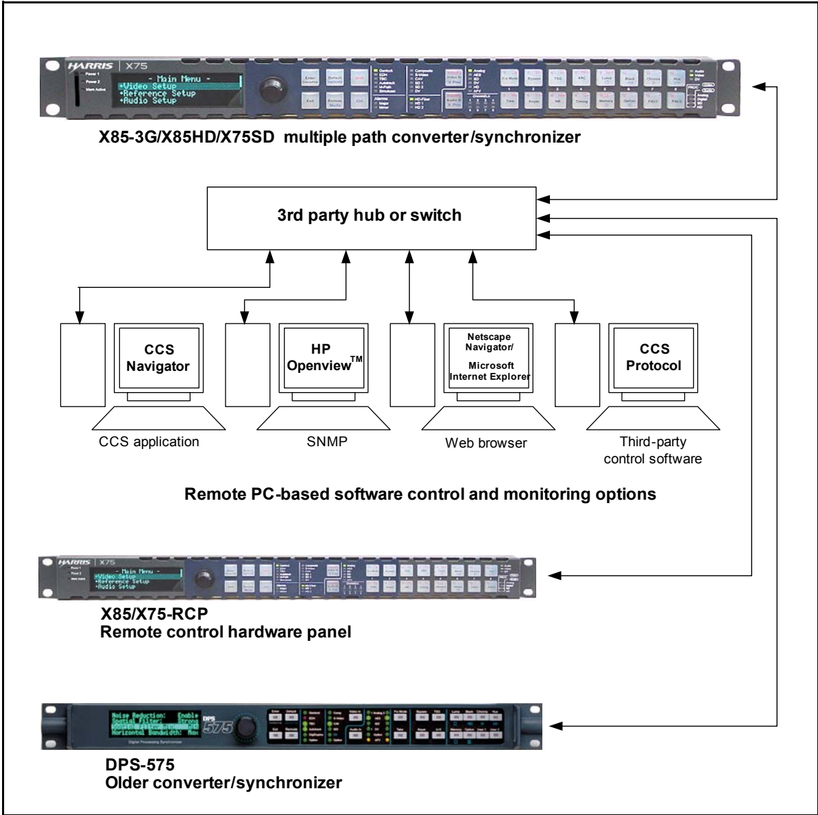
Figure 7-4. Network Configuration Diagram
