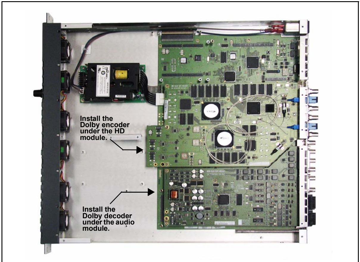
Figure C-33. Location of Dolby Decoder and Encoder (X75OPT-HDUPG HD Module Shown)
