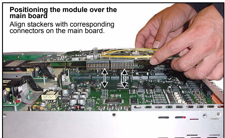
Figure C-12. Positioning Module over Standoffs
