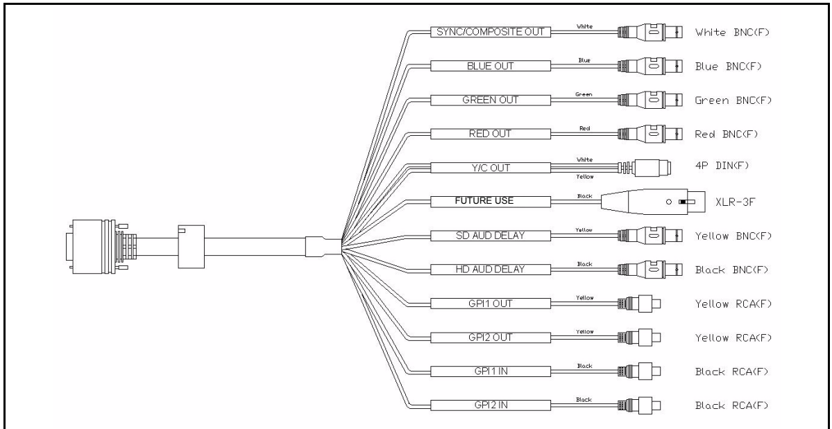
Figure A-2. X75OPTCAB-MULTI Cable Connectors
