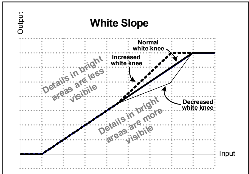
Figure 8-25. Examples of Increased and Decreased White Slope
