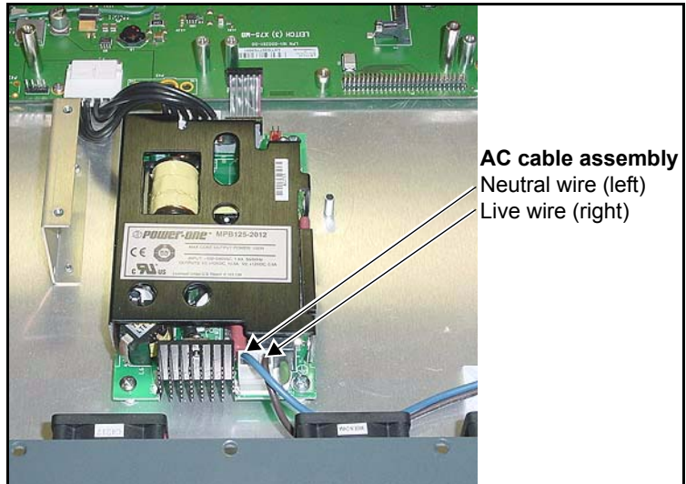
Figure C-48. Connecting AC Cables to Power Supply
