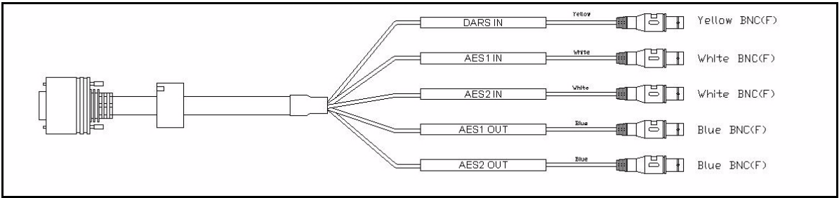
Figure A-5. X75OPTCAB-8-C Cable Connectors
