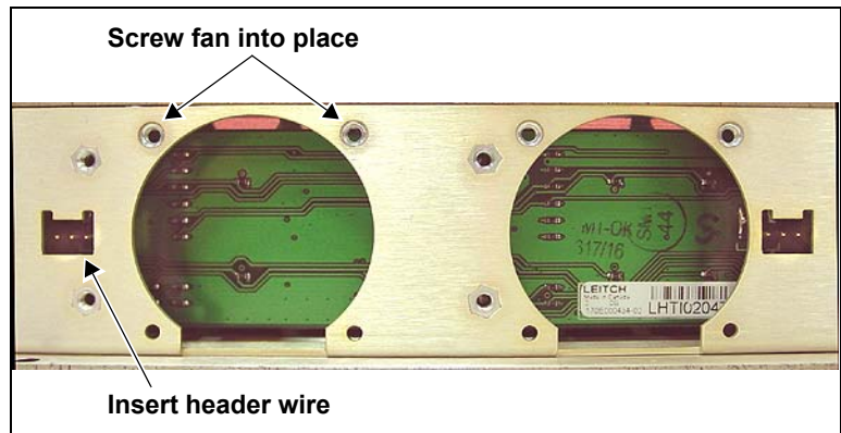
Figure C-56. Replacing a Fan within the Assembly
