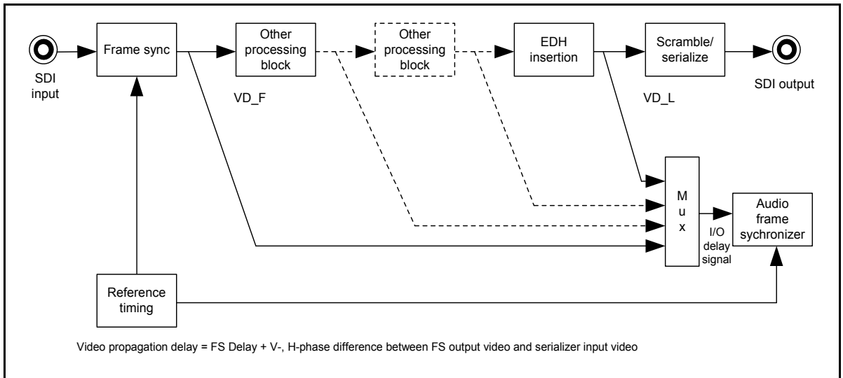
Figure B-7. I/O Delay Signal
