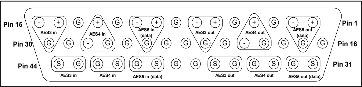
Figure A-12. CAB-X75HD-COMBO Connector Pinout
