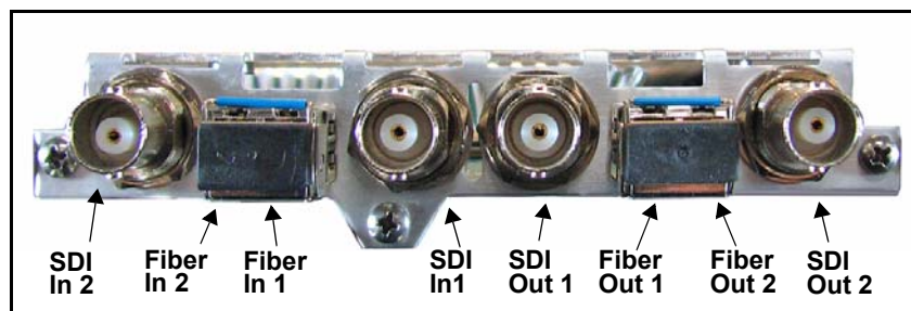
Figure 1-11. X85 Back Panel
