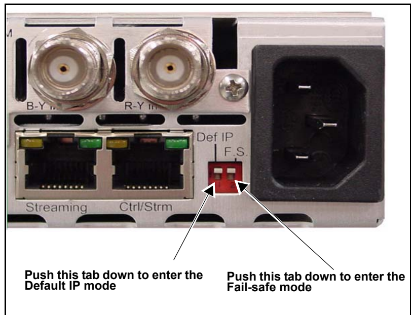
Figure B-10. Location of Def IP and FS DIP Switches
