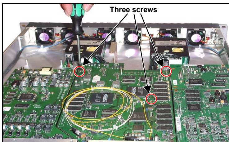
Figure C-38. Removing HDTV Board Mounting Screws
