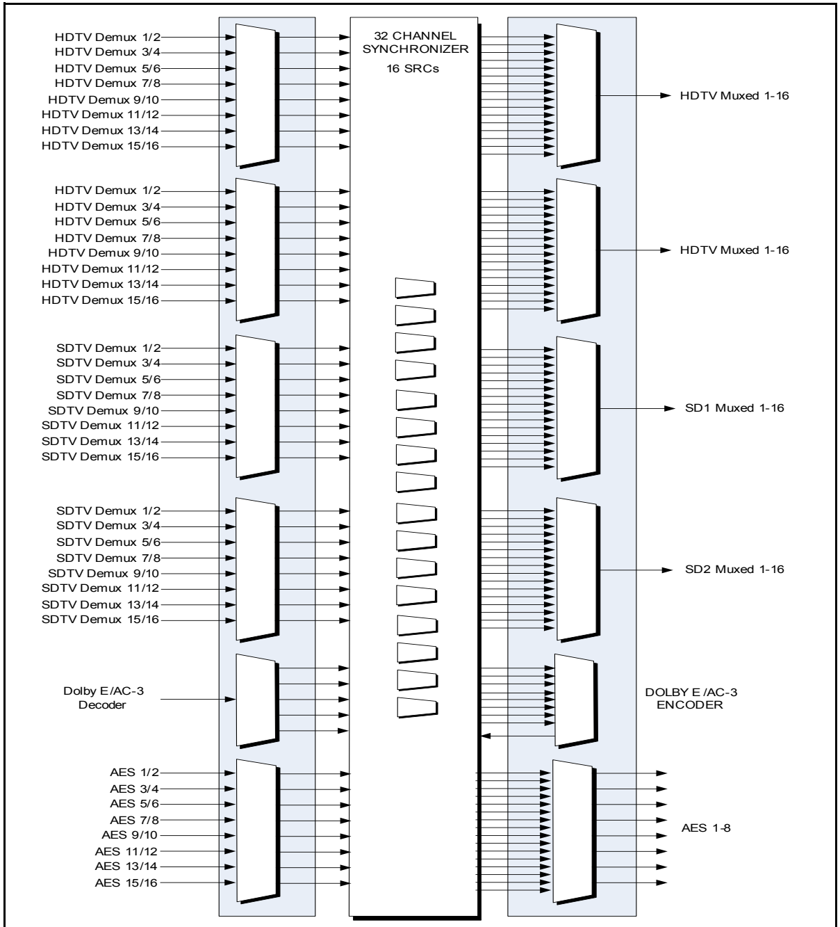
Figure 2-11. 32-Channel 3 Gb/s Audio Functional Block Diagram
