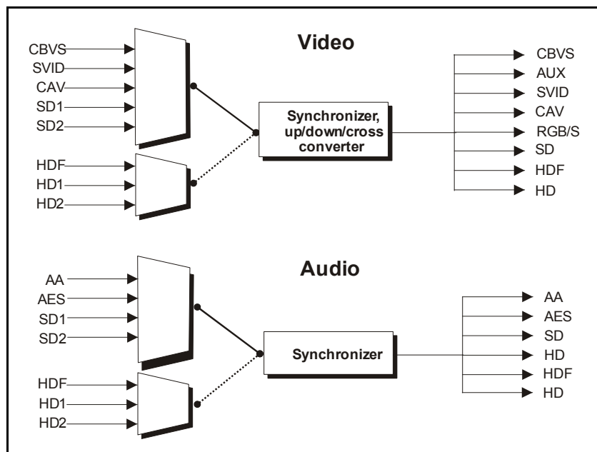
Figure 2-12. X75 Simulcast Processing
