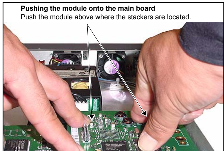
Figure C-29. Pushing the Module on to the Main Board
