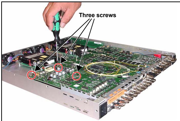
Figure C-37. Removing Audio Board Mounting Screws
