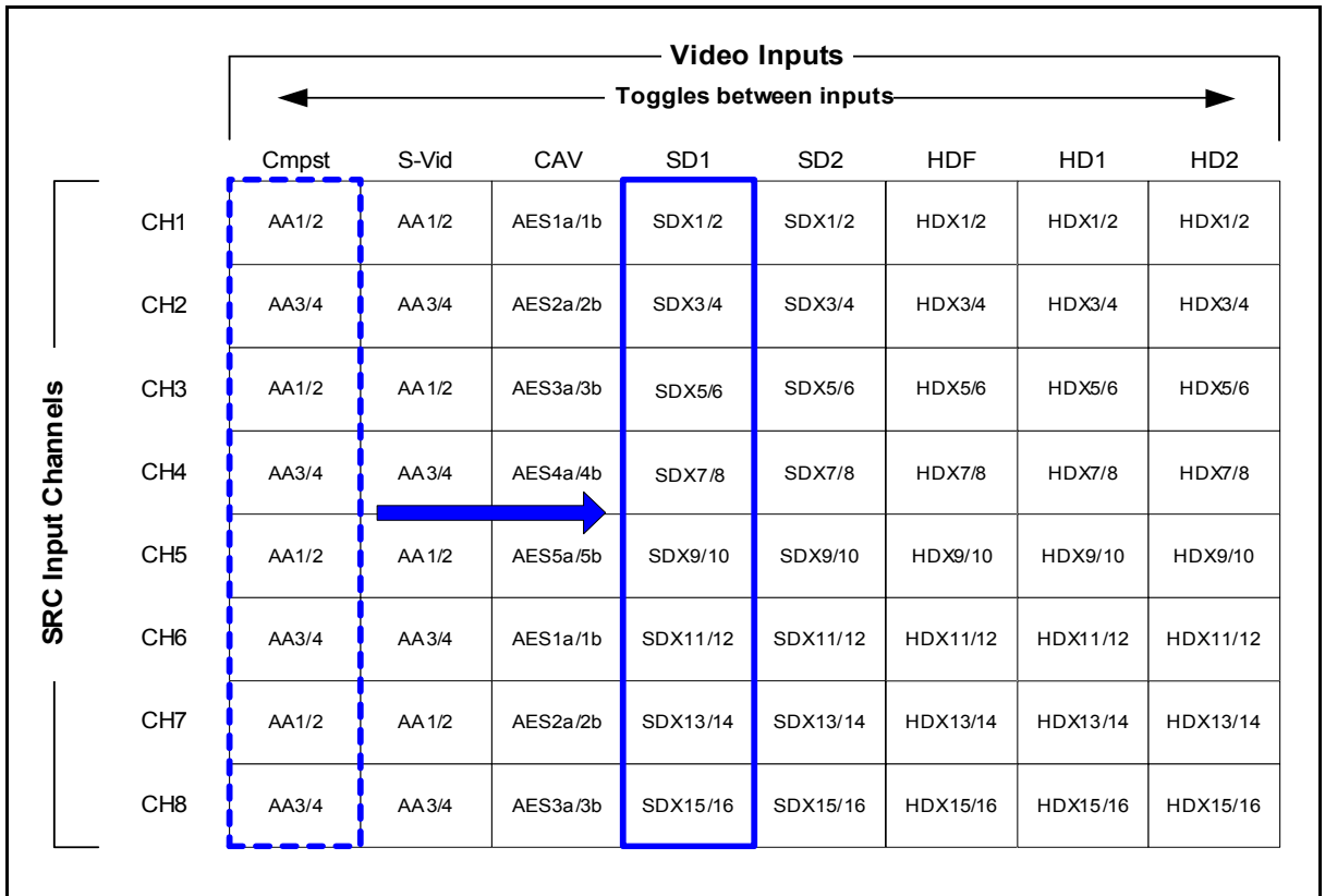
Figure 9-3. X75 Default AFV Channel Assignment
