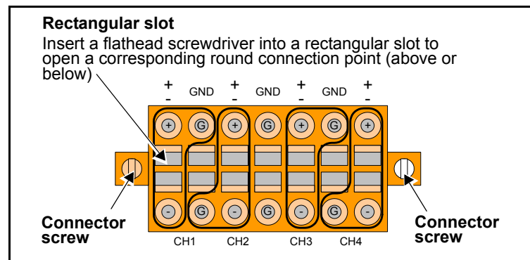
Figure 1-4. Installing Analog Audio Receptacles
