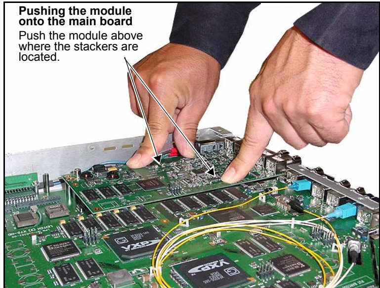
Figure C-27. Pushing the Module on to the Main Board (X75 Shown)
