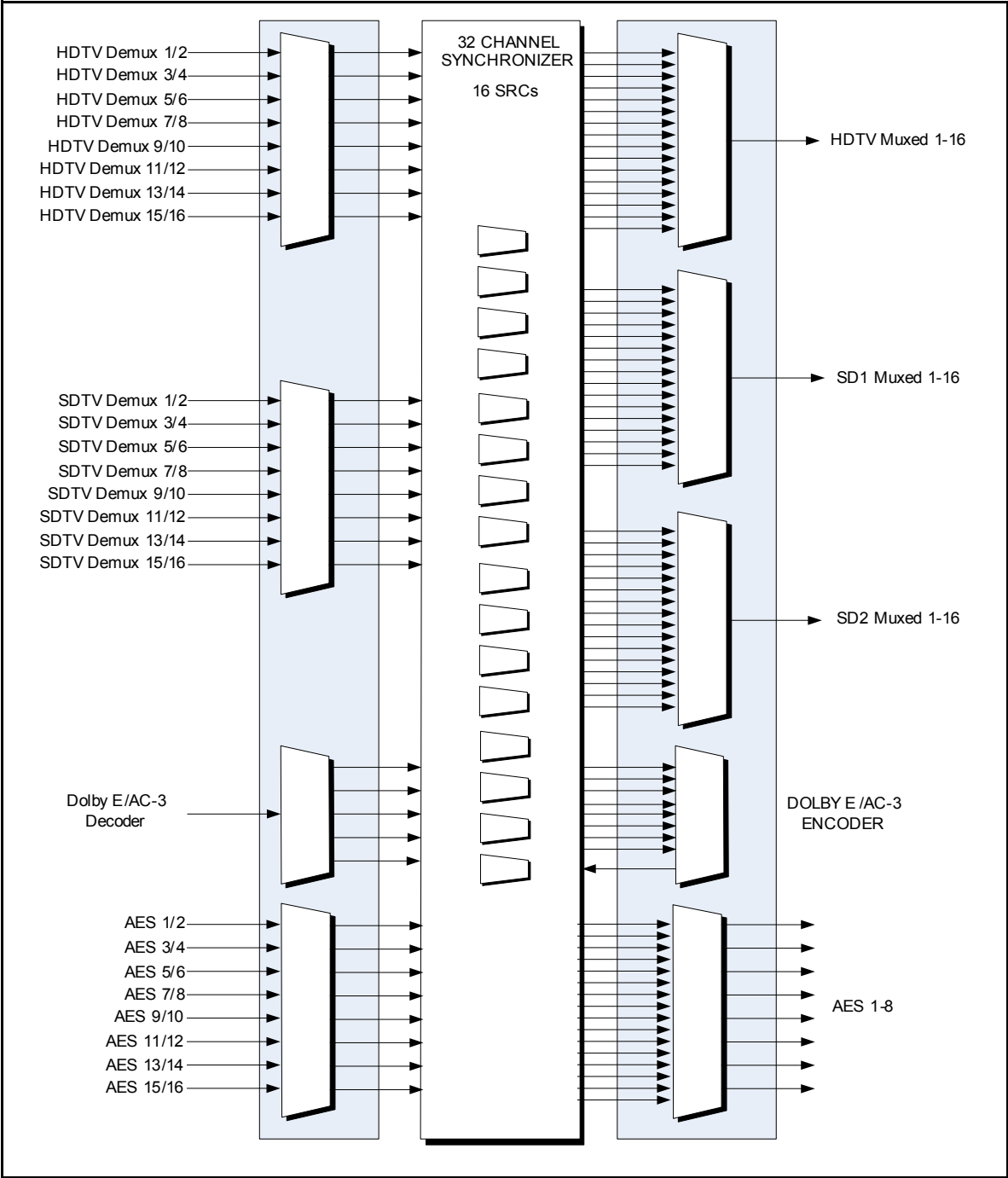
Figure 2-10. 32-Channel Audio Functional Block Diagram
