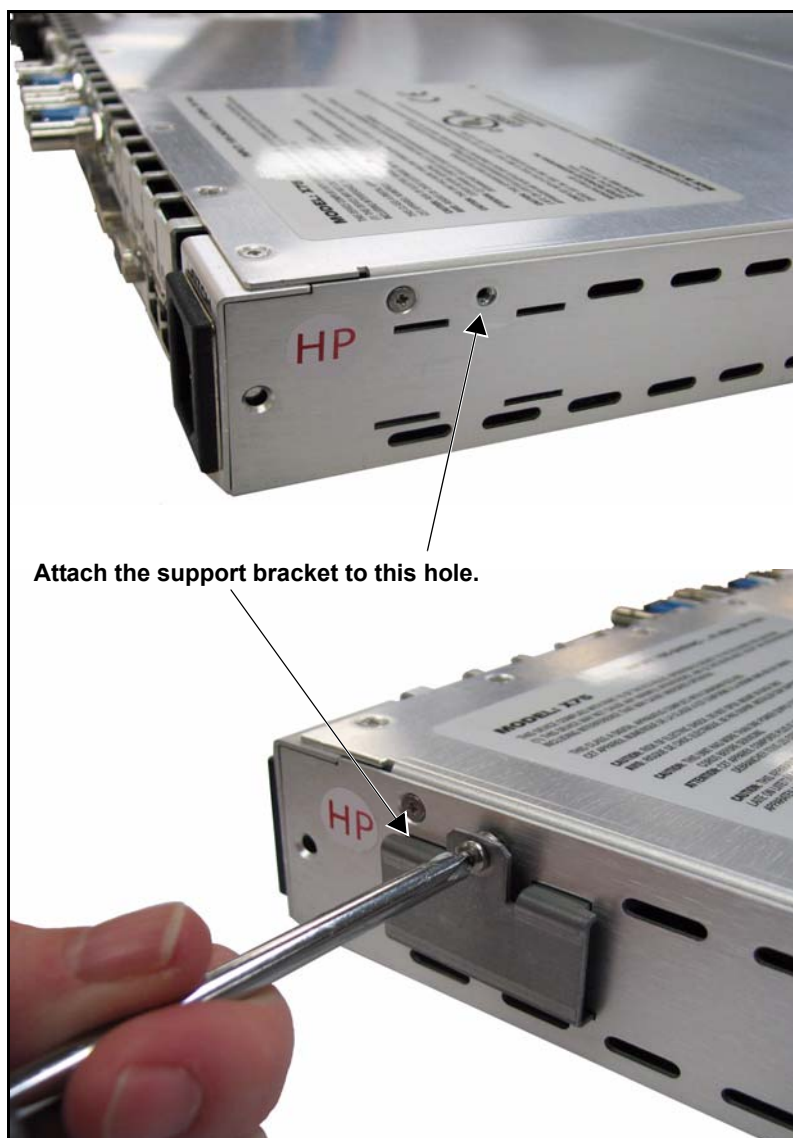
Figure 4-2. Bracket Installation
