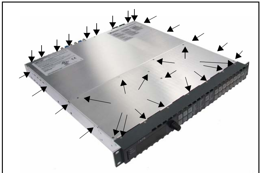
Figure C-2. Location of Chassis Cover Screws
