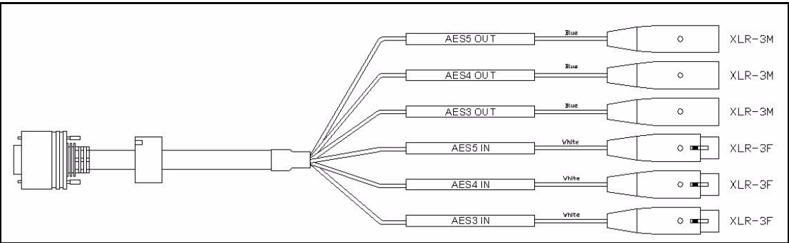
Figure A-15. X75OPTCAB-XLR Cable Connectors
