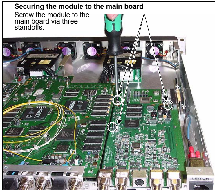
Figure C-28. Securing the Module to the Main Board
