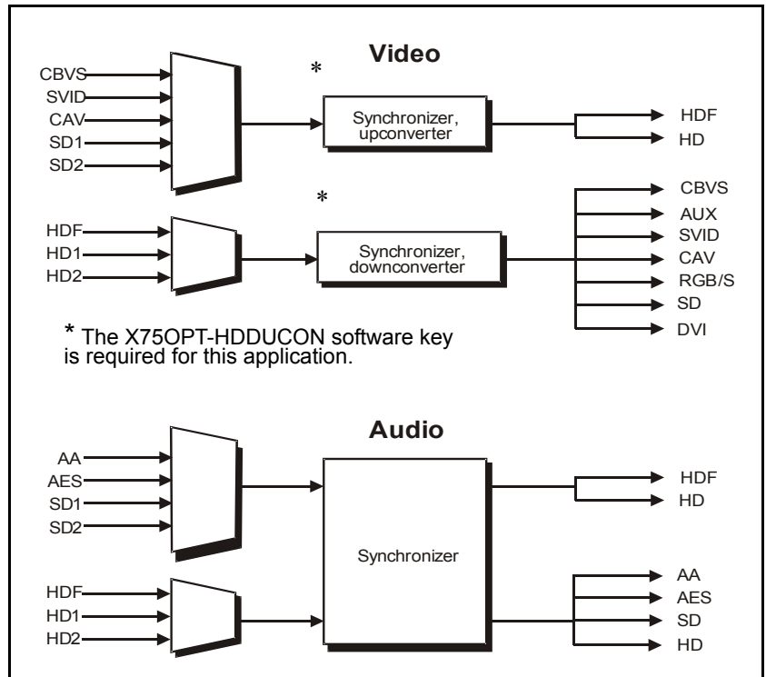
Figure 2-7. X75 M-Path (Dual Source Video and Audio) Processing
