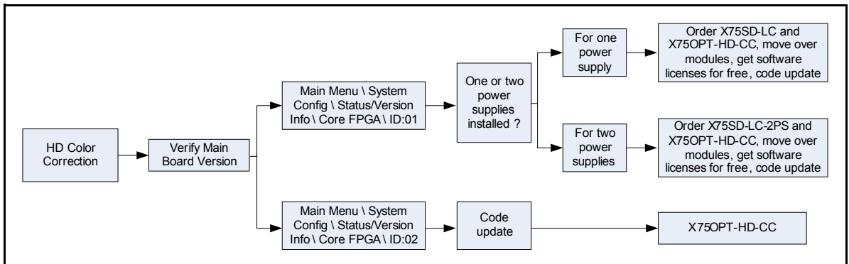
Figure 8-24. HD-SDI Color Correction Requirements
