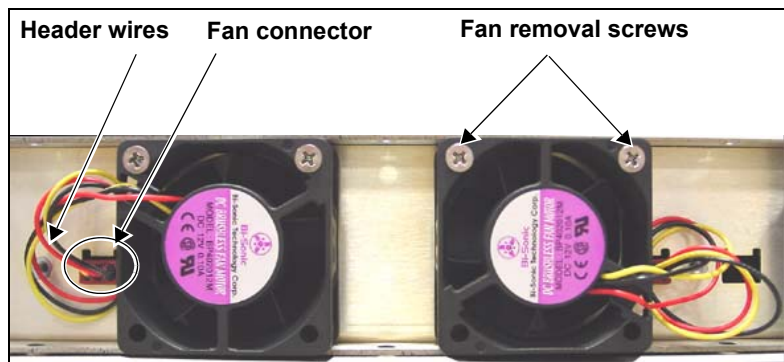
Figure C-55. Removing Header Wires from Fan Assembly Connector
