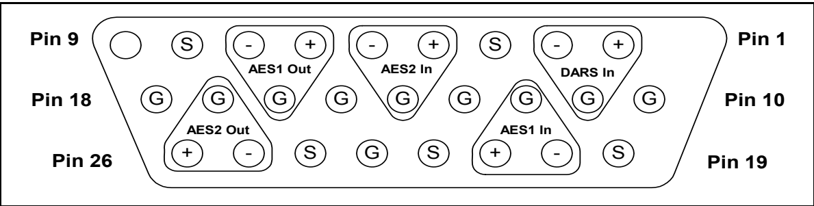
Figure A-14. X75OPTCAB-8-X Connector Pinout
