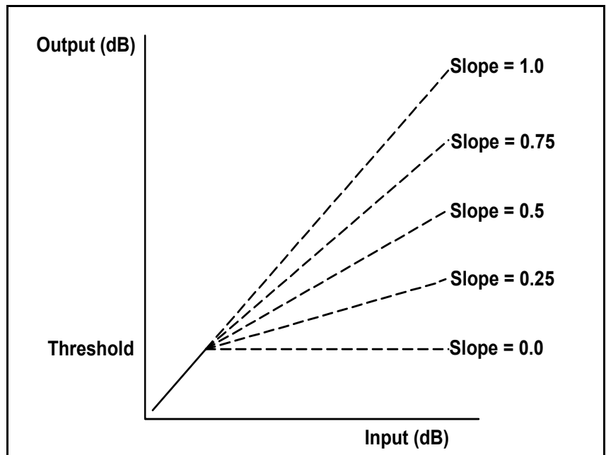
Figure C-32. Audio Limiter Transfer Function
