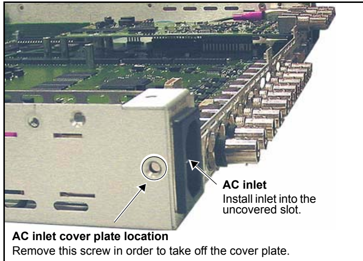
Figure C-50. Removing Cover Plate and Installing AC Inlet
