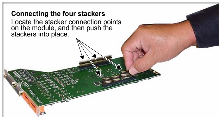
Figure C-4. Connecting Four Stackers to Module
