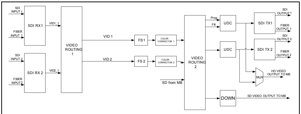
Figure 2-5. Keyer with I-Wings Side Panel Fill Mode
