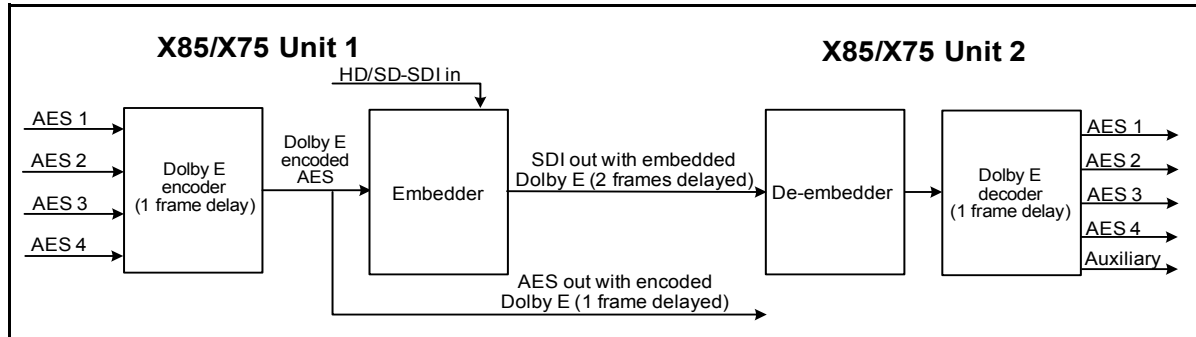
Figure 9-11. Audio Delay in Dolby E
