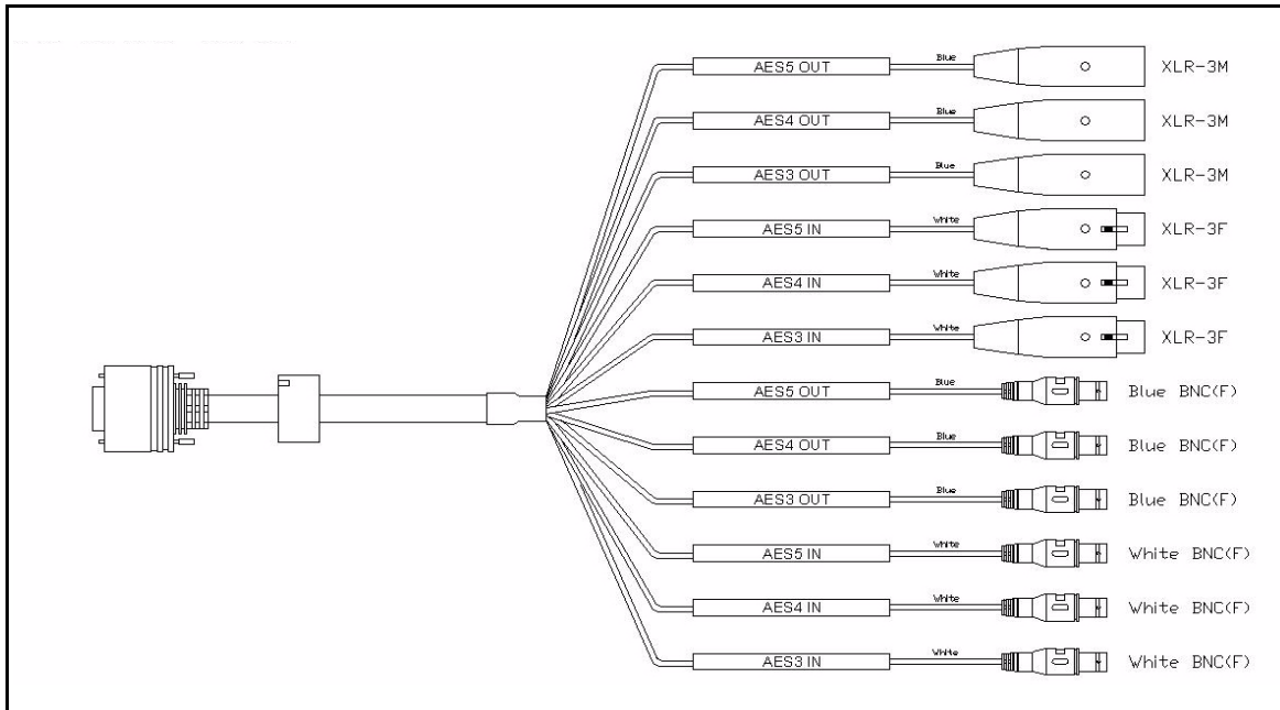
Figure A-11. CAB-X75HD-COMBO Cable Connectors
