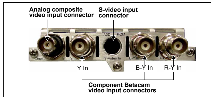
Figure 1-7. PQM-X75 Back Panel
