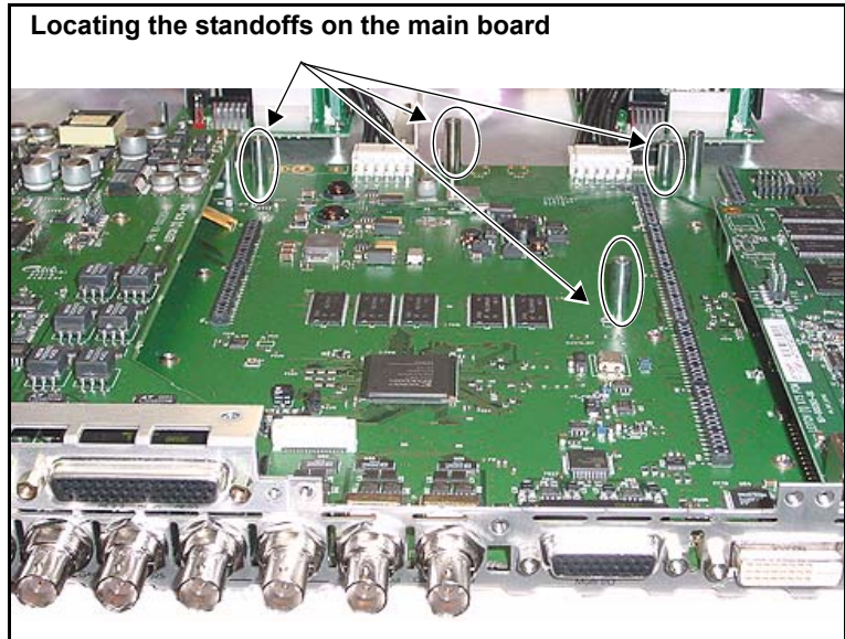
Figure C-11. Locating Main Board Standoffs
