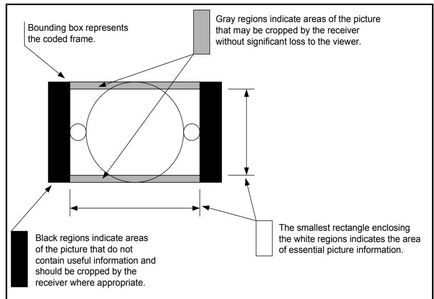
Figure 8-16. AFD Diagram Explanation
