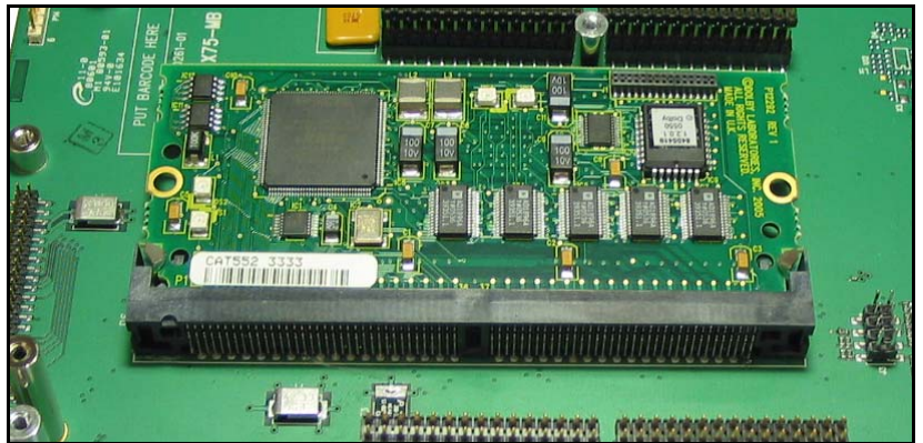
Figure C-40. Dolby Decoder Module Installed
