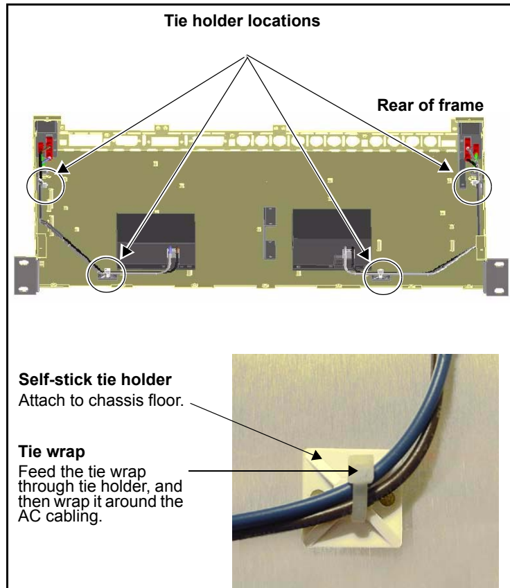
Figure C-49. Attaching Tie Wraps to AC Cabling
