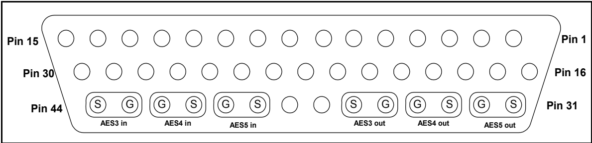
Figure A-8. CAB-X75HD-COAX Connector Pinout
