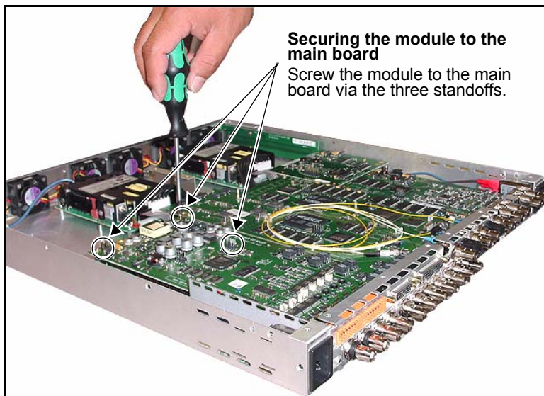
Figure C-8. Securing the Module to the Main Board
