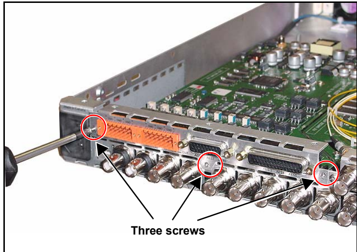
Figure C-35. Removing Audio Back Module Screws
