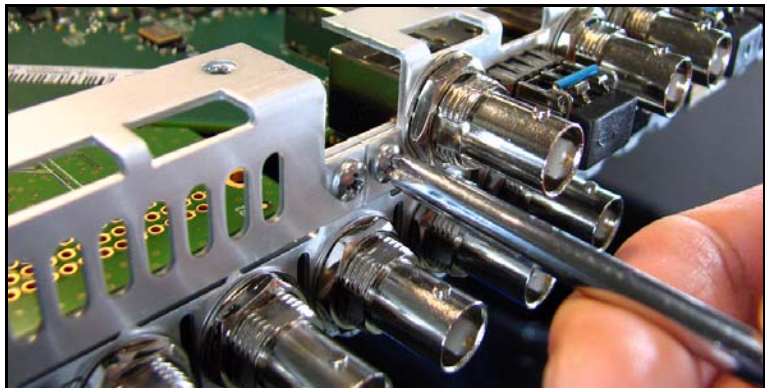
Figure C-21. Securing the Back Connector to the Frame
