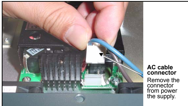
Figure C-44. Removing AC Cable from Power Supply
