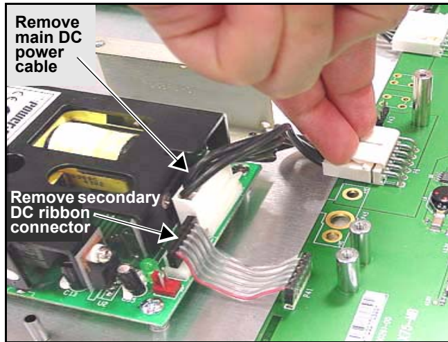
Figure C-43. Removing the DC and Ribbon Cables
