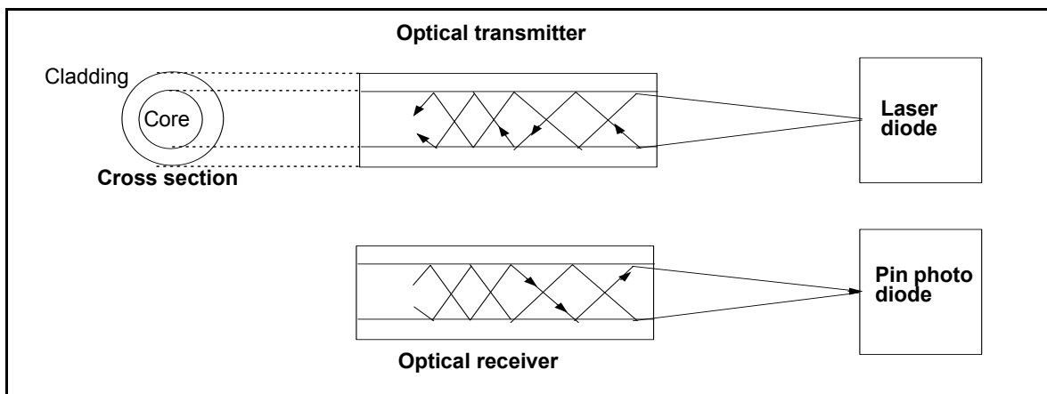
Figure C-1. Fiber Optic Transmitting and Receiving
