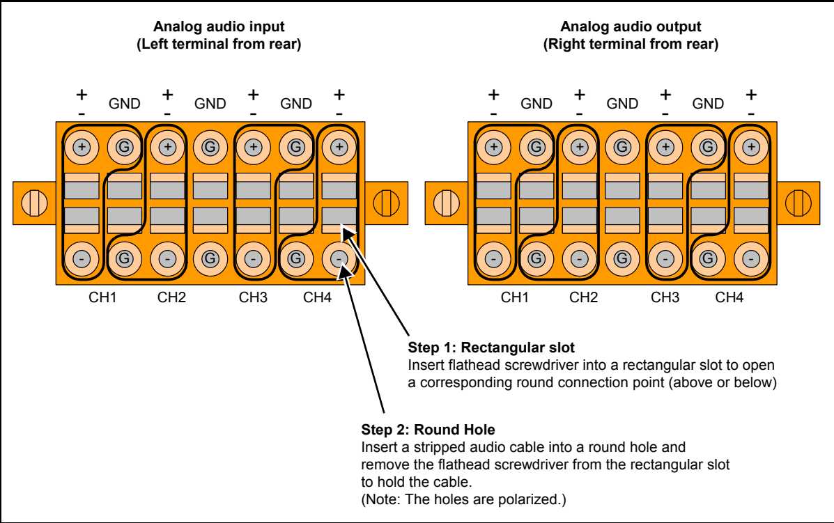
Figure A-1. Analog Audio Input and Output Terminal Blocks
