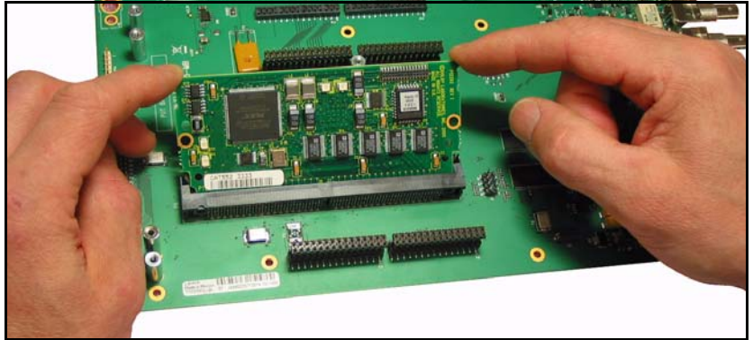
Figure C-39. Inserting Dolby Decoder Module into Socket
