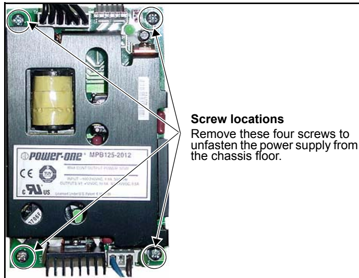
Figure C-45. Removing the Power Supply
