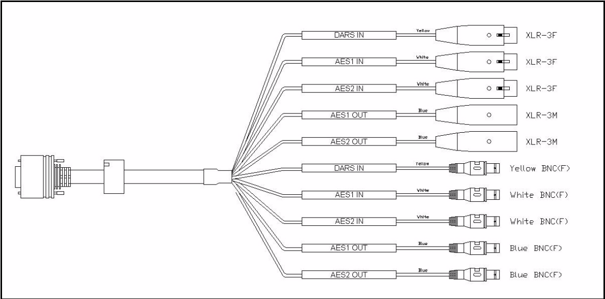
Figure A-9. X75OPTCAB-8-XC Cable Connectors
