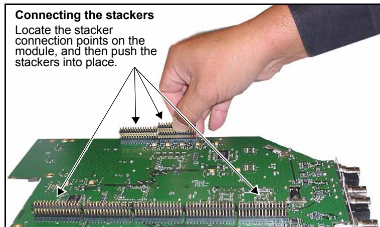
Figure C-10. Connecting Seven Stackers to Module
