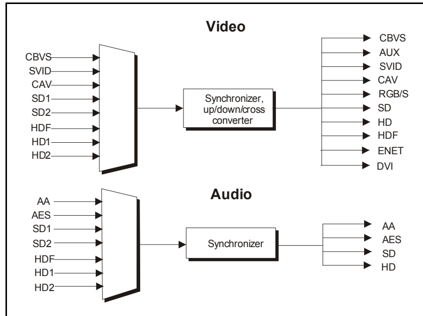
Figure 2-6. X75 M-Path Single-Source Video and Audio Processing
