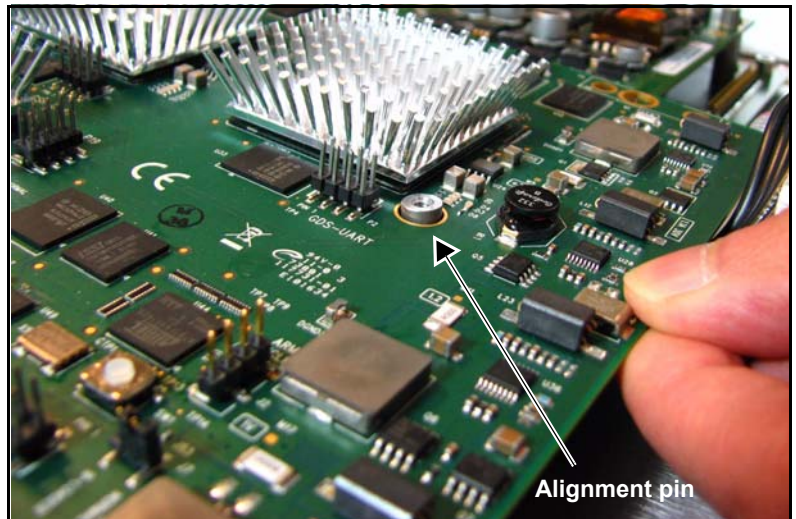
Figure C-18. Alignment Pin for the X85 Module
