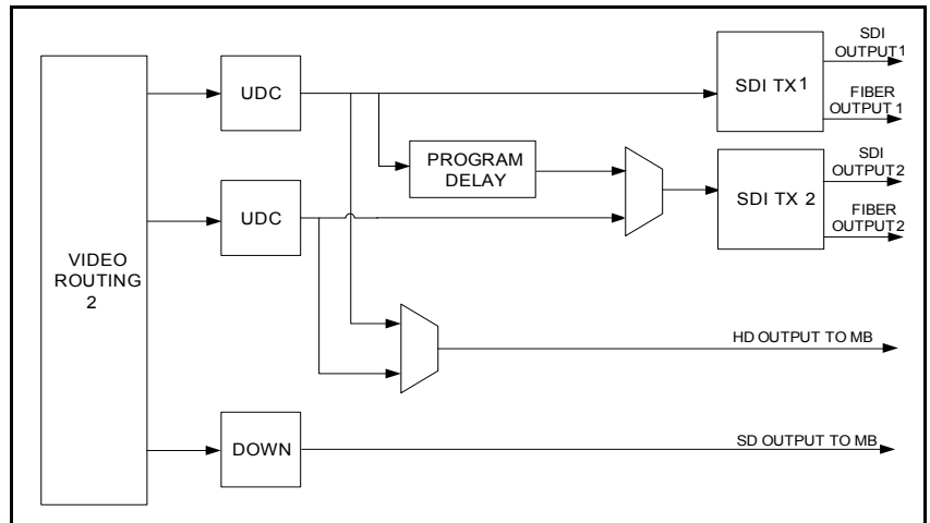
Figure 2-4. X85 Program Delay Mode
