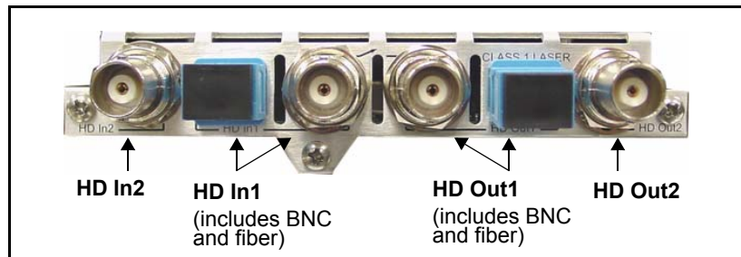
Figure 1-10. HD-X75 Back Panel
