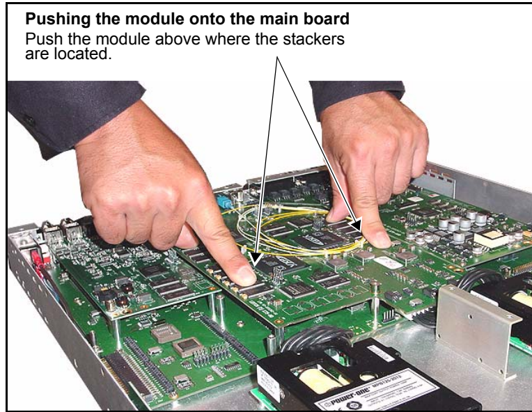
Figure C-13. Pushing the Module on to the Main Board
