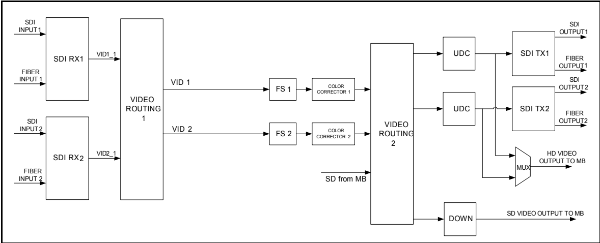
Figure 2-2. X85 M-Path Mode
