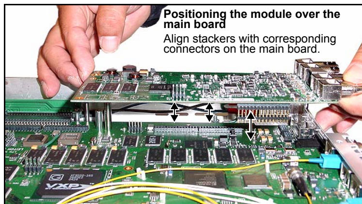
Figure C-26. Positioning Module over Standoffs
