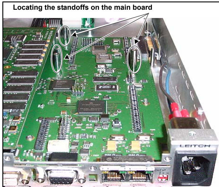
Figure C-25. Locating Main Board Standoffs
