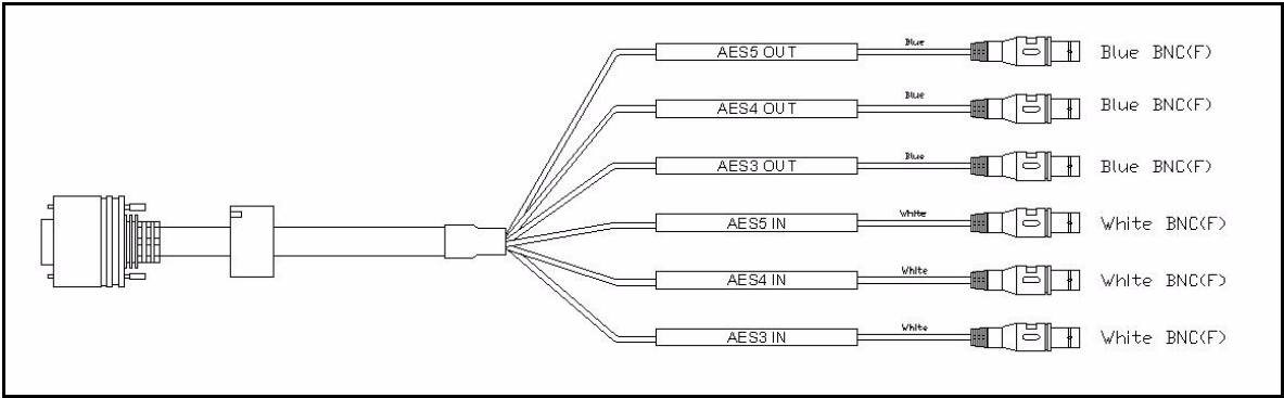
Figure A-7. CAB-X75HD-COAX Cable Connectors
