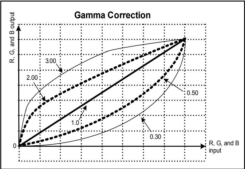
Figure 8-27. Example of Gamma Corrections to R, G, and B
