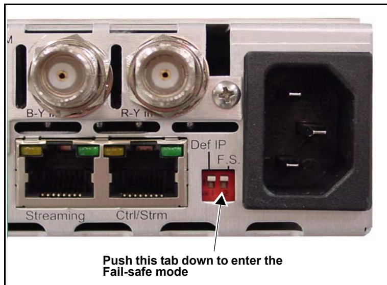
Figure B-12. Location of the F.S. (Fail-safe) DIP Switch
