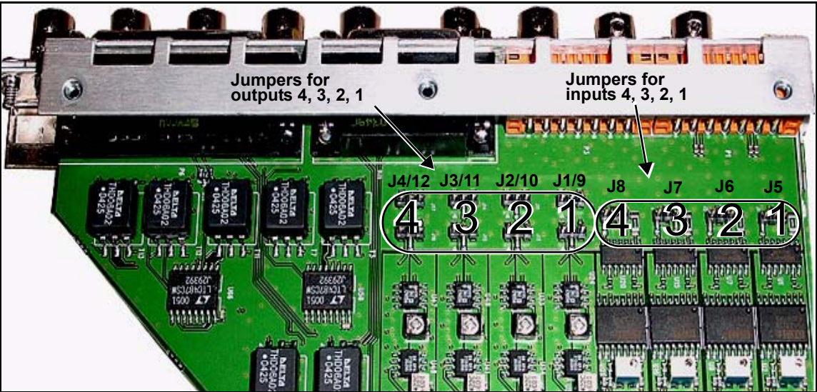
Figure 1-3. Jumper Locations for X75OPT-AS-16 and X75OPT-AS-8 Modules
