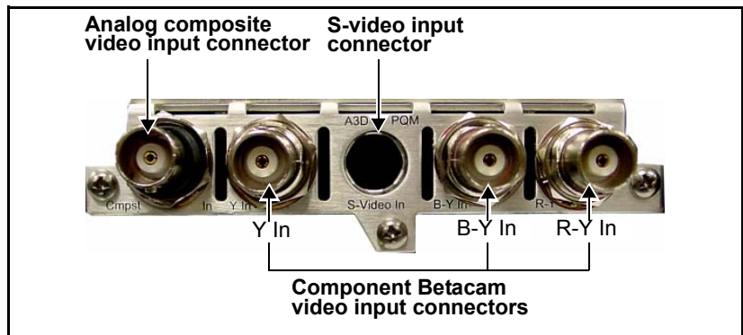
Figure 1-6. X75OPT-A3D Module Back Panel
