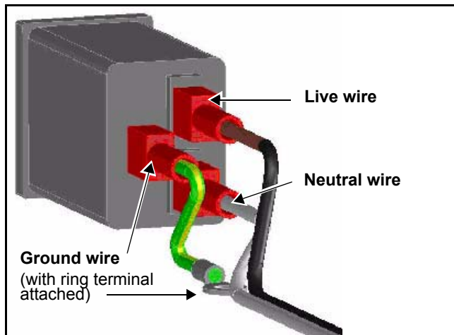
Figure C-51. Connecting AC Cables to Inlet
