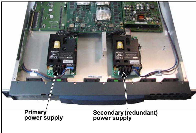
Figure C-42. Location of Connected Power Supply
