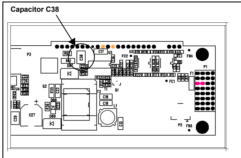
Figure B-3. Location of Failed Capacitor Behind VFD
