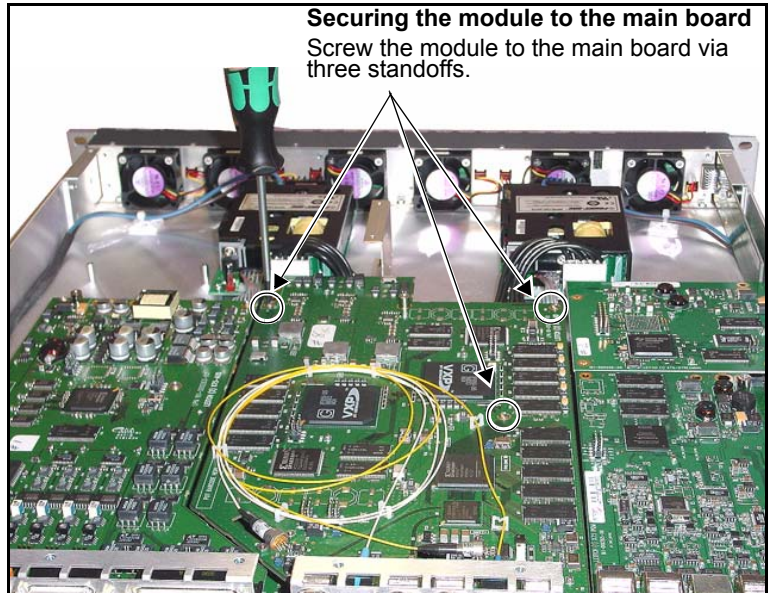
Figure C-14. Securing the Module to the Main Board
