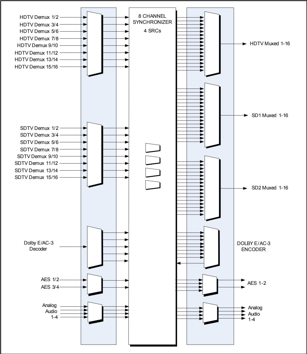
Figure 2-8. Eight-Channel Audio Functional Block Diagram
