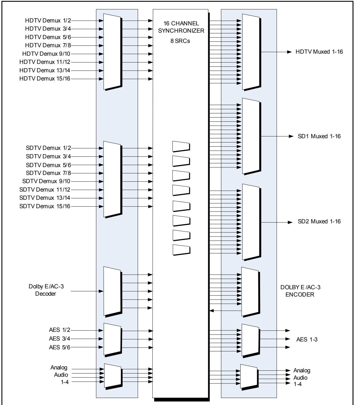
Figure 2-9. 16-Channel Audio Functional Block Diagram
