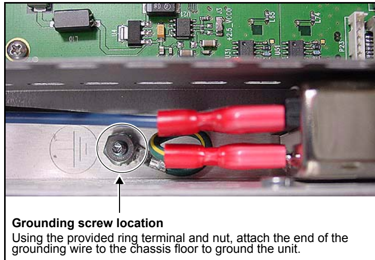
Figure C-52. Grounding AC Inlet
