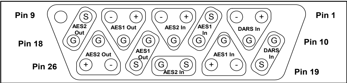
Figure A-10. X75OPTCAB-8-XC Connector Pinout
