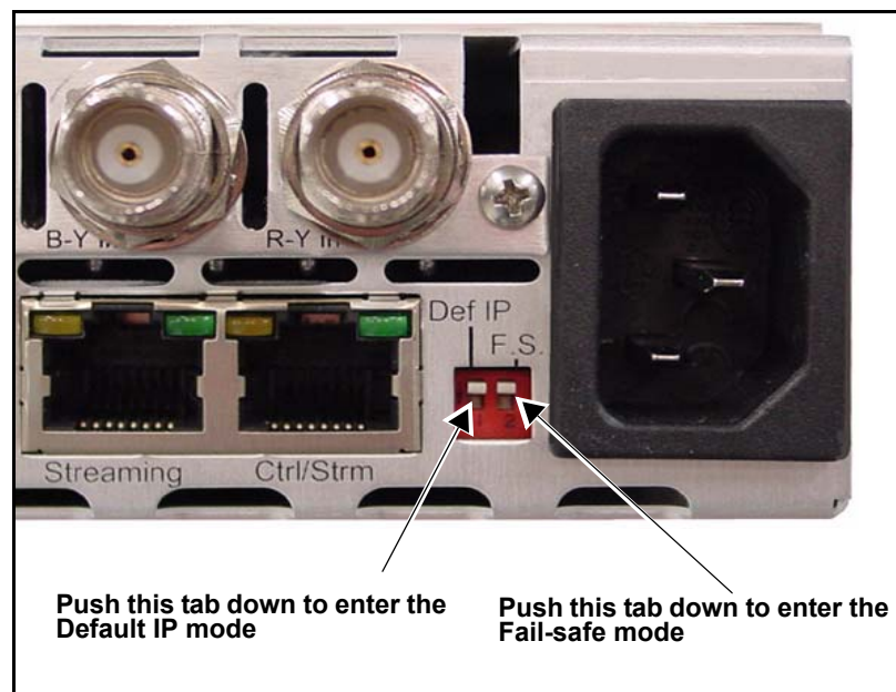
Figure B-11. Location of Def IP and FS DIP Switches
