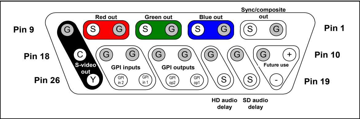
Figure A-3. X75OPTCAB-MULTI I/O Connector Pinout
