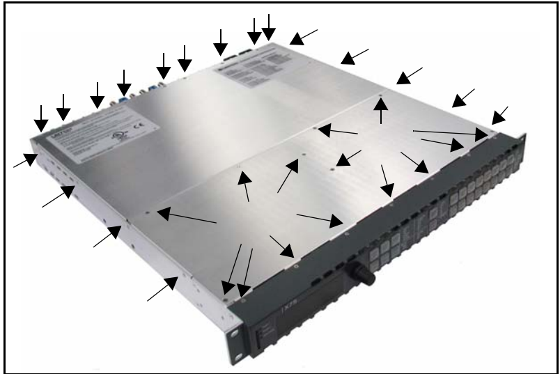
Figure C-34. Chassis Cover Screws
