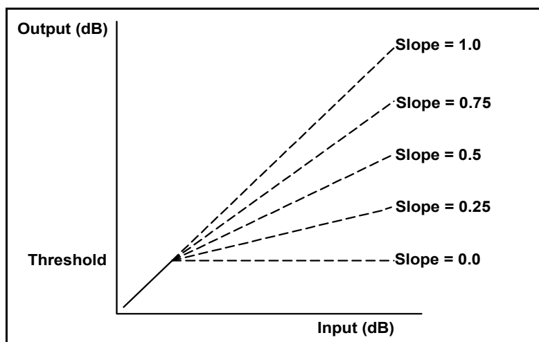
Figure 1-5. Audio Limiter Transfer Function
