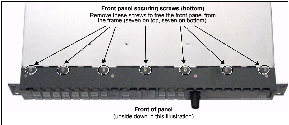
Figure C-53. Freeing the Front Panel from the Frame
