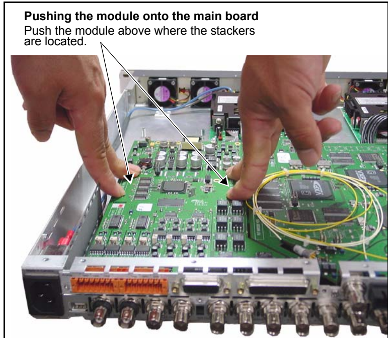
Figure C-7. Pushing the Module on to the Main Board
