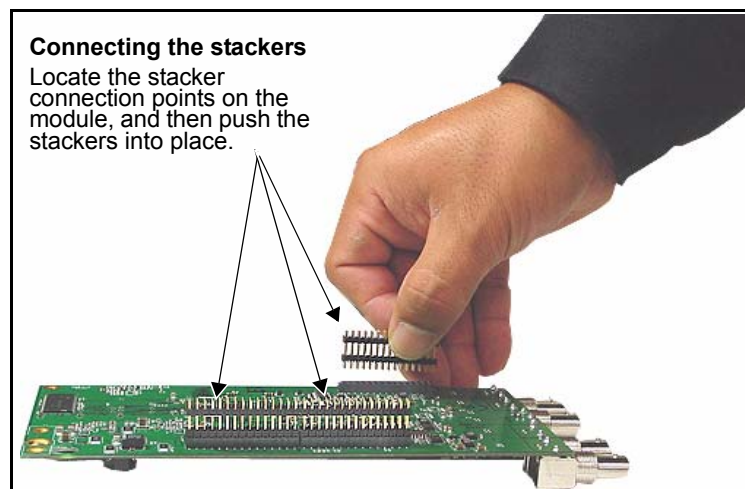
Figure C-24. Connecting Three Stackers to Module
