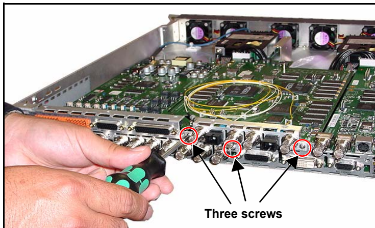
Figure C-36. Removing HDTV Back Module Screws (X75OPT-HDUPG HD Module Shown)
