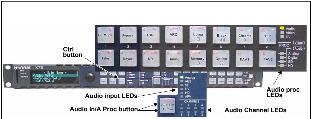
Figure 9-2. Location of Audio LEDs (X75 Shown)
