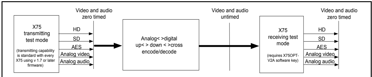
Figure 8-2. X75OPT-V2A Video/Audio Timing Feature
