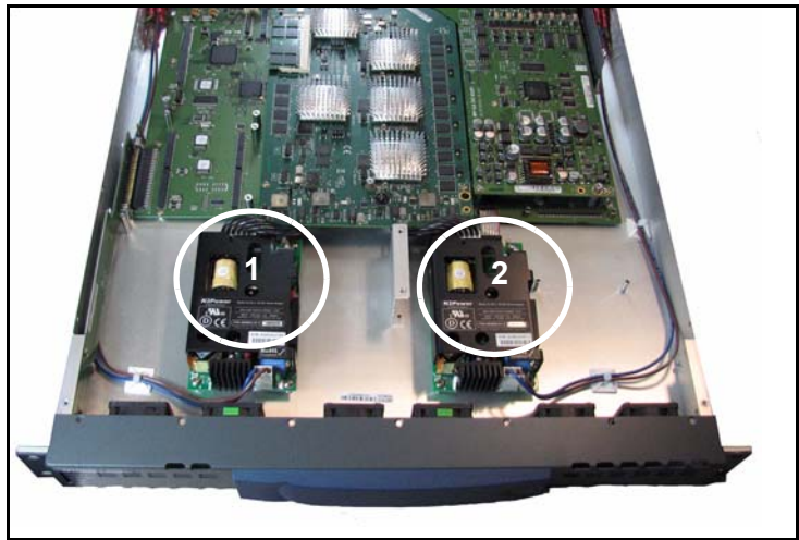
Figure C-46. Where to Install a Redundant Power Supply
