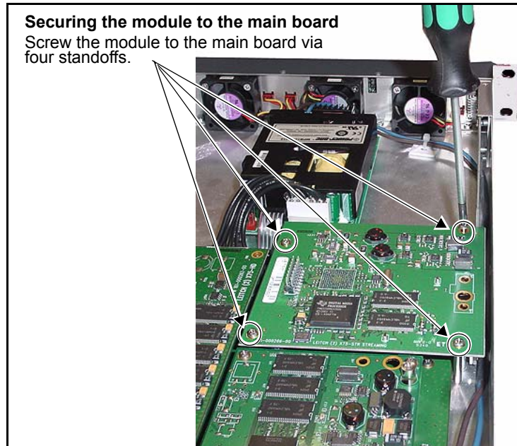
Figure C-30. Securing the Module to the Main Board
