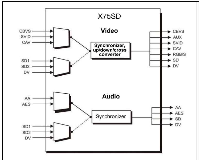
Figure 2-13. X75 Simulcast Switcher Application
