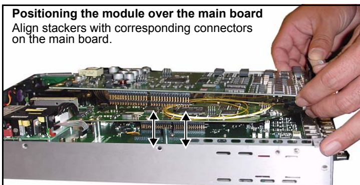
Figure C-6. Positioning Module over Standoffs
