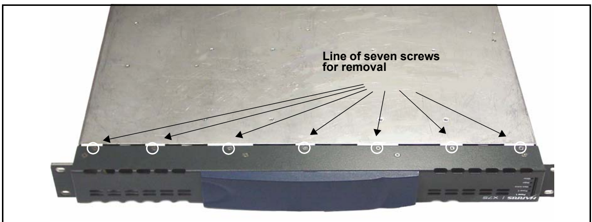
Figure C-3. Removing the Bottom Front Panel Screws
