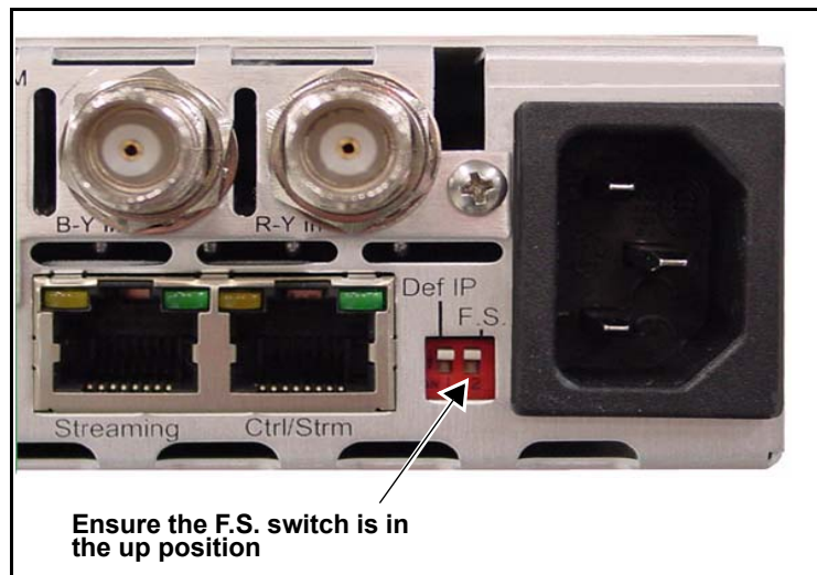
Figure B-2. Fail-safe Switch
