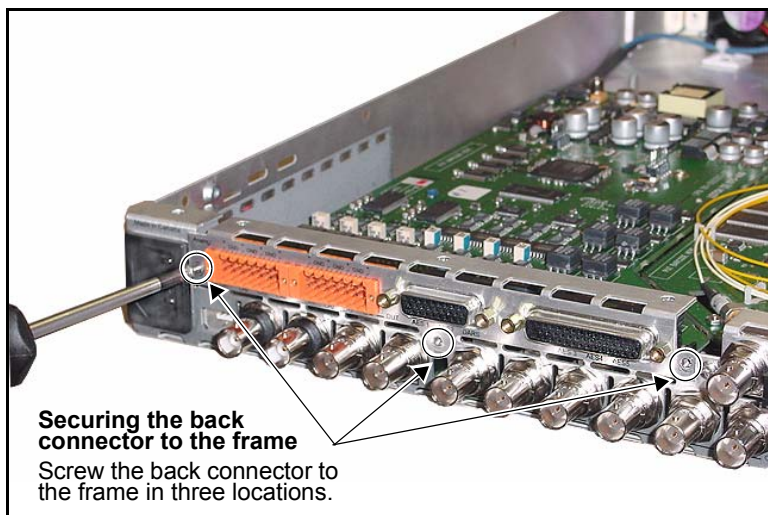
Figure C-9. Securing the Back Connector to the Frame
