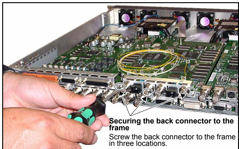
Figure C-15. Securing the Back Connector to the Frame
