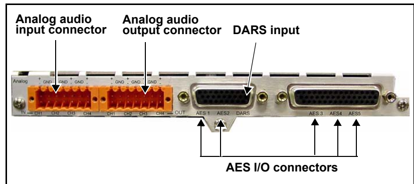
Figure 1-1. X75OPT-AS-16/X75OPT-AS-8 Back Panel
