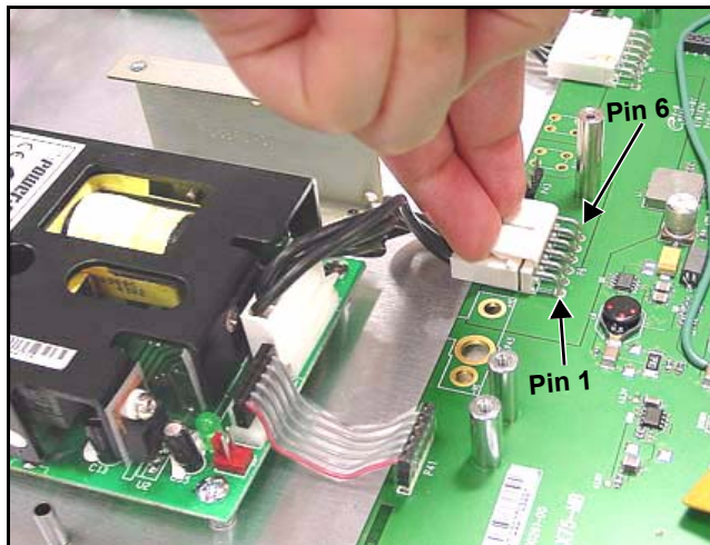
Figure B-4. Location of Power Supplies DC Cables
