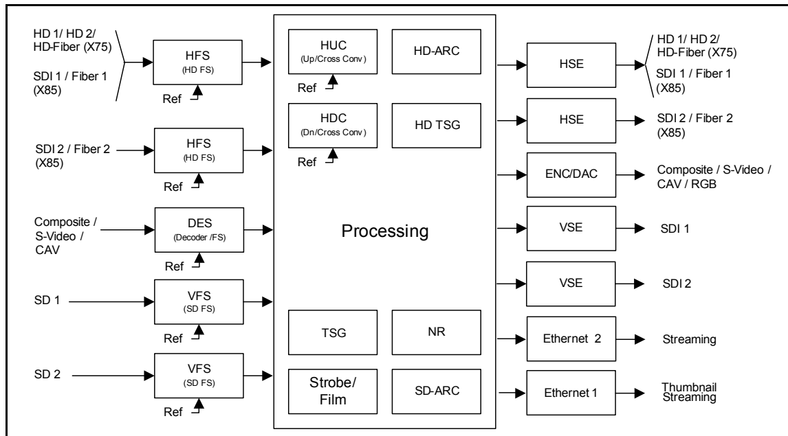
Figure 2-1. Video Functional Block Diagram
