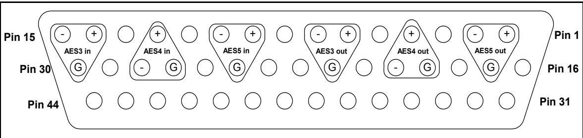
Figure A-16. X75OPTCAB-XLR Connector Pinout
