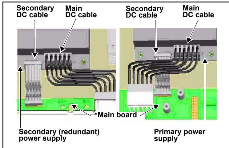
Figure C-47. Connecting DC and Ribbon Cables
