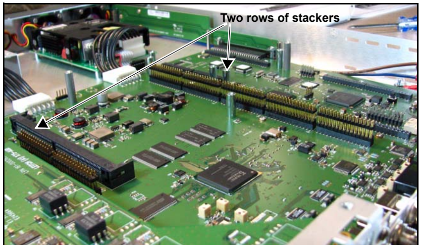
Figure C-16. Stackers on the Main Board
