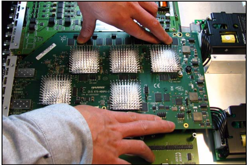
Figure C-20. Pushing the Module Onto the Main Board
