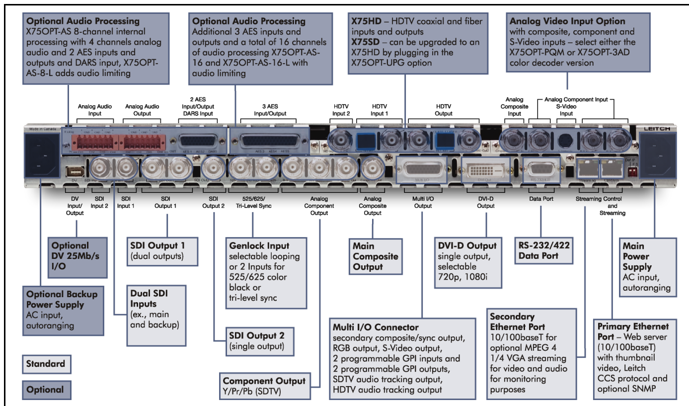
Figure 1. X75 Back Panel
