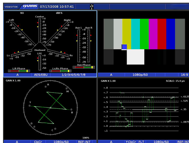
Figure 3-72. 3Gbs WFM/VEC Mode Display
