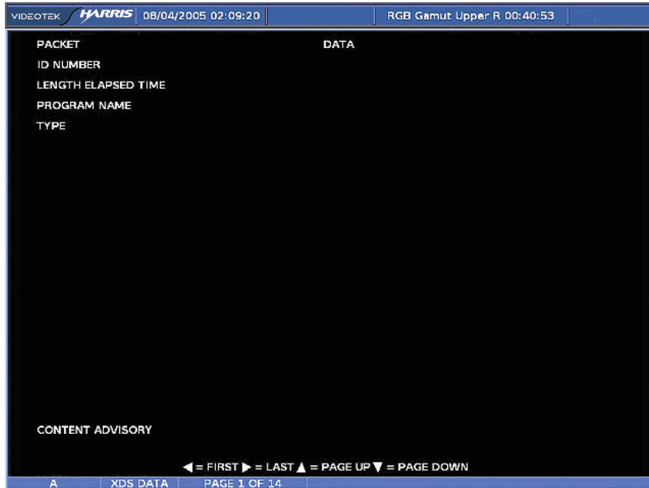
Figure 3-60. XDS Pane
