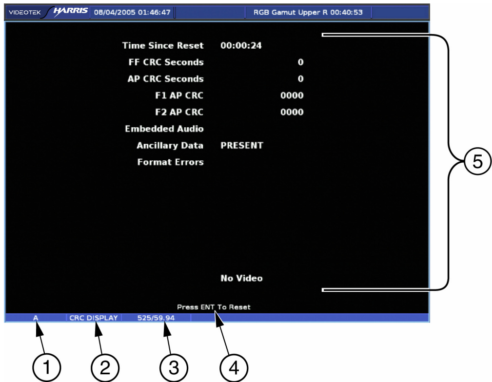
Figure 3-61. CRC Display Diagram
