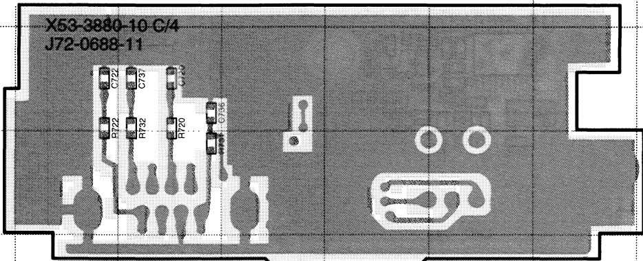
CONTROL UNIT (X53-3880-10) (C/4) Foil Side View
