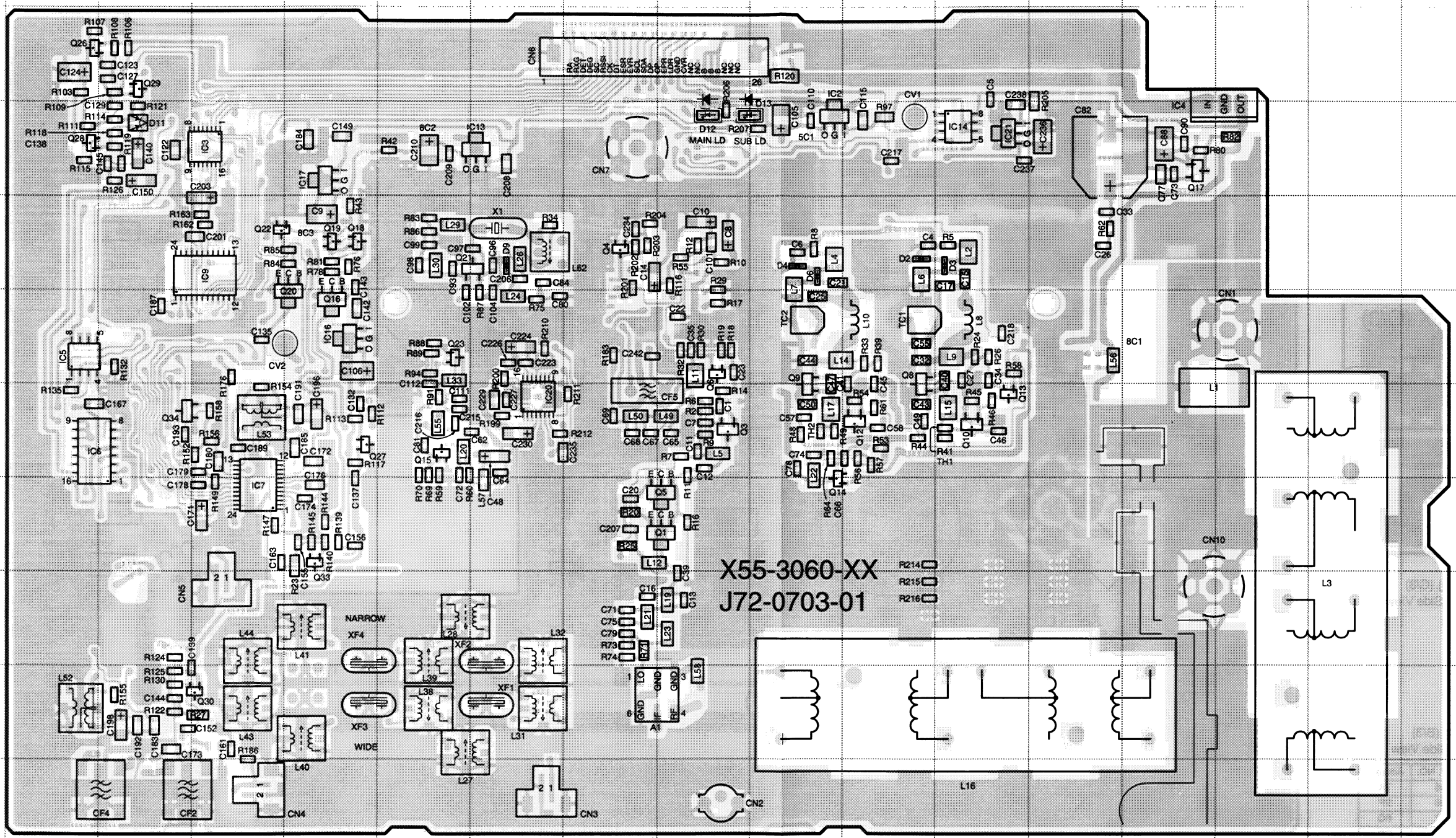
RX UNIT (X55-3060-XX) Component Side View
