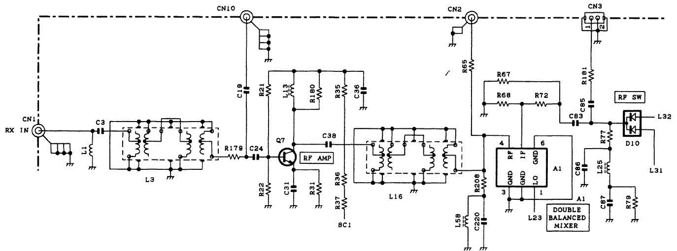
Fig.15 Front-end circuit
