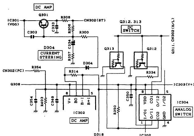
Fig.11 APC circuit
