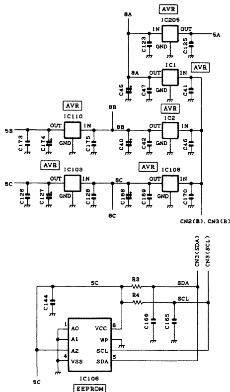
Fig.7 Other circuits
