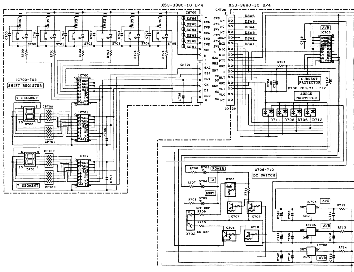
Fig.27 Display circuit
