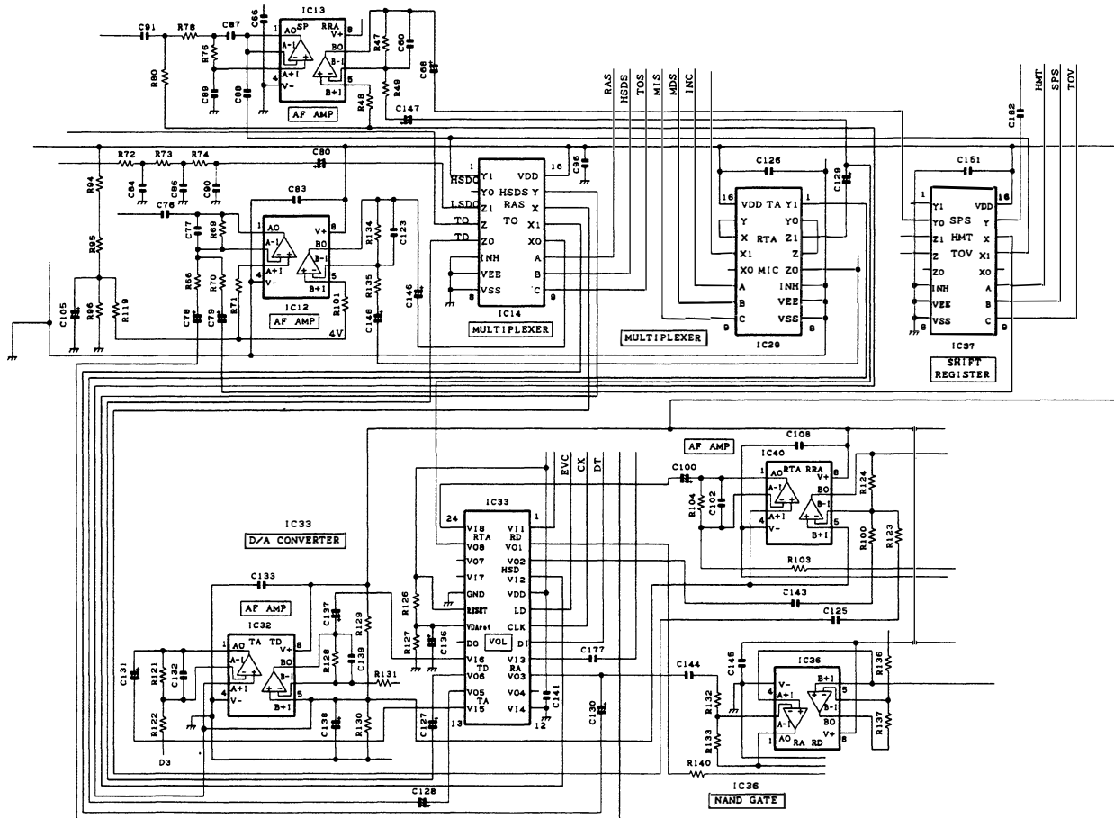
Fig.28 Baseband circuit
