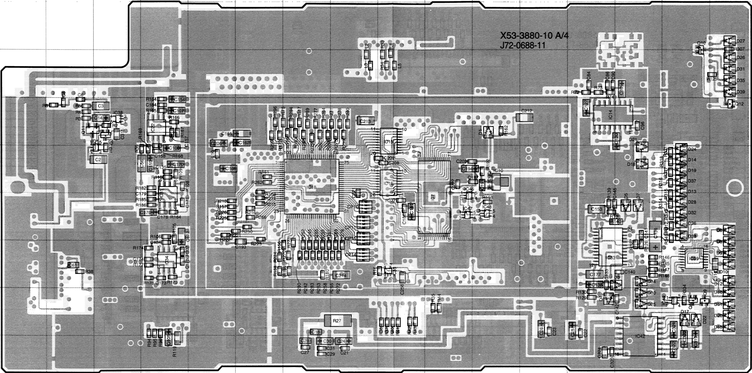
CONTROL UNIT (X53-3880-10) (A/4) Foil Side View
