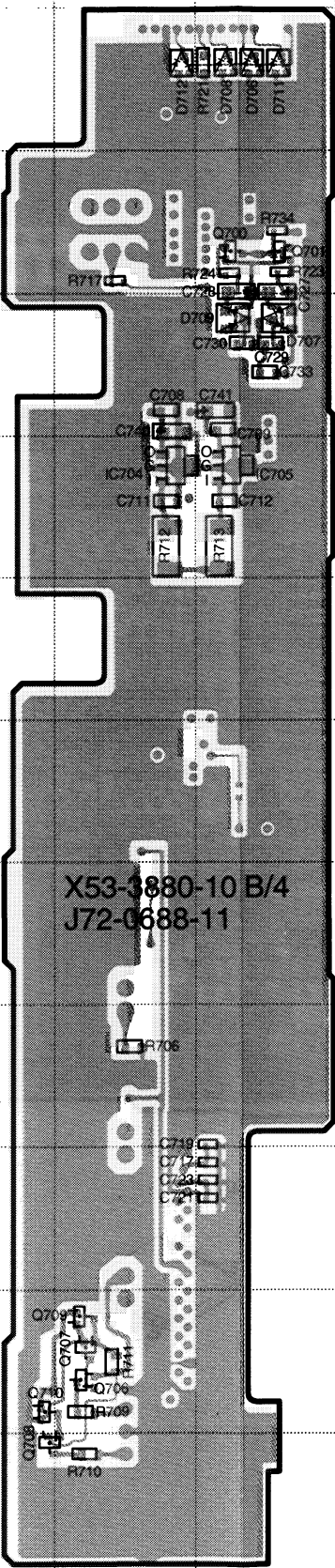
CONTROL UNIT (X53-3880-10) (B/4) Foil Side View
