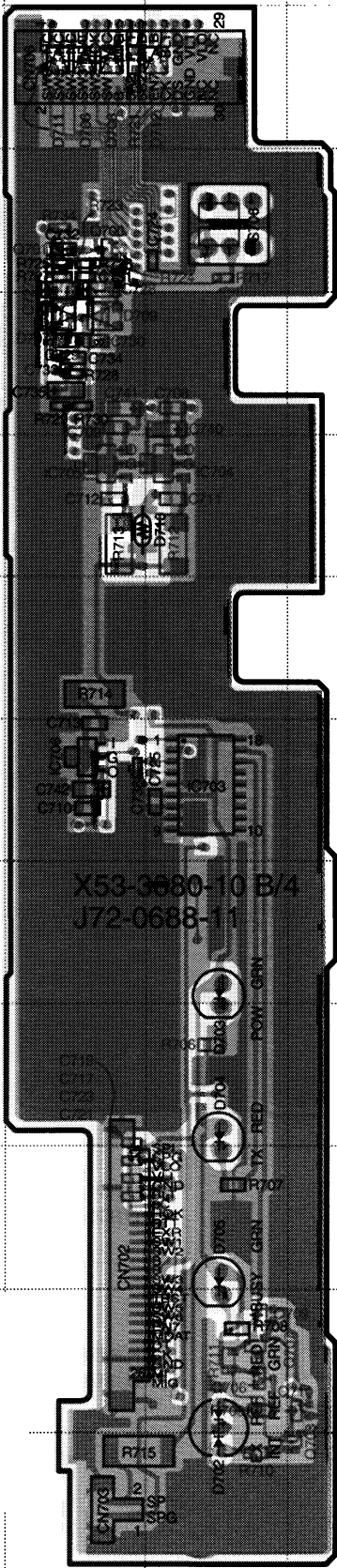
CONTROL UNIT (X53-3880-10) (B/4) Component Side + Foil Side View
