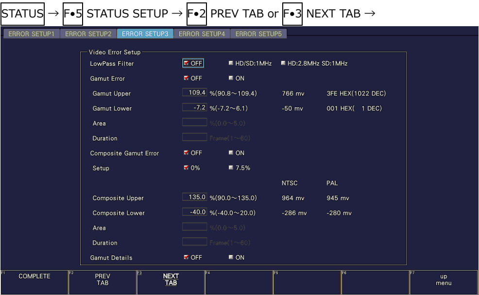
Figure 16-4 ERROR SETUP3 tab
