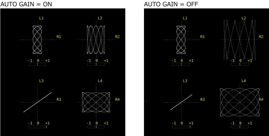
Figure 15-12 Setting the Lissajous curve gain
