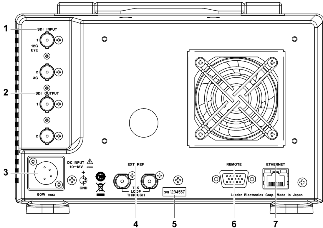
Figure 4-4 LV5300 rear panel
