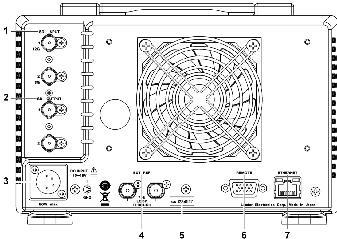
Figure 4-5 LV5350 rear panel
