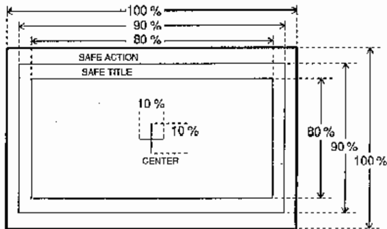
Figure 8.4 HD-SDI Marker Display (4:3 OFF)
