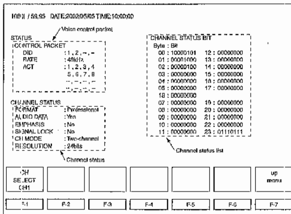
Figure 11.11 Detailed status display of embedded audio
