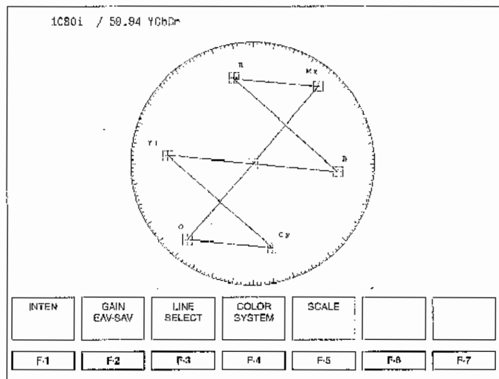
Figure 7.2 Vectorscope display and vectorscope display menu
