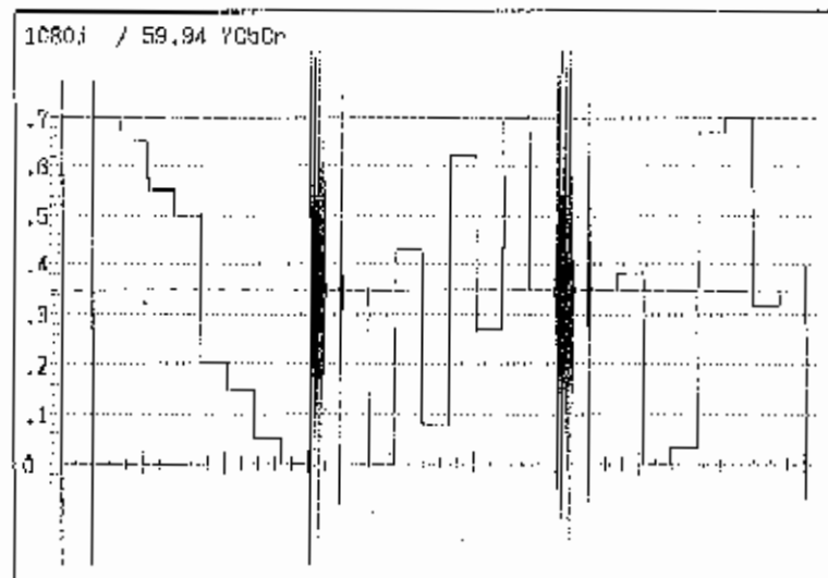
Figure 6.22 Waveform Display during the Blanking Period
