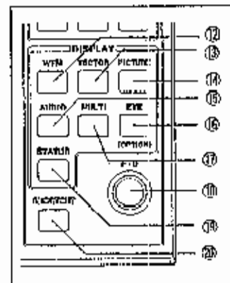
Figure 9.1 Area around the AUDIO key ⑮
