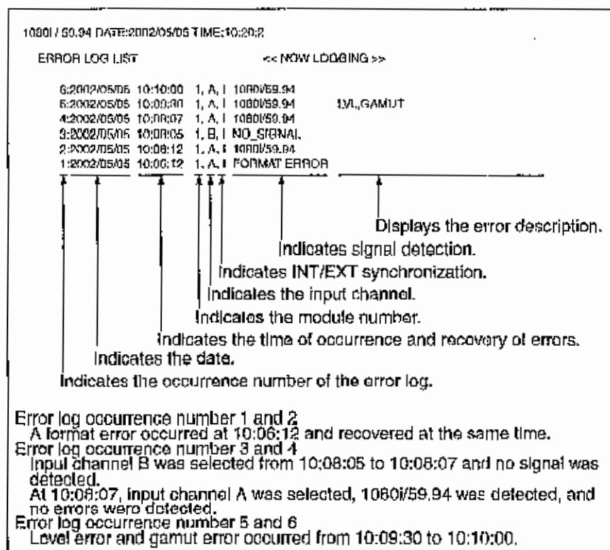
Figure 11.4 Error Log Display
