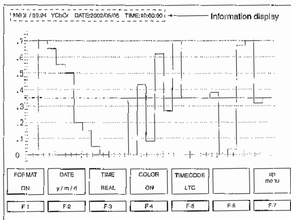
Figure 5.10 Information Display
