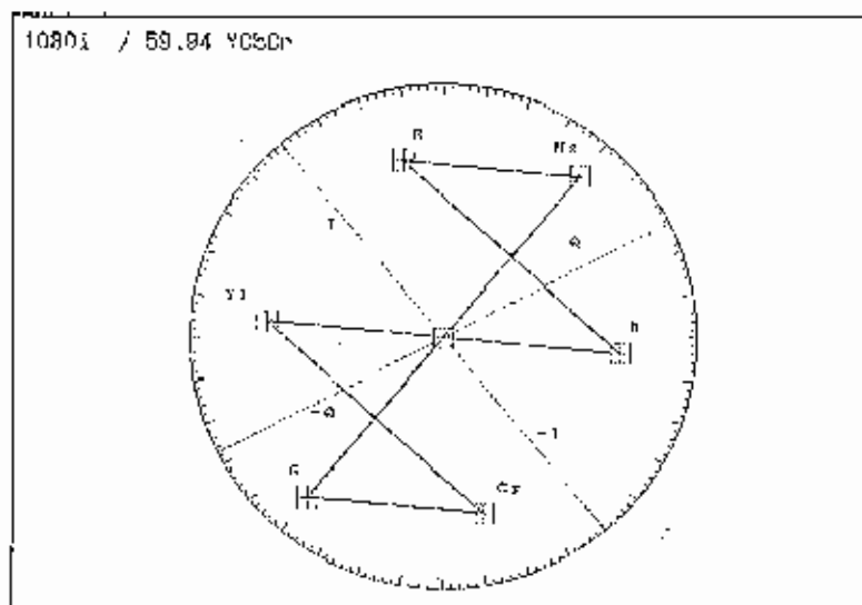
Figure 7.9 IQ axis on the vectorscope display
