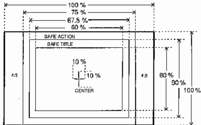
Figure 8.5 HD-SDI Marker Display (4:3 ON)
