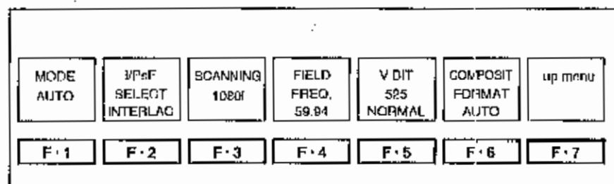
Figure 5.7 Video signal format setup menu
