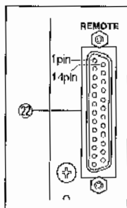
Figure 5.12 REMOTE Connector ②
