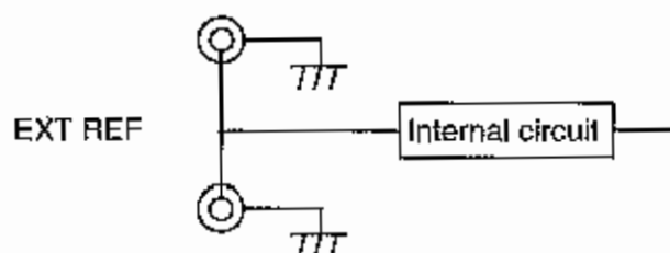
Figure 3.3 Loop-through input
