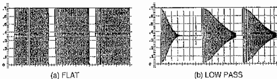
Figure 6.8 Low-pass Filter Waveform
