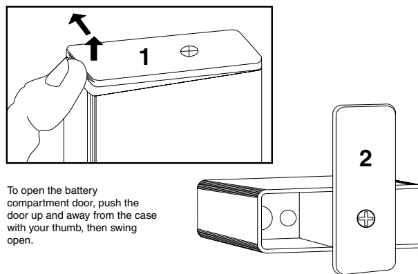
Figure 5 - Battery Replacement
