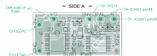
— SUB1 CIRCUIT BOARD —
